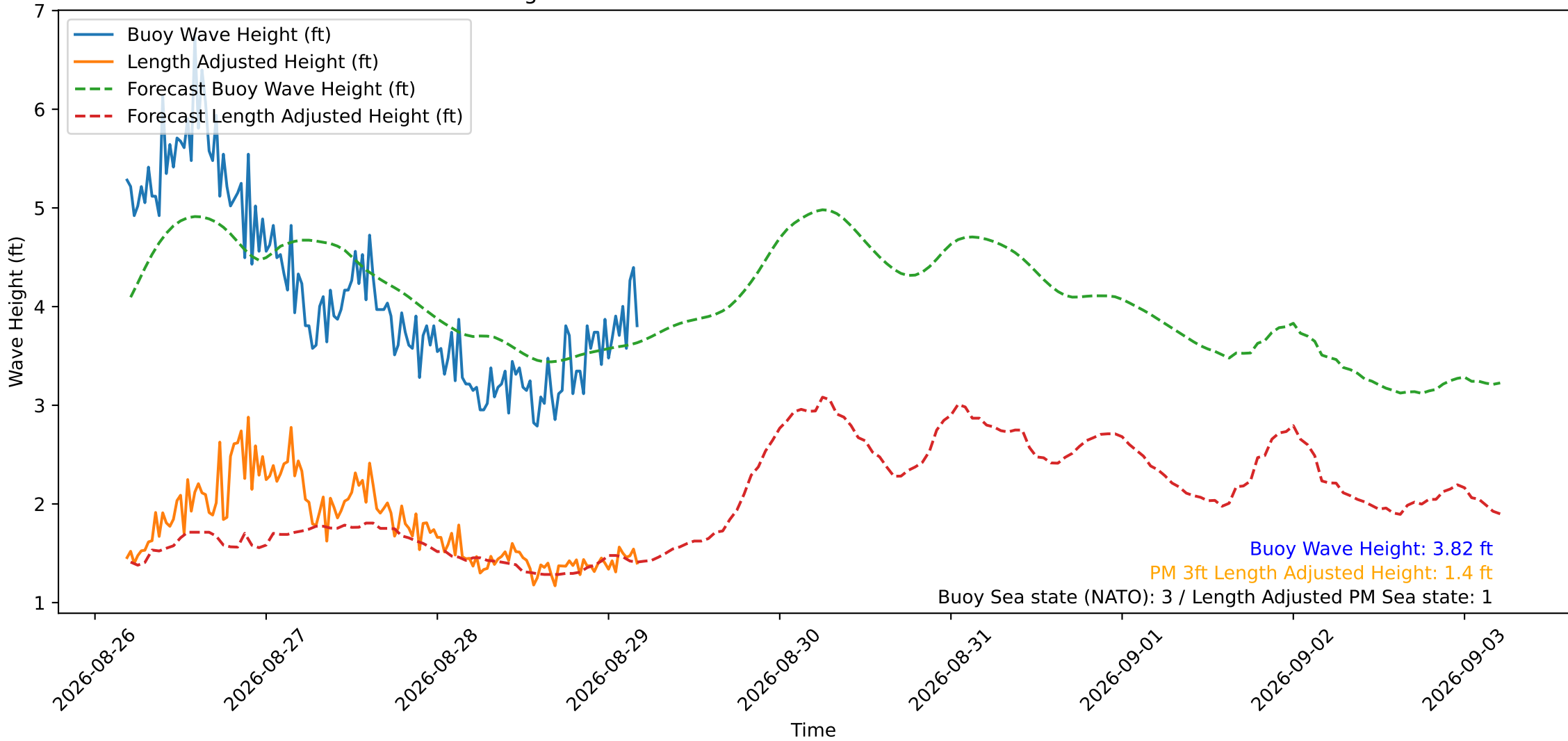
Wave Heights over Time for Oceanside Harbor at 2026-08-29 04:30:30
