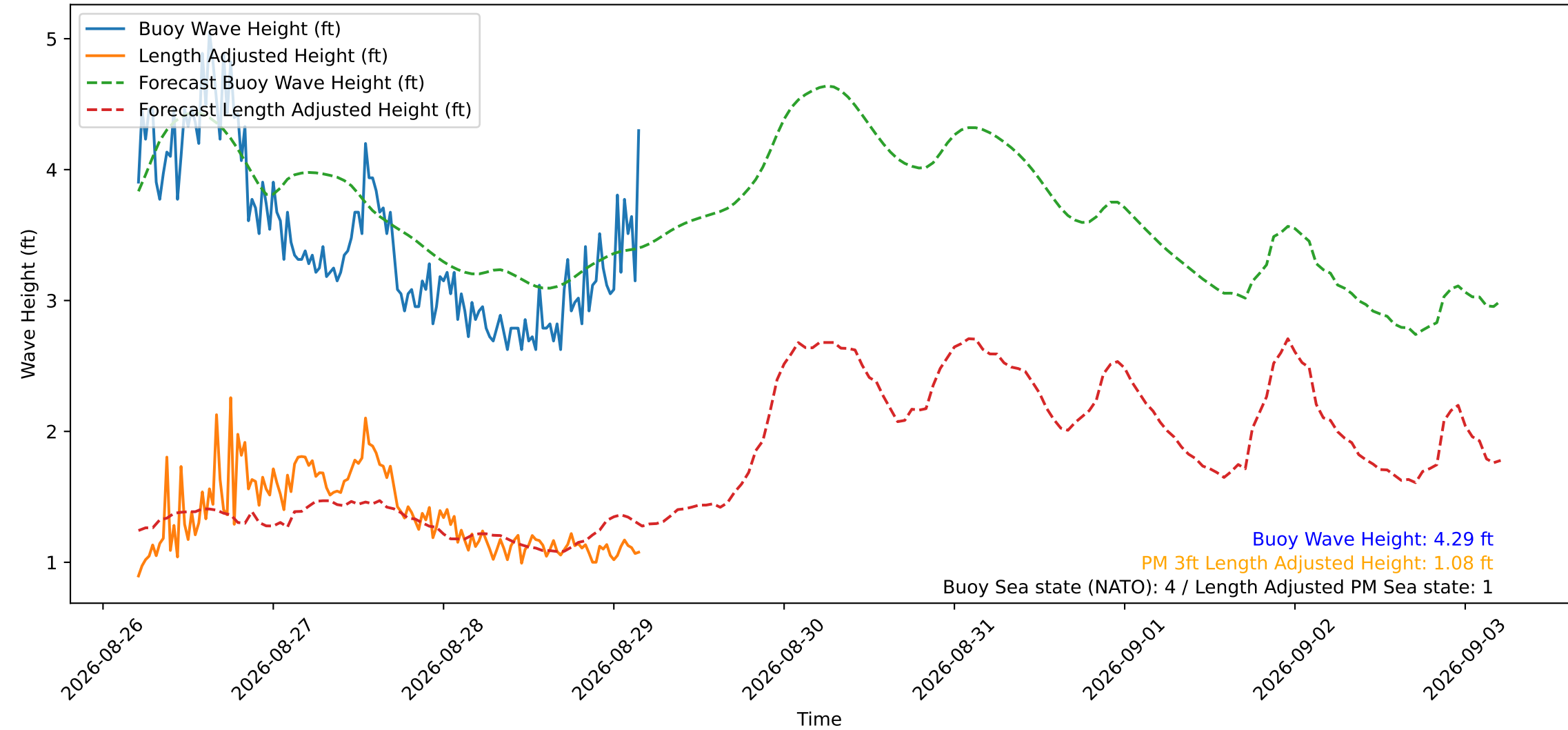
Wave Heights over Time for Red Beach at 2026-08-29 04:30:50
