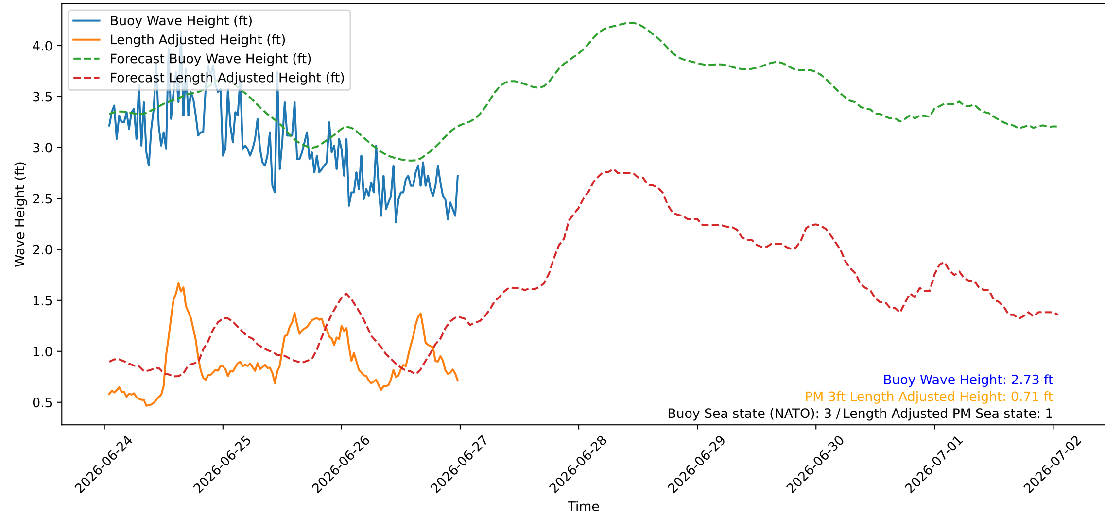
Wave Heights over Time for Red Beach at 2026-06-27 00:30:45
