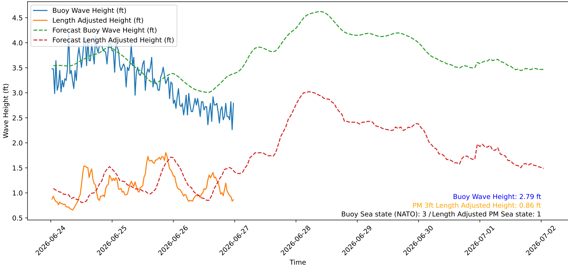
Wave Heights over Time for Green Beach at 2026-06-27 00:31:07
