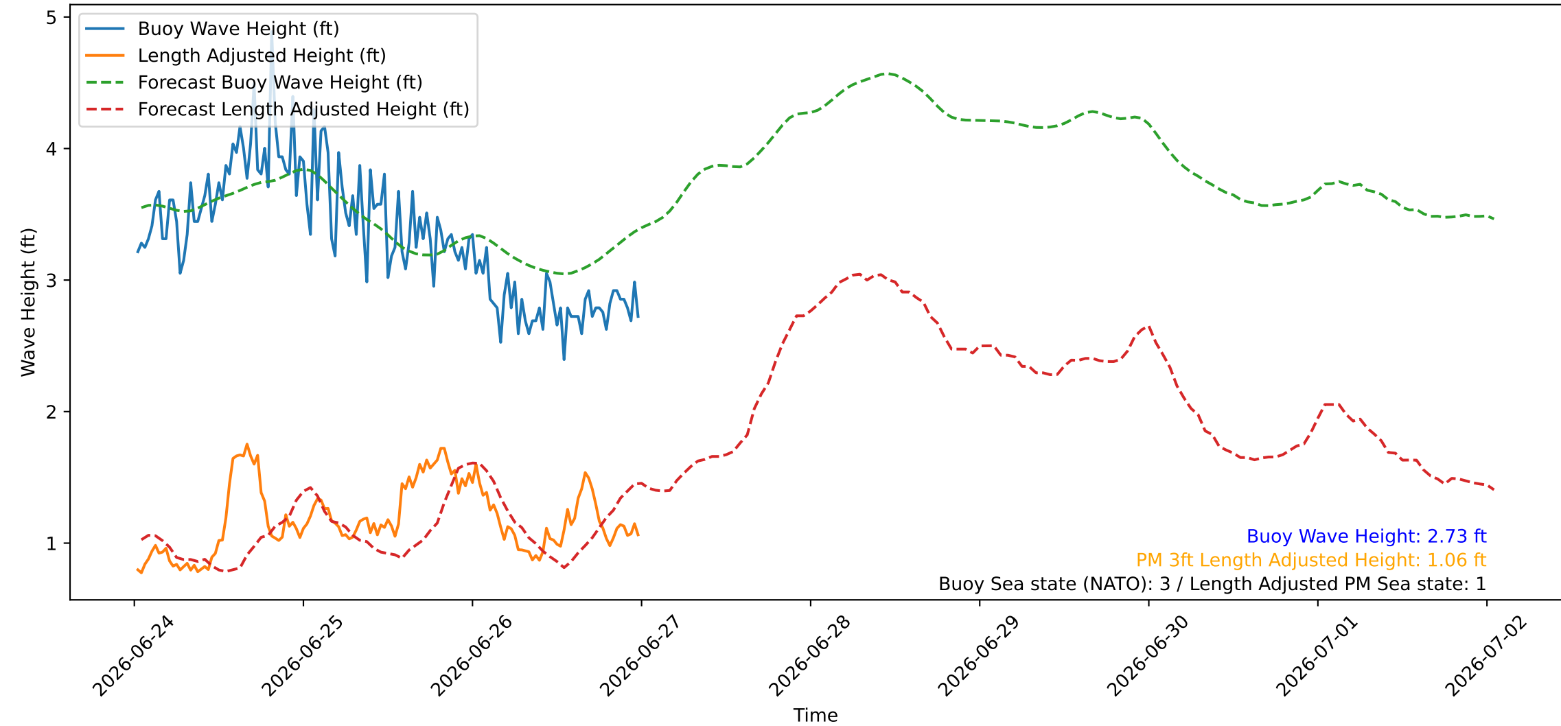
Wave Heights over Time for Oceanside Harbor at 2026-06-27 00:30:26
