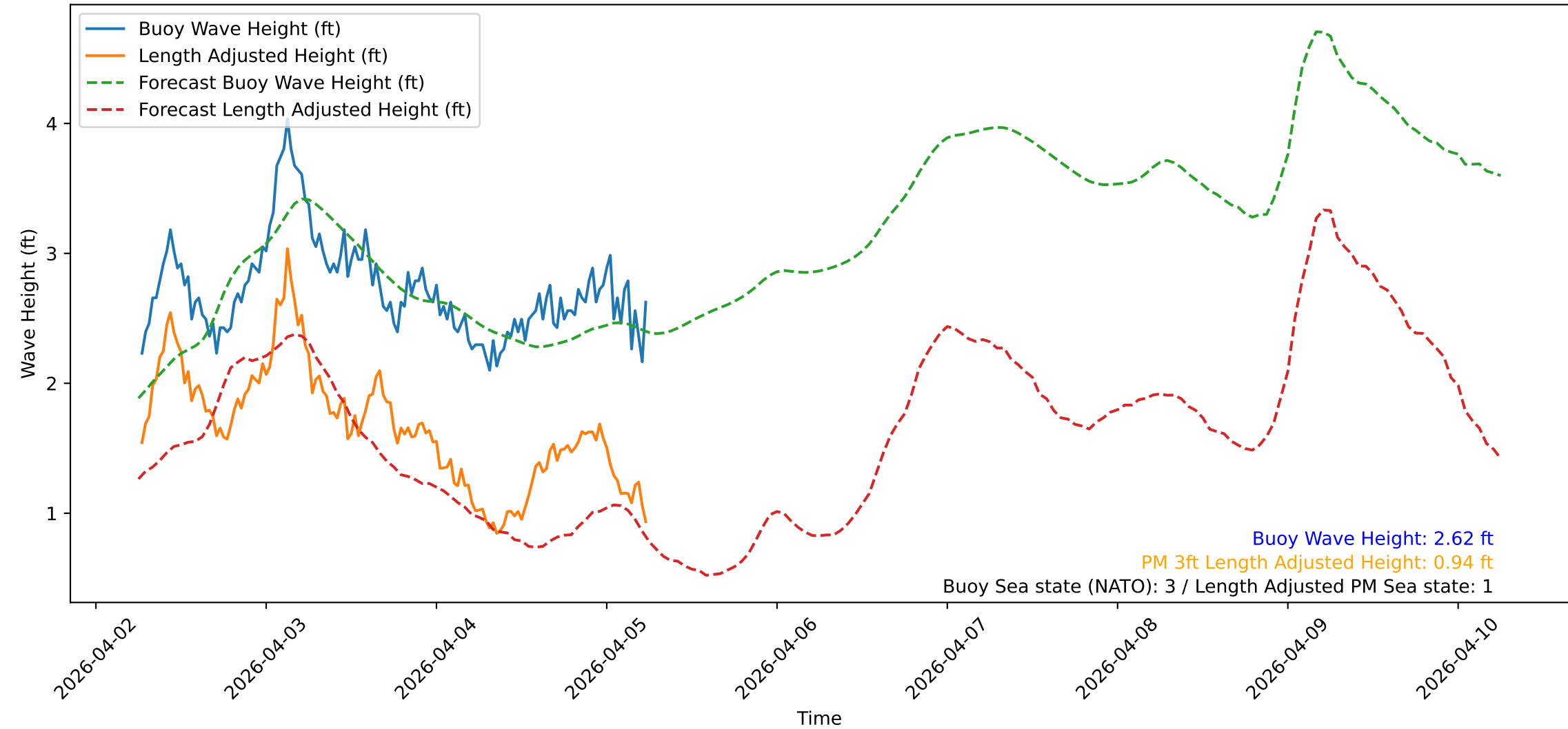
Wave Heights over Time for Oceanside Harbor at 2026-04-05 06:20:31
