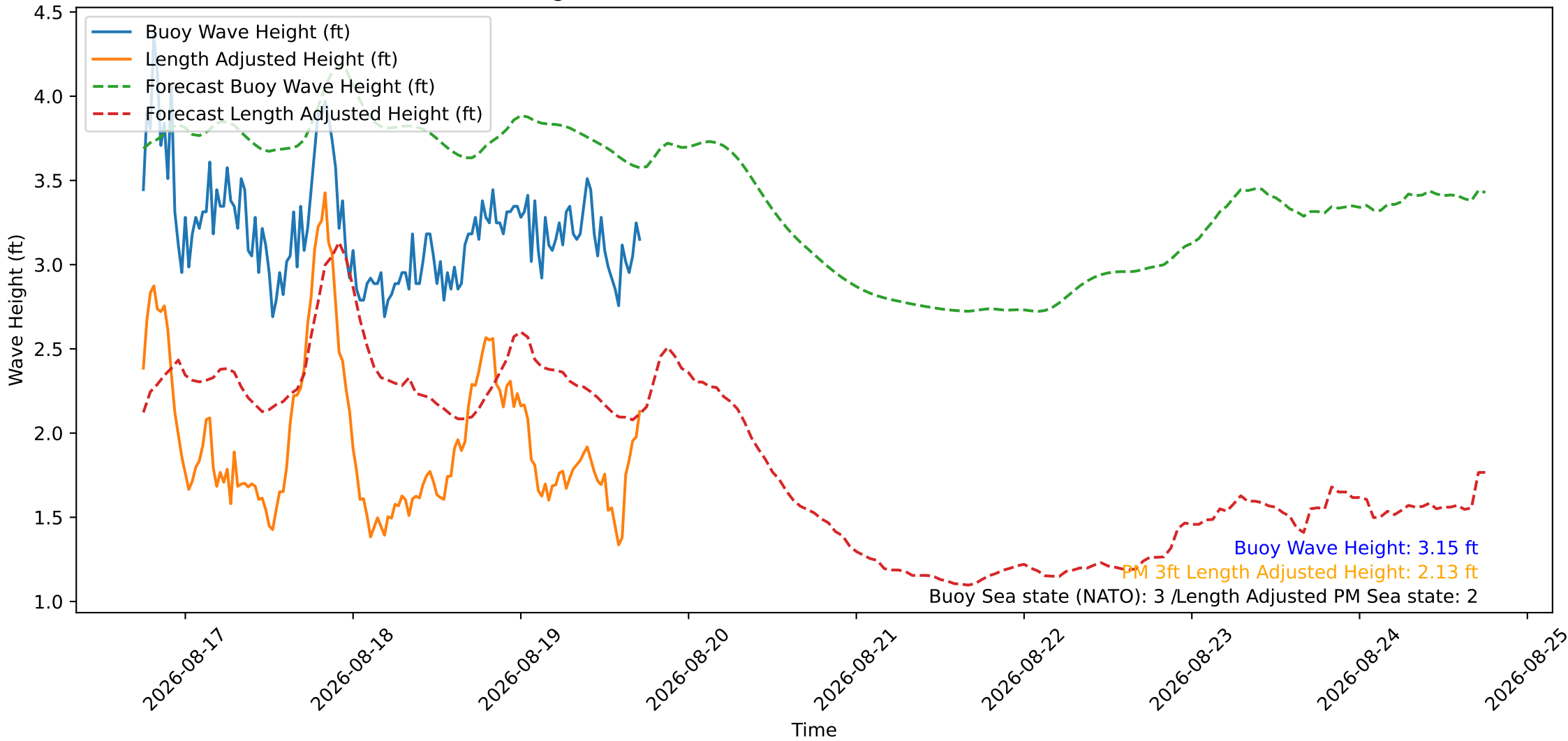
Wave Heights over Time for Green Beach at 2026-08-19 17:41:09
