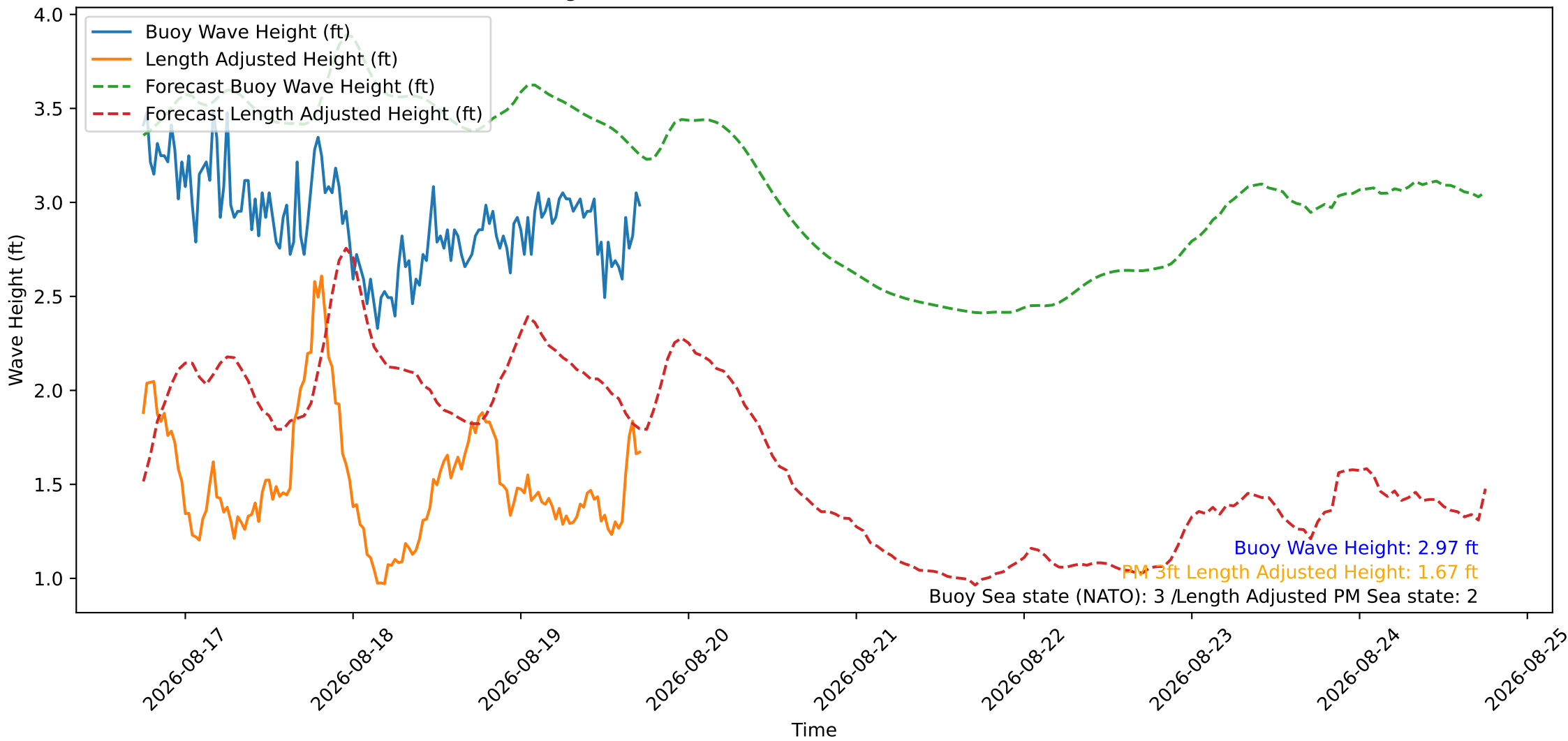
Wave Heights over Time for Red Beach at 2026-08-19 17:40:46
