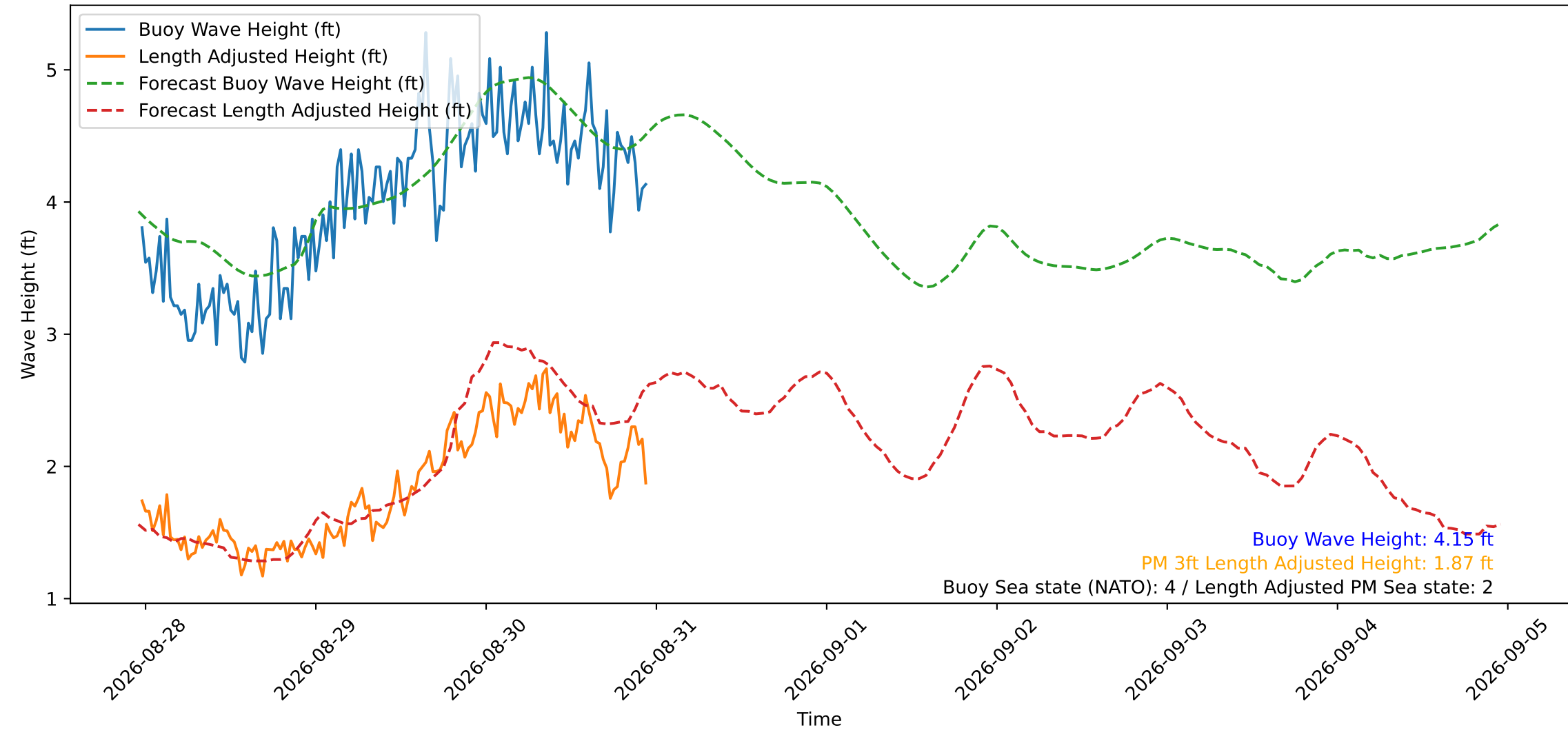
Wave Heights over Time for Oceanside Harbor at 2026-08-30 23:20:30
