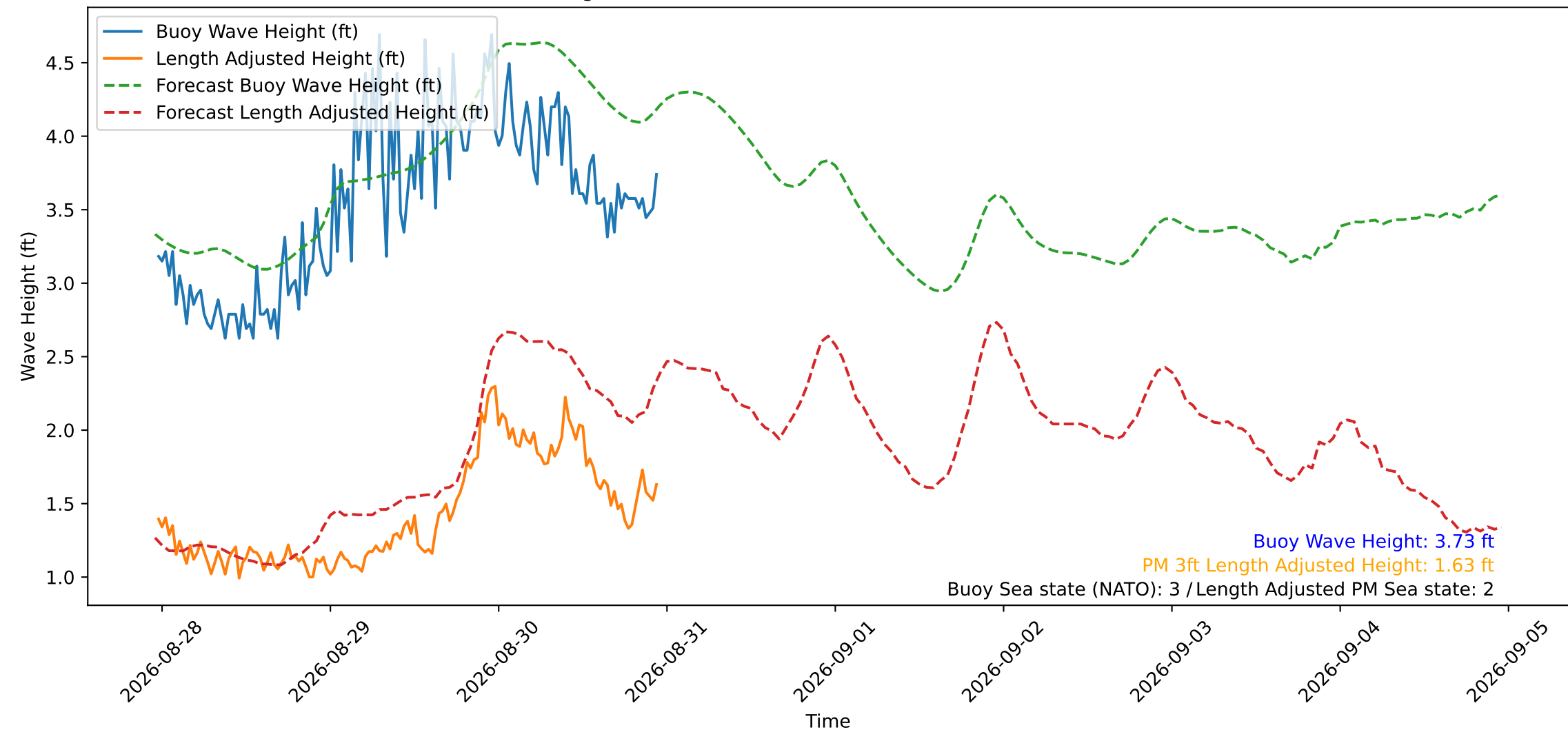
Wave Heights over Time for Red Beach at 2026-08-30 23:20:50
