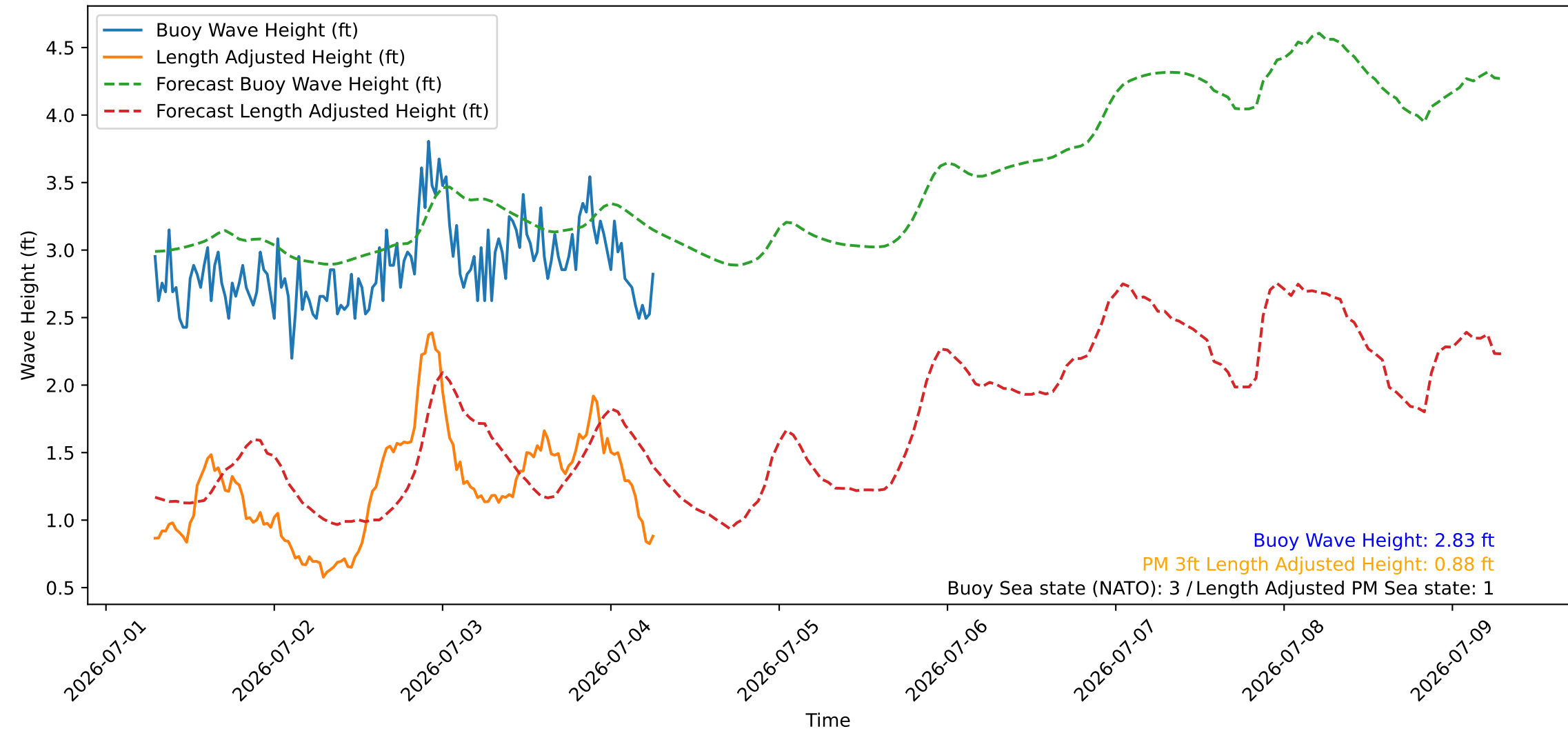
Wave Heights over Time for Red Beach at 2026-07-04 06:40:45
