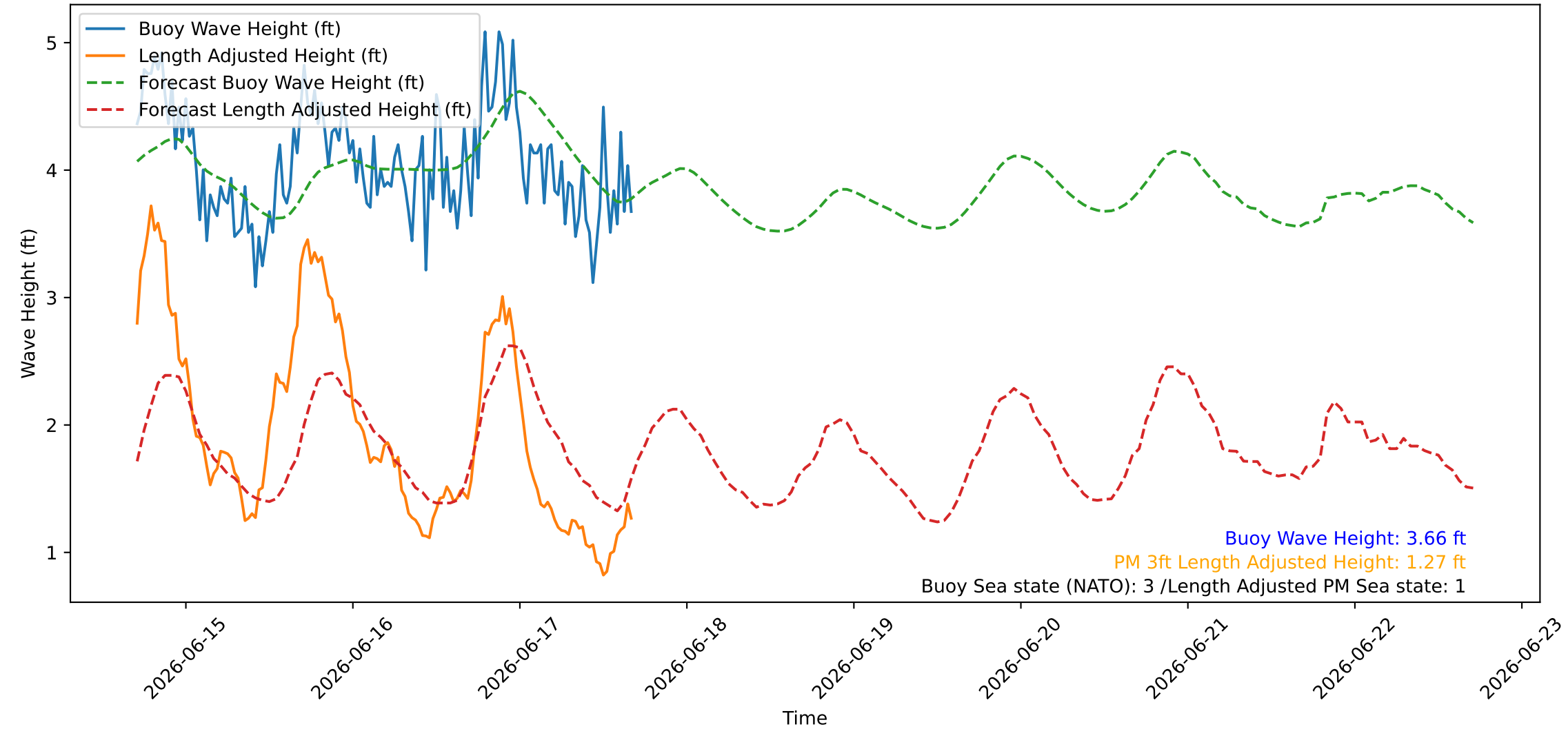
Wave Heights over Time for Green Beach at 2026-06-17 16:51:10
