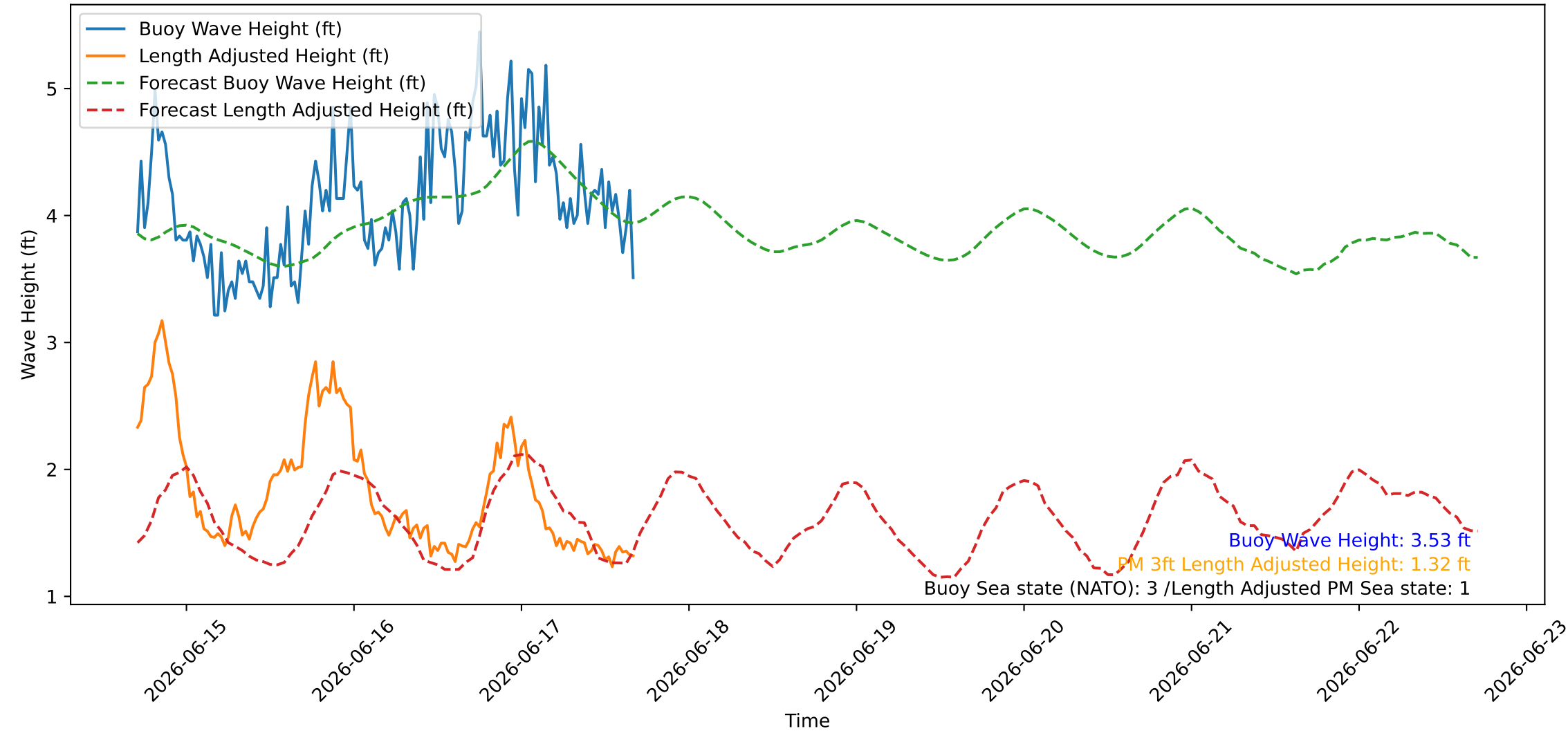
Wave Heights over Time for Oceanside Harbor at 2026-06-17 16:50:27
