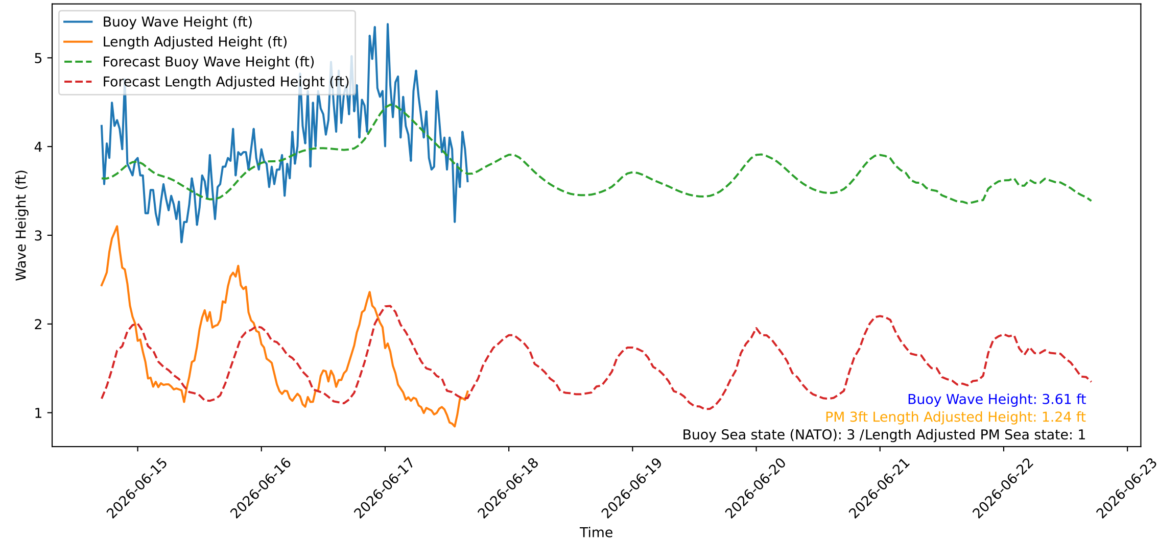
Wave Heights over Time for Red Beach at 2026-06-17 16:50:47
