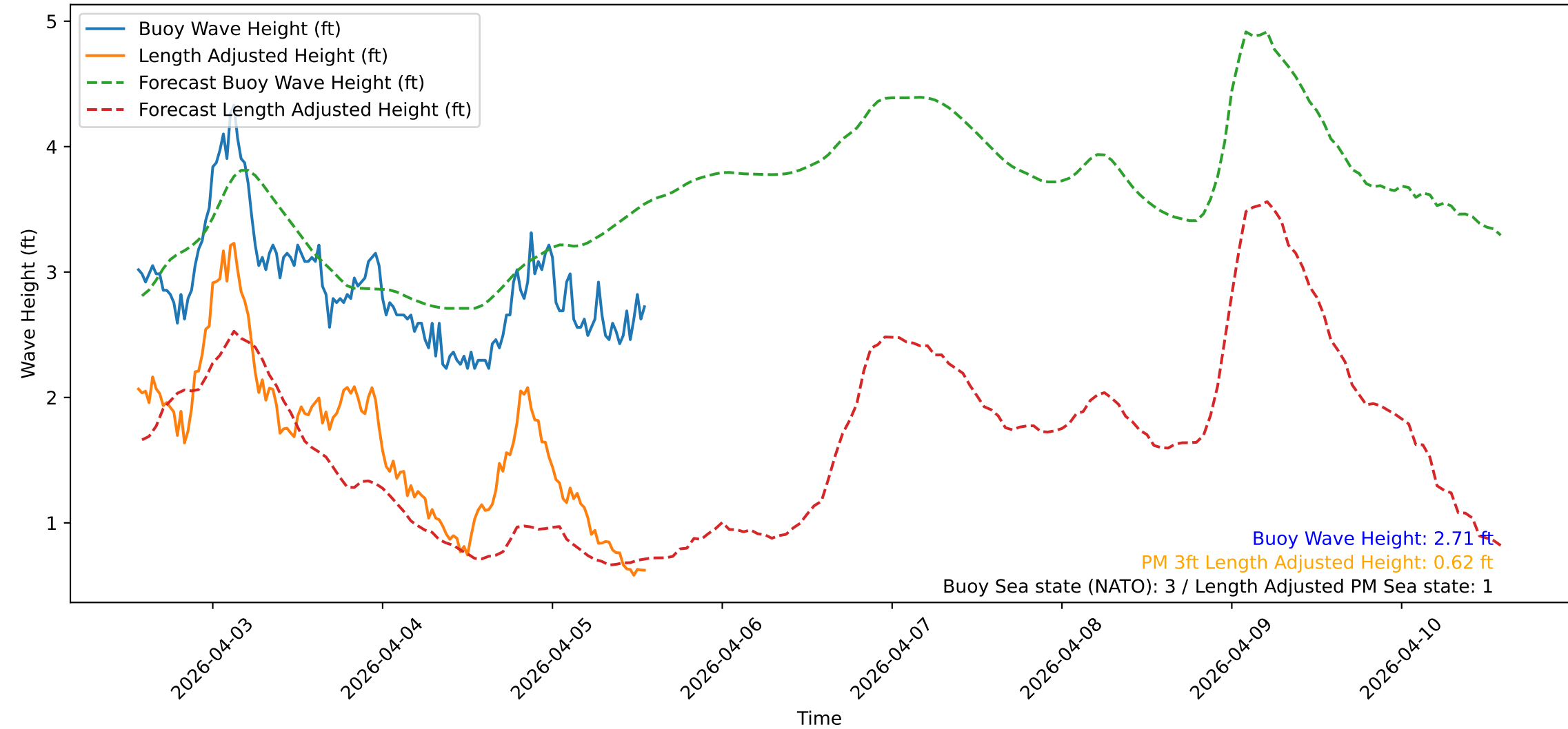
Wave Heights over Time for Green Beach at 2026-04-05 13:41:12
