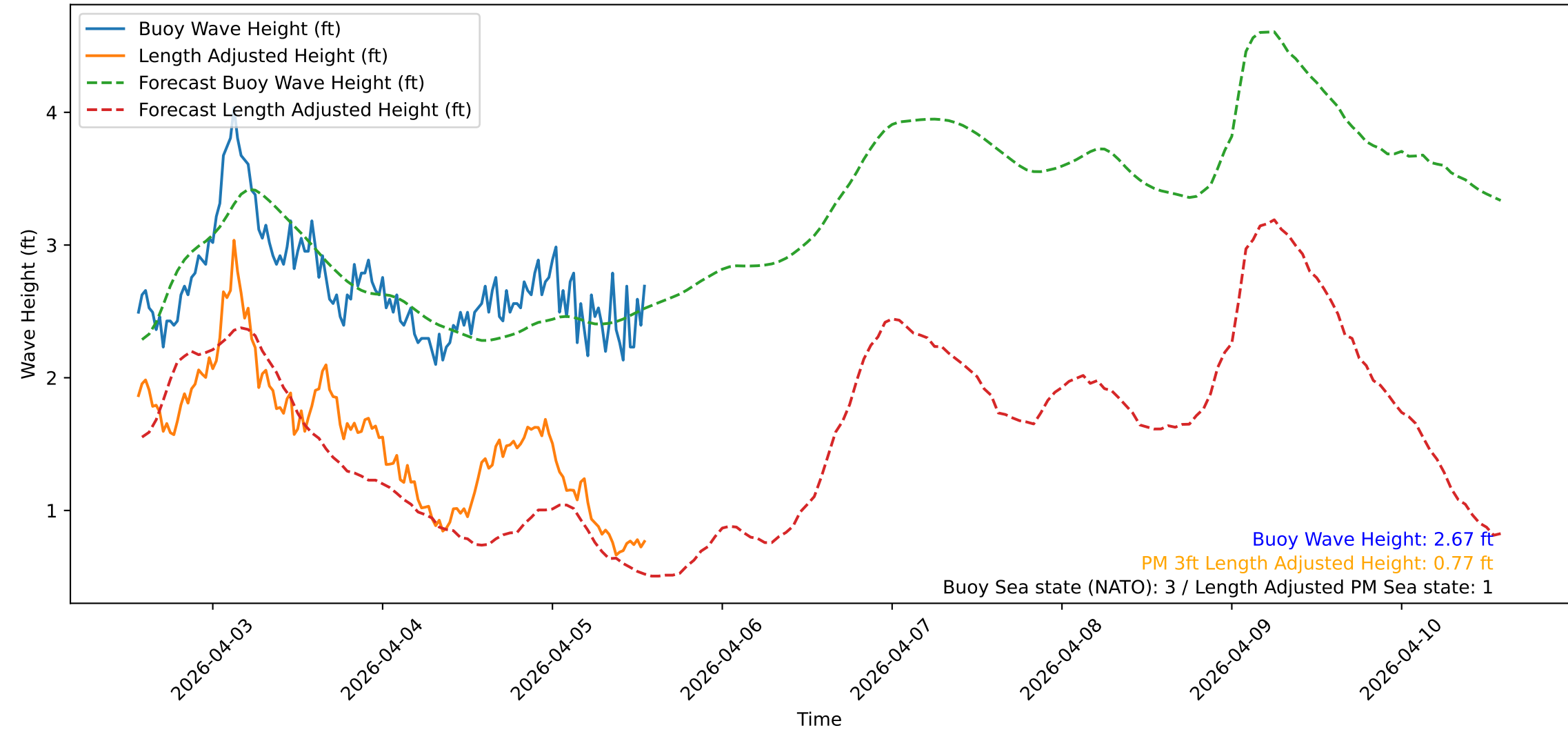
Wave Heights over Time for Oceanside Harbor at 2026-04-05 13:40:32
