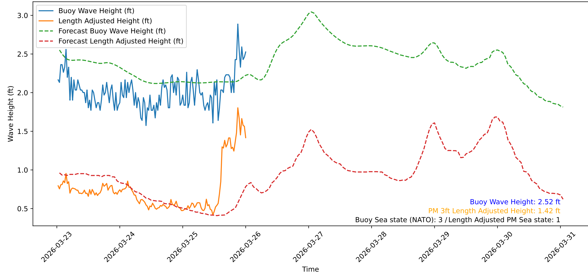
Wave Heights over Time for Oceanside Harbor at 2026-03-26 00:30:31
