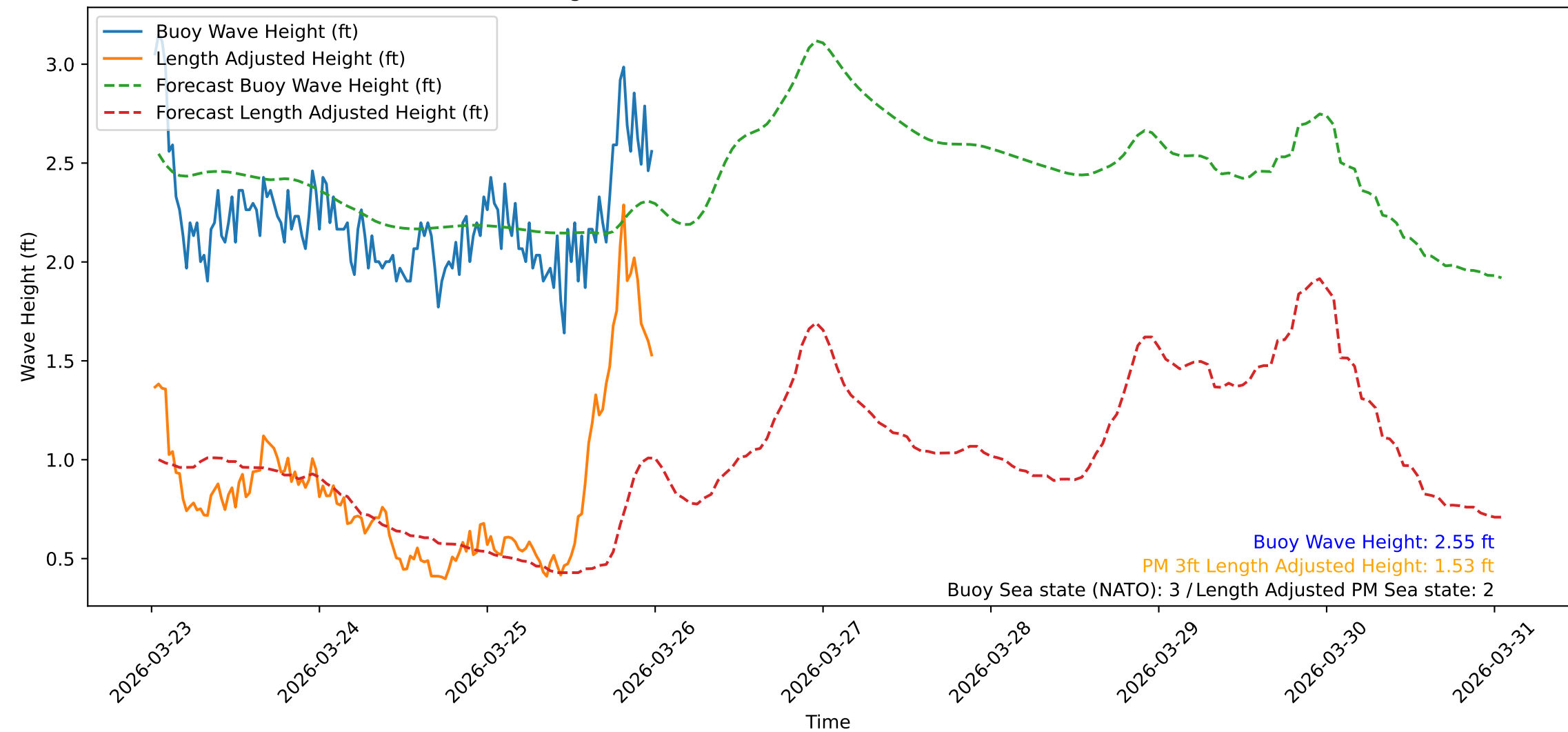
Wave Heights over Time for Green Beach at 2026-03-26 00:31:09
