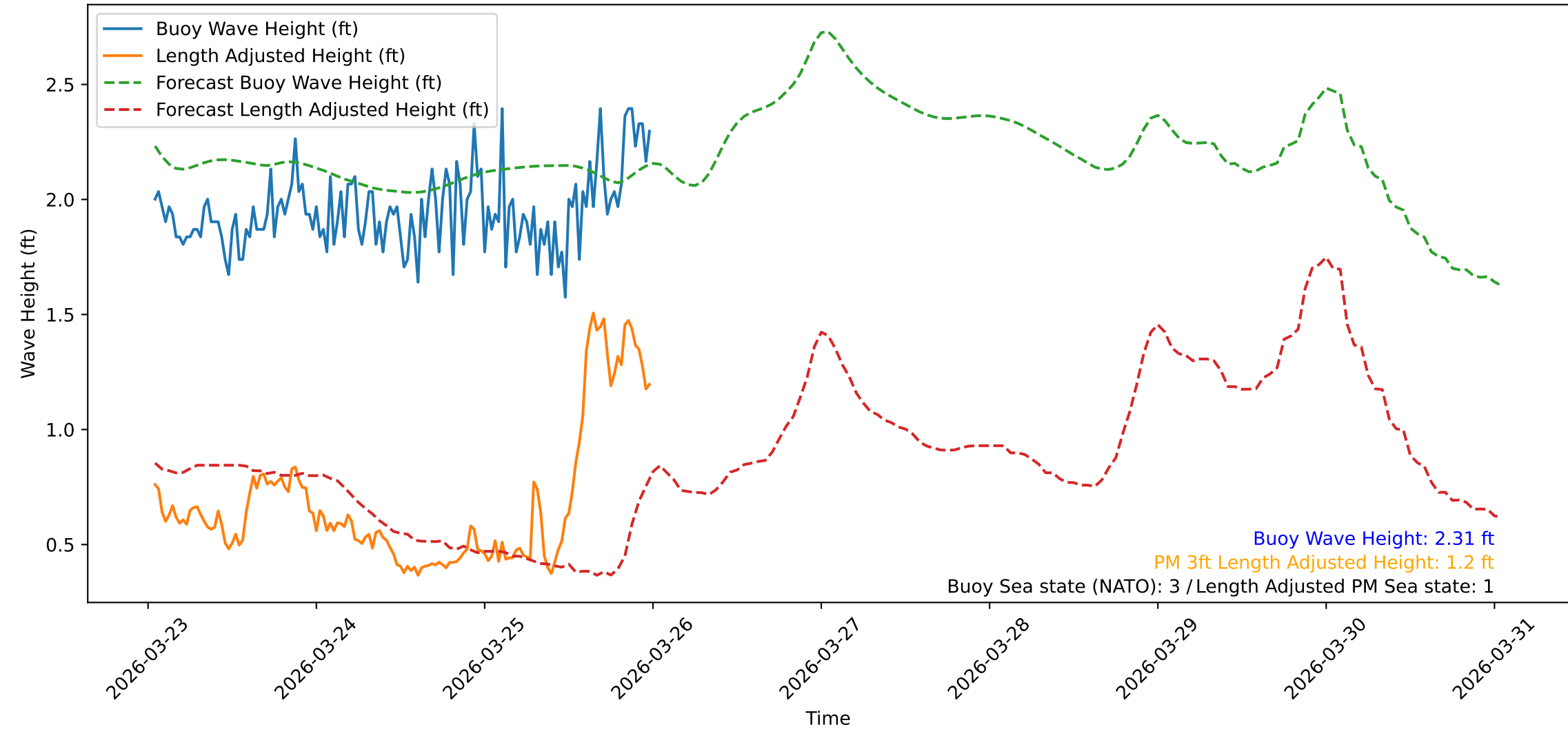
Wave Heights over Time for Red Beach at 2026-03-26 00:30:47
