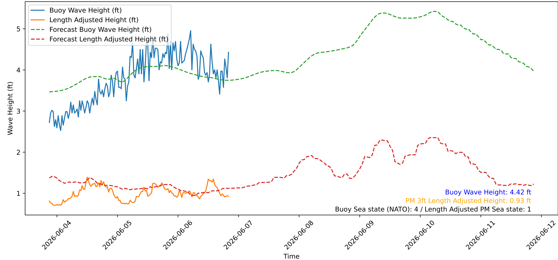
Wave Heights over Time for Red Beach at 2026-06-06 20:50:47
