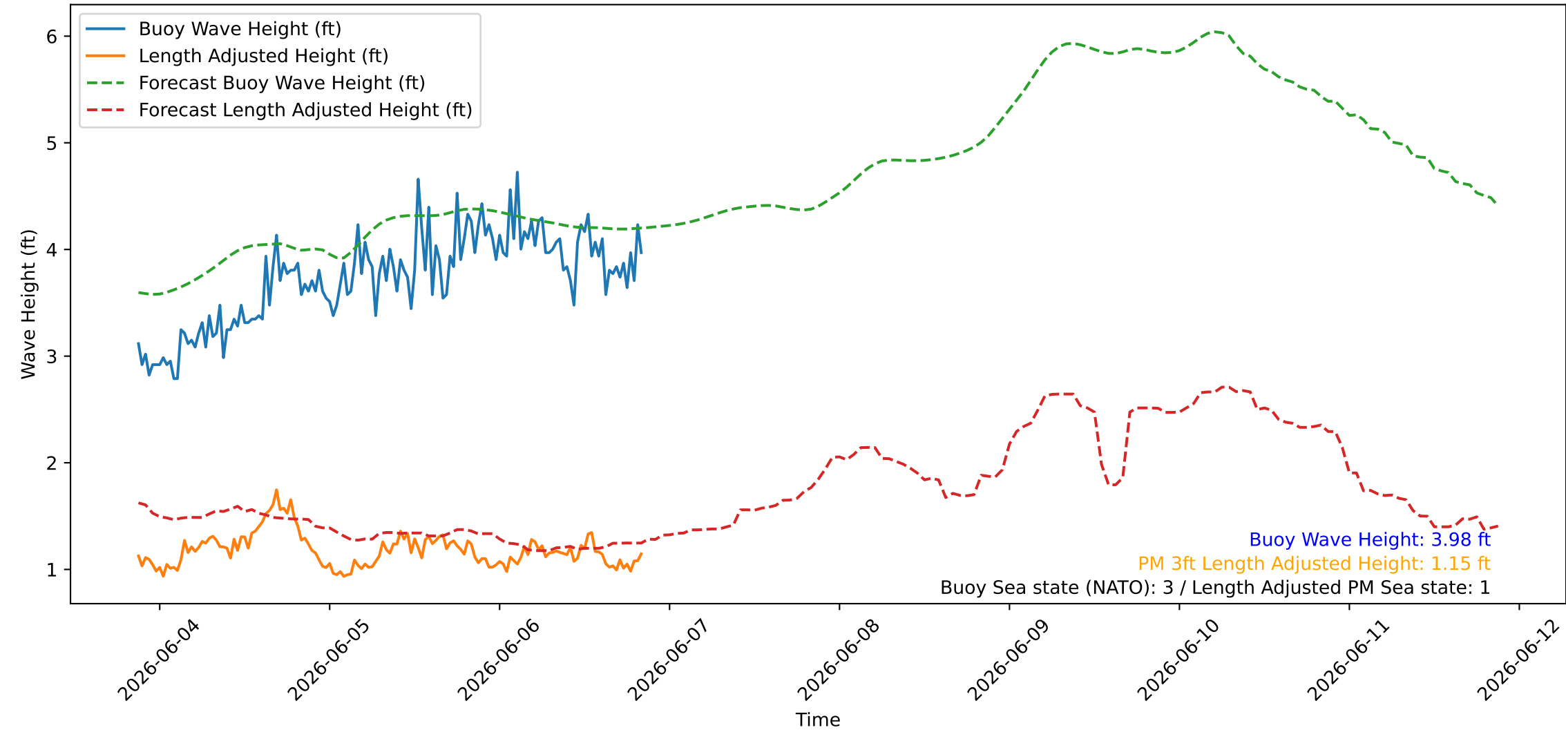
Wave Heights over Time for Green Beach at 2026-06-06 20:51:10
