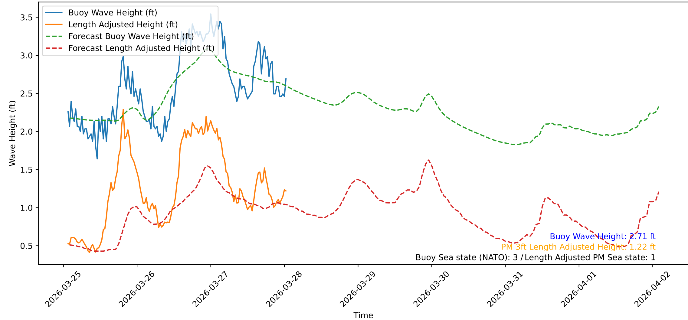
Wave Heights over Time for Green Beach at 2026-03-28 01:31:10
