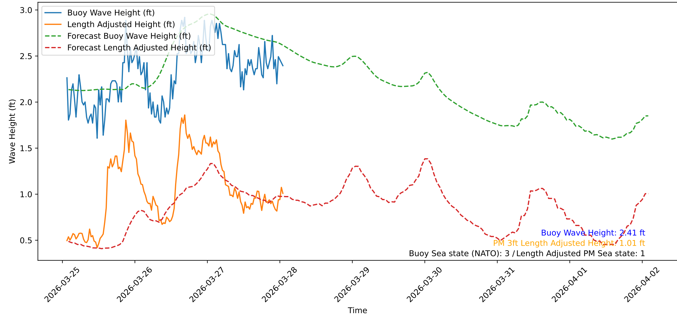
Wave Heights over Time for Oceanside Harbor at 2026-03-28 01:30:31
