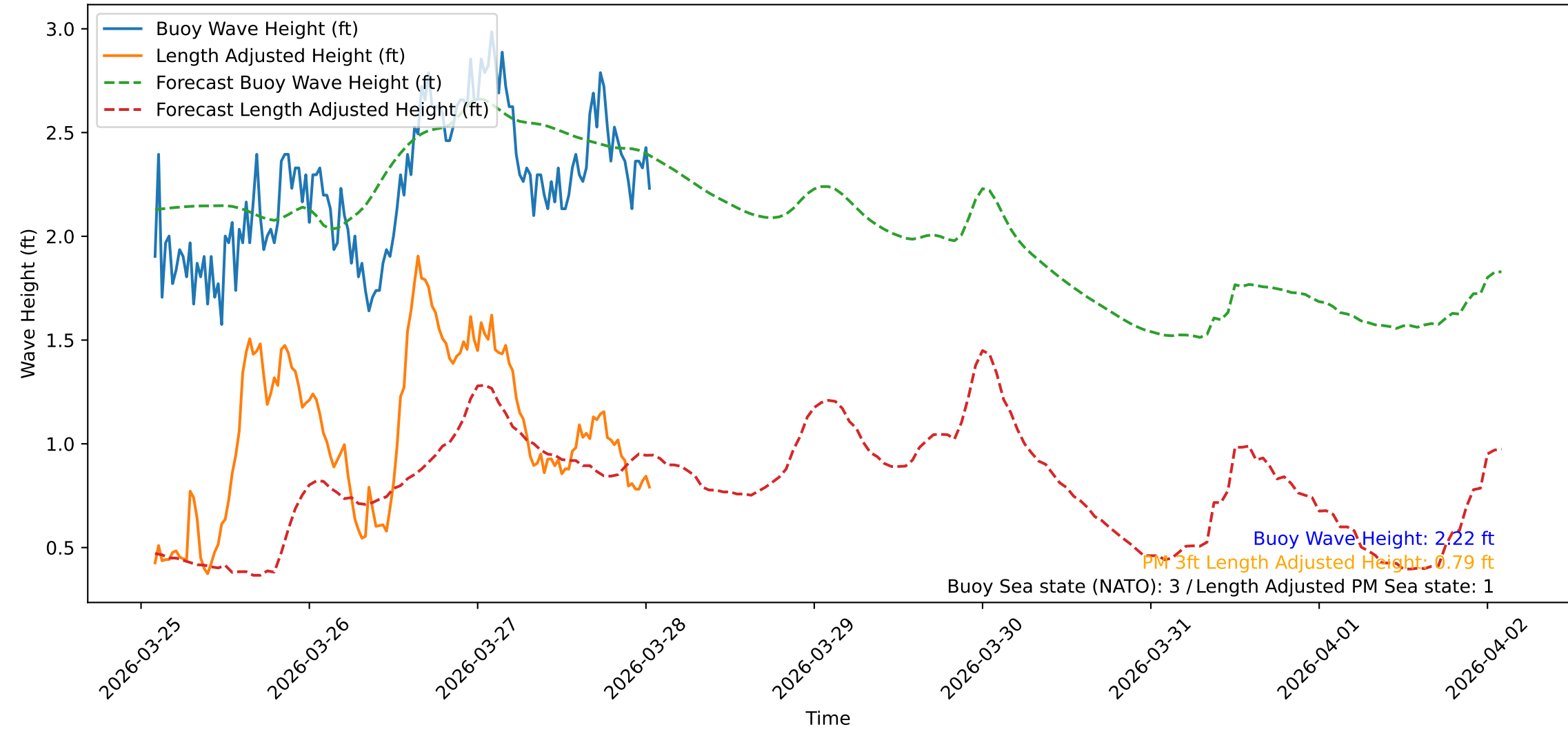
Wave Heights over Time for Red Beach at 2026-03-28 01:30:47
