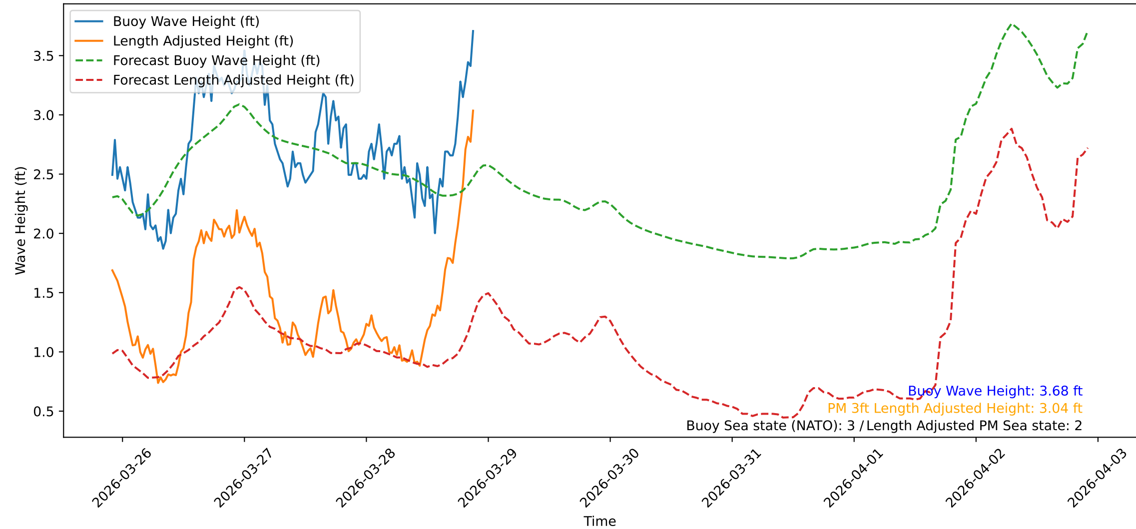
Wave Heights over Time for Green Beach at 2026-03-28 21:51:09
