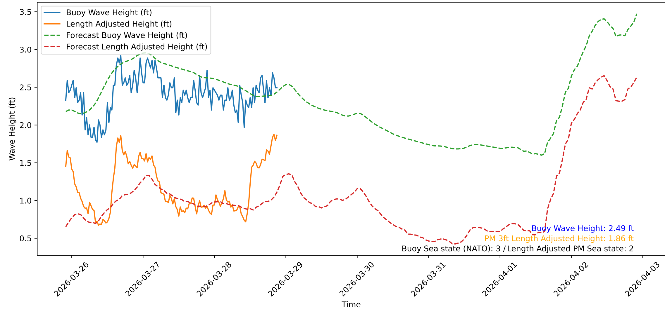
Wave Heights over Time for Oceanside Harbor at 2026-03-28 21:50:31
