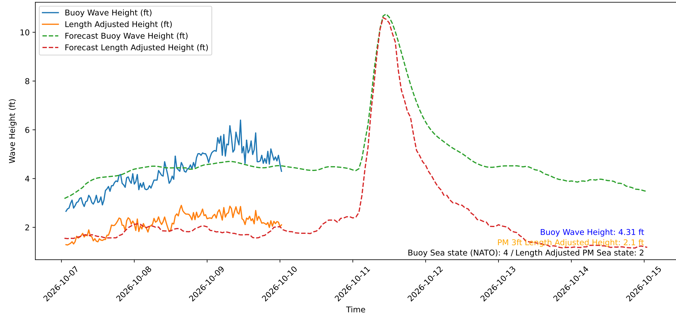
Wave Heights over Time for Oceanside Harbor at 2026-10-10 01:20:29
