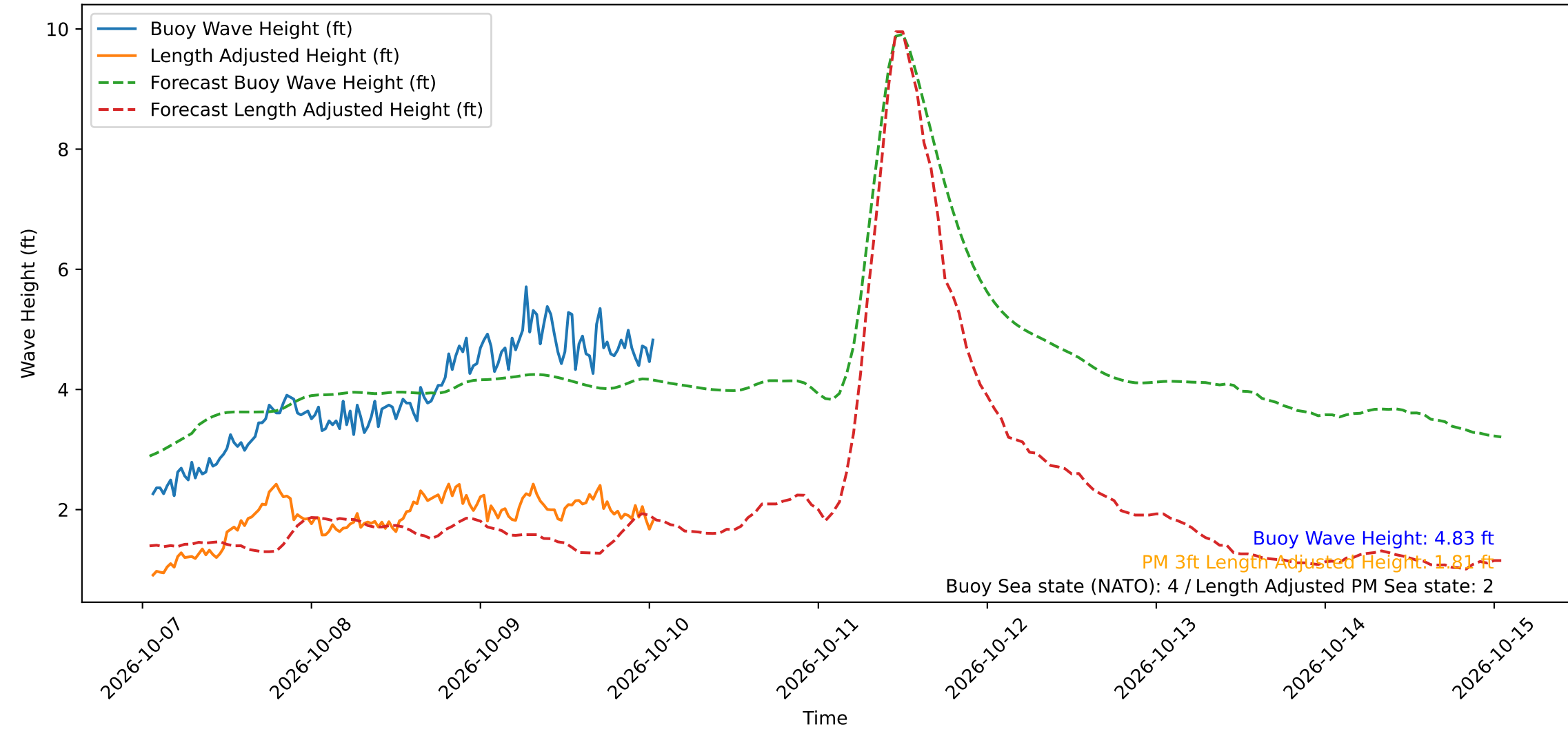
Wave Heights over Time for Red Beach at 2026-10-10 01:20:50
