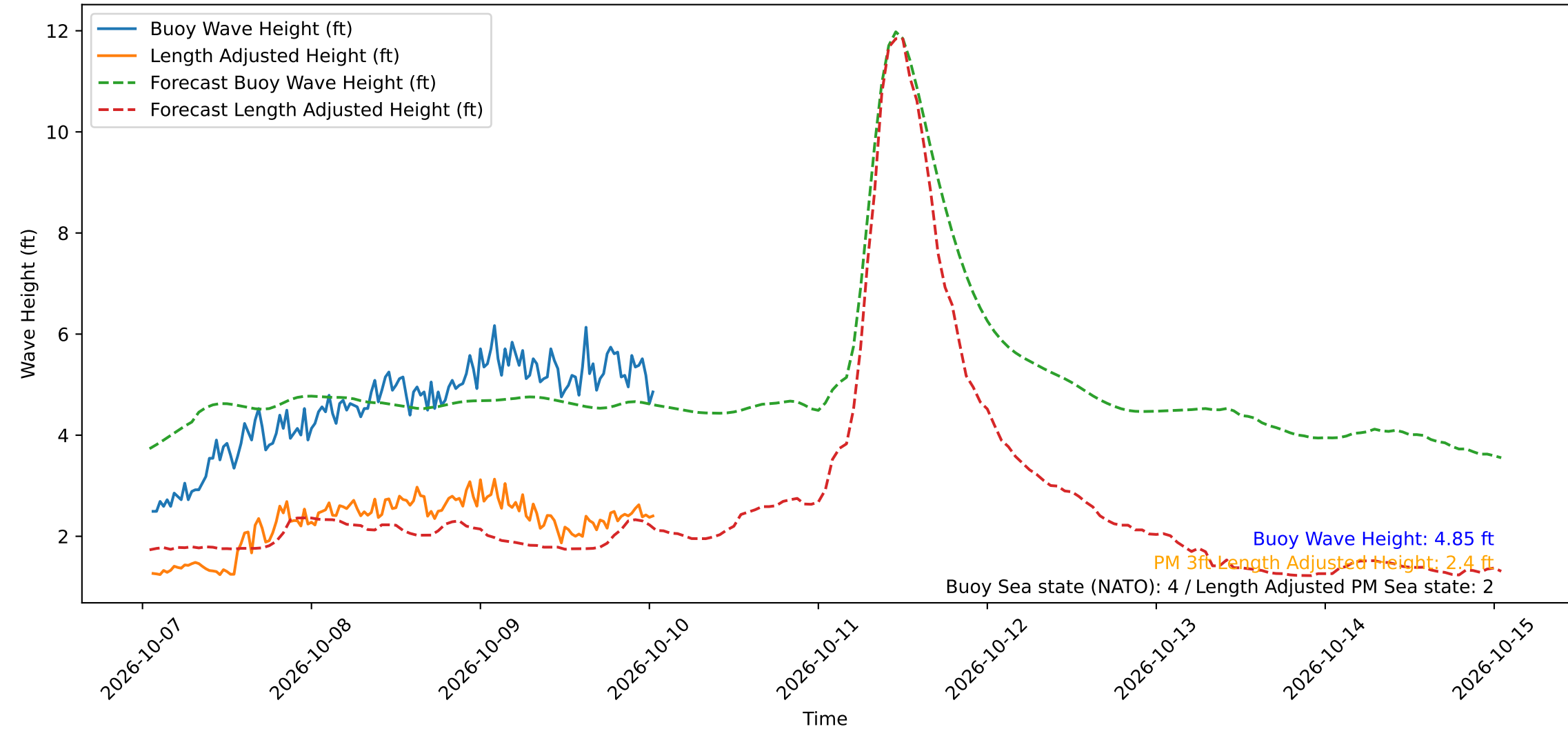
Wave Heights over Time for Green Beach at 2026-10-10 01:21:14
