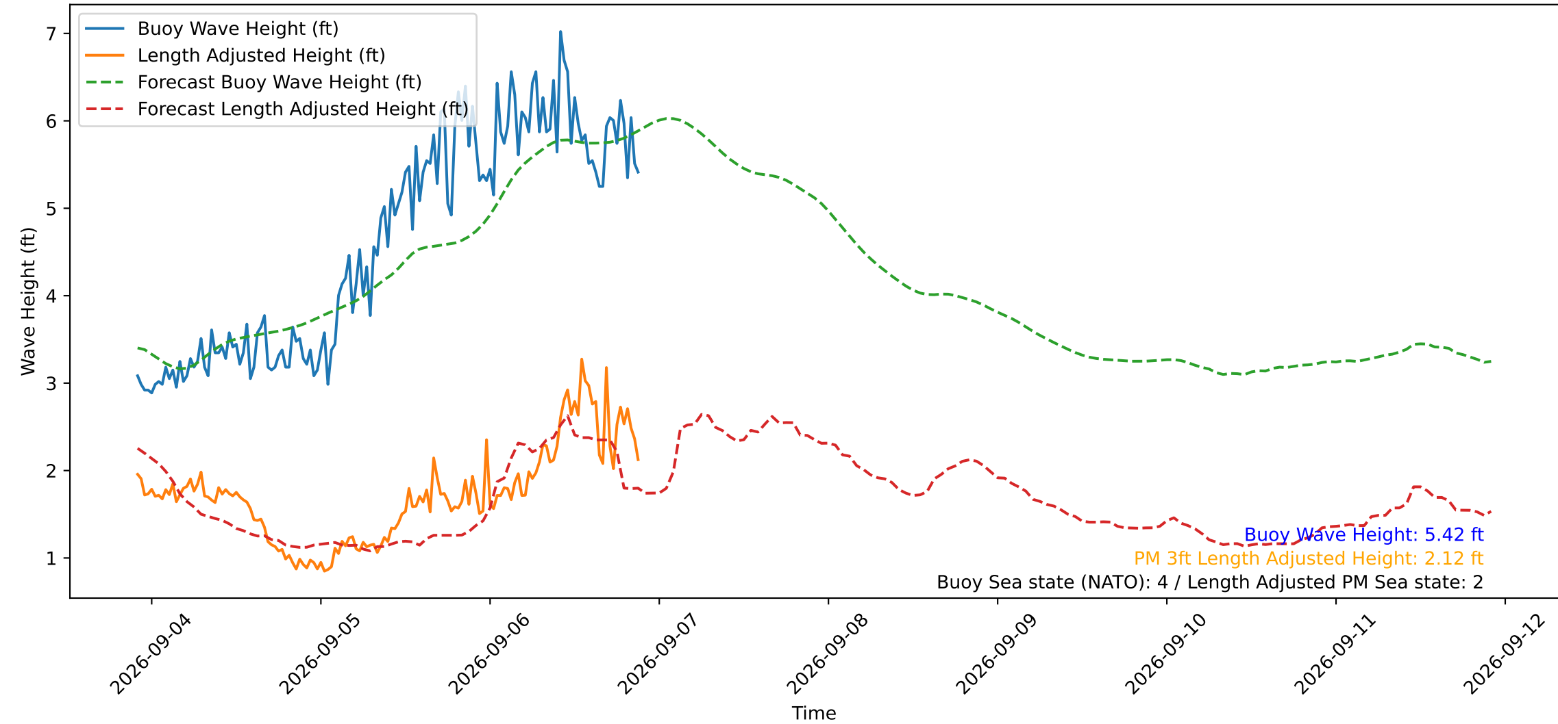
Wave Heights over Time for Oceanside Harbor at 2026-09-06 21:50:30
