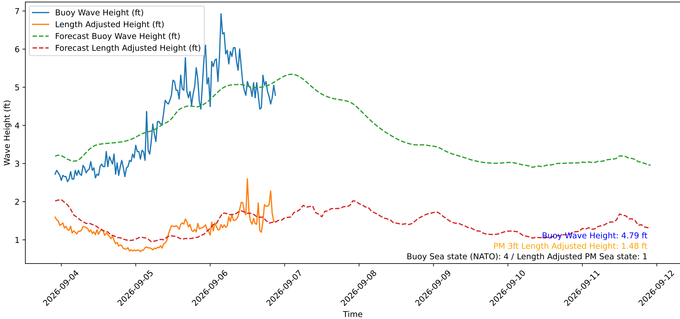
Wave Heights over Time for Red Beach at 2026-09-06 21:50:50
