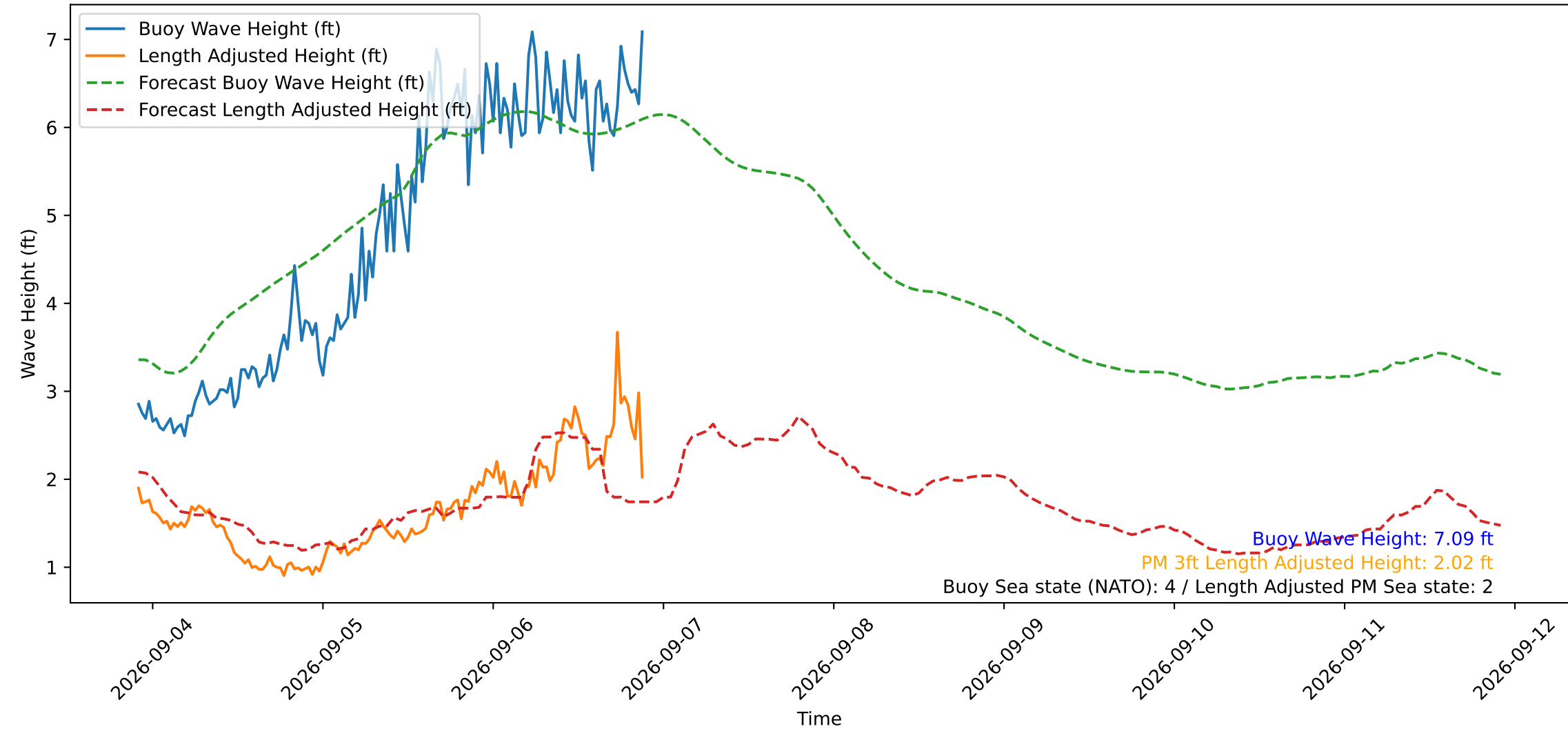
Wave Heights over Time for Green Beach at 2026-09-06 21:51:14
