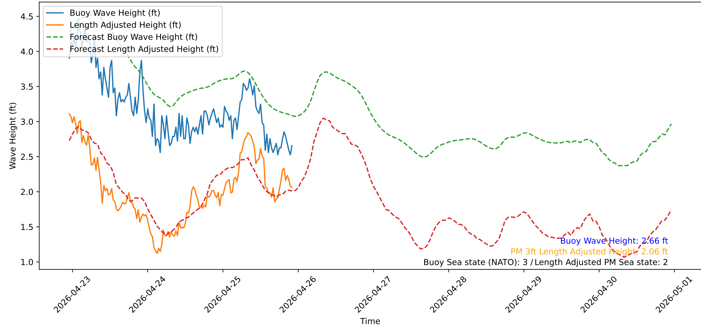
Wave Heights over Time for Oceanside Harbor at 2026-04-25 22:50:30
