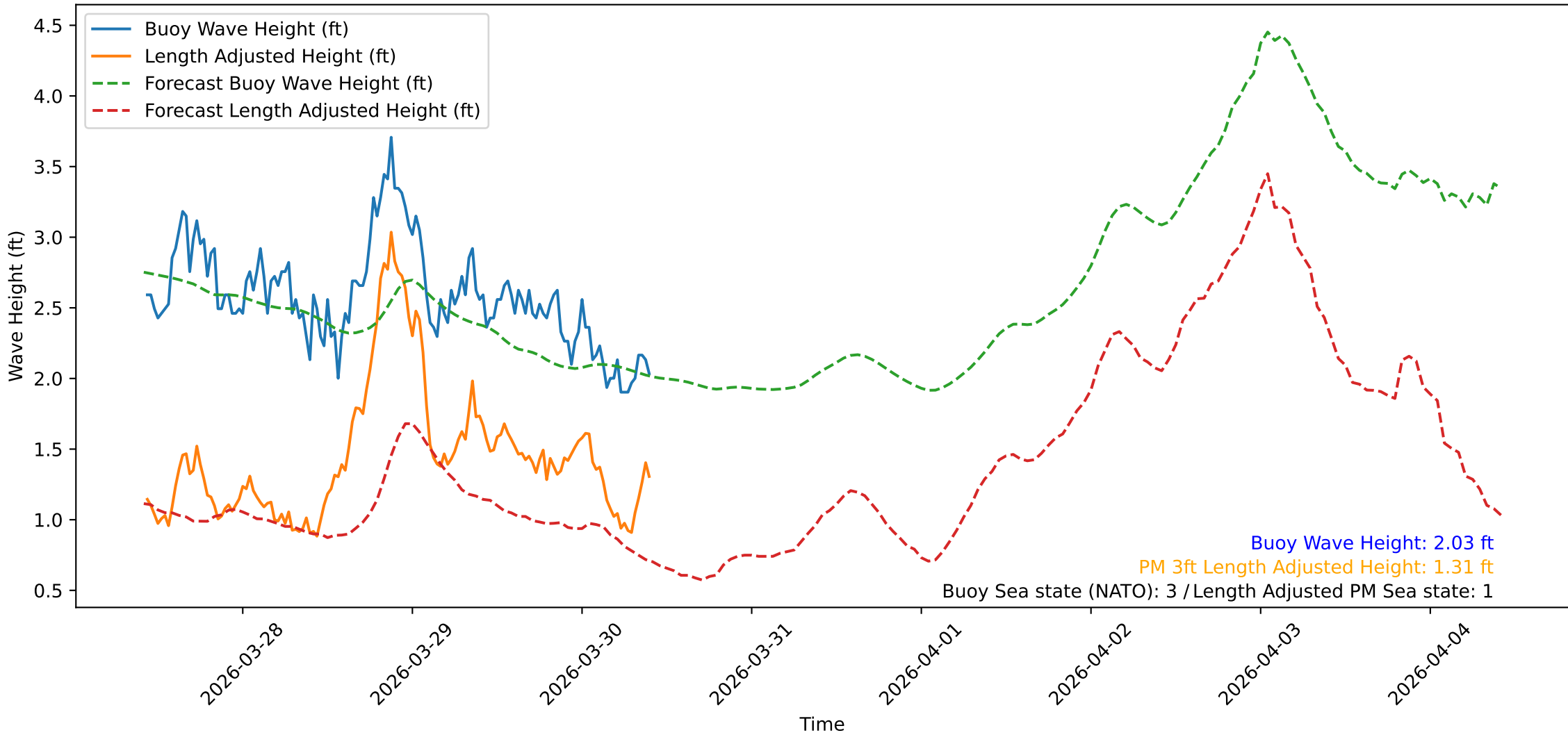
Wave Heights over Time for Green Beach at 2026-03-30 10:21:10
