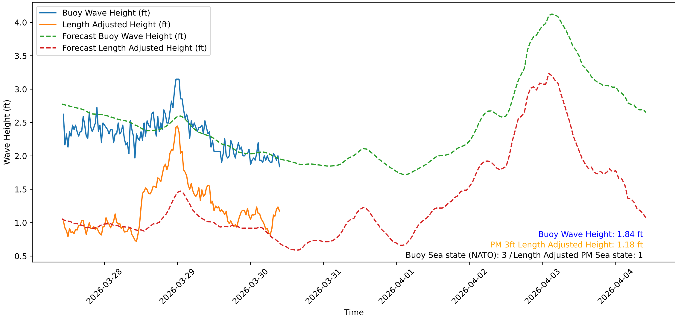
Wave Heights over Time for Oceanside Harbor at 2026-03-30 10:20:31
