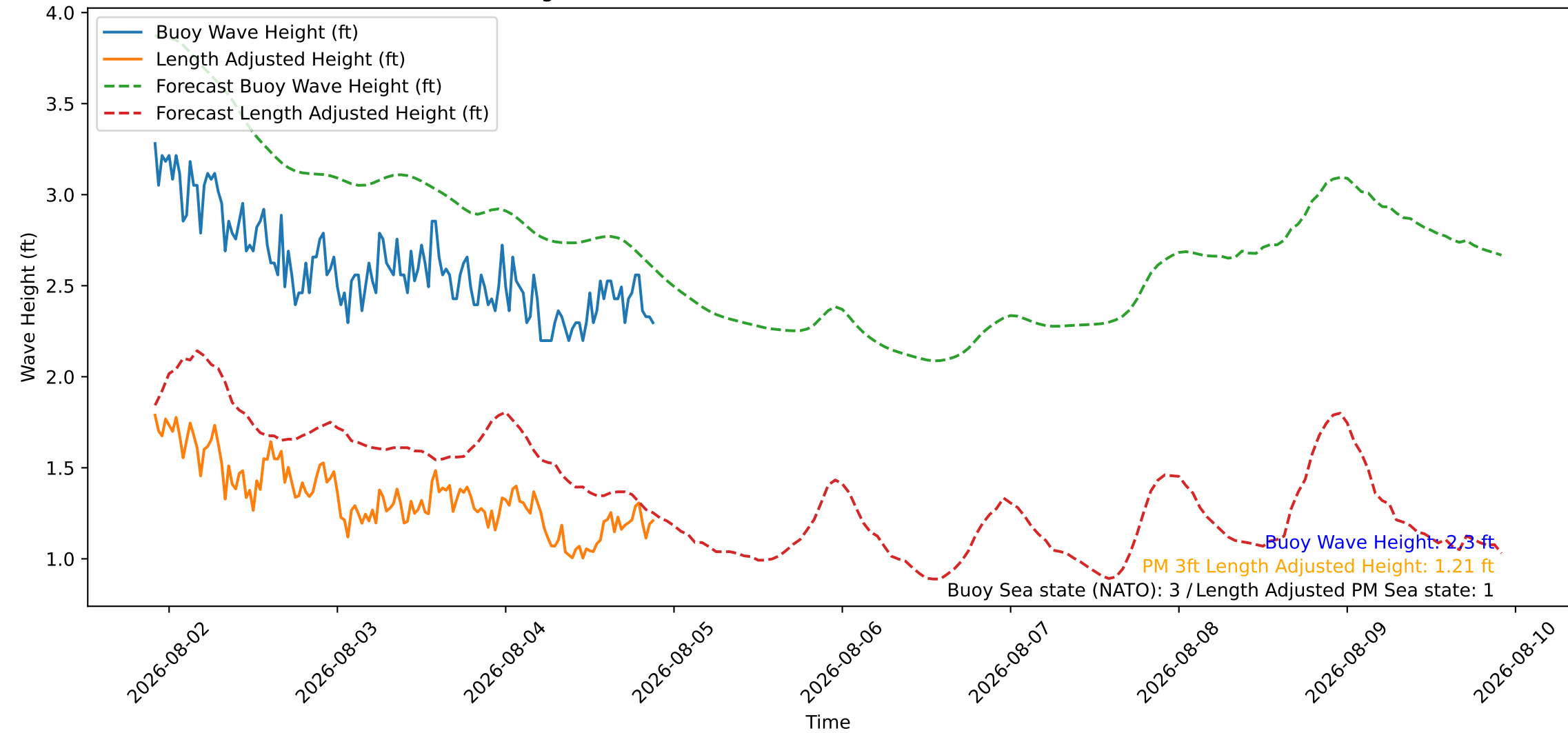
Wave Heights over Time for Oceanside Harbor at 2026-08-04 21:50:27
