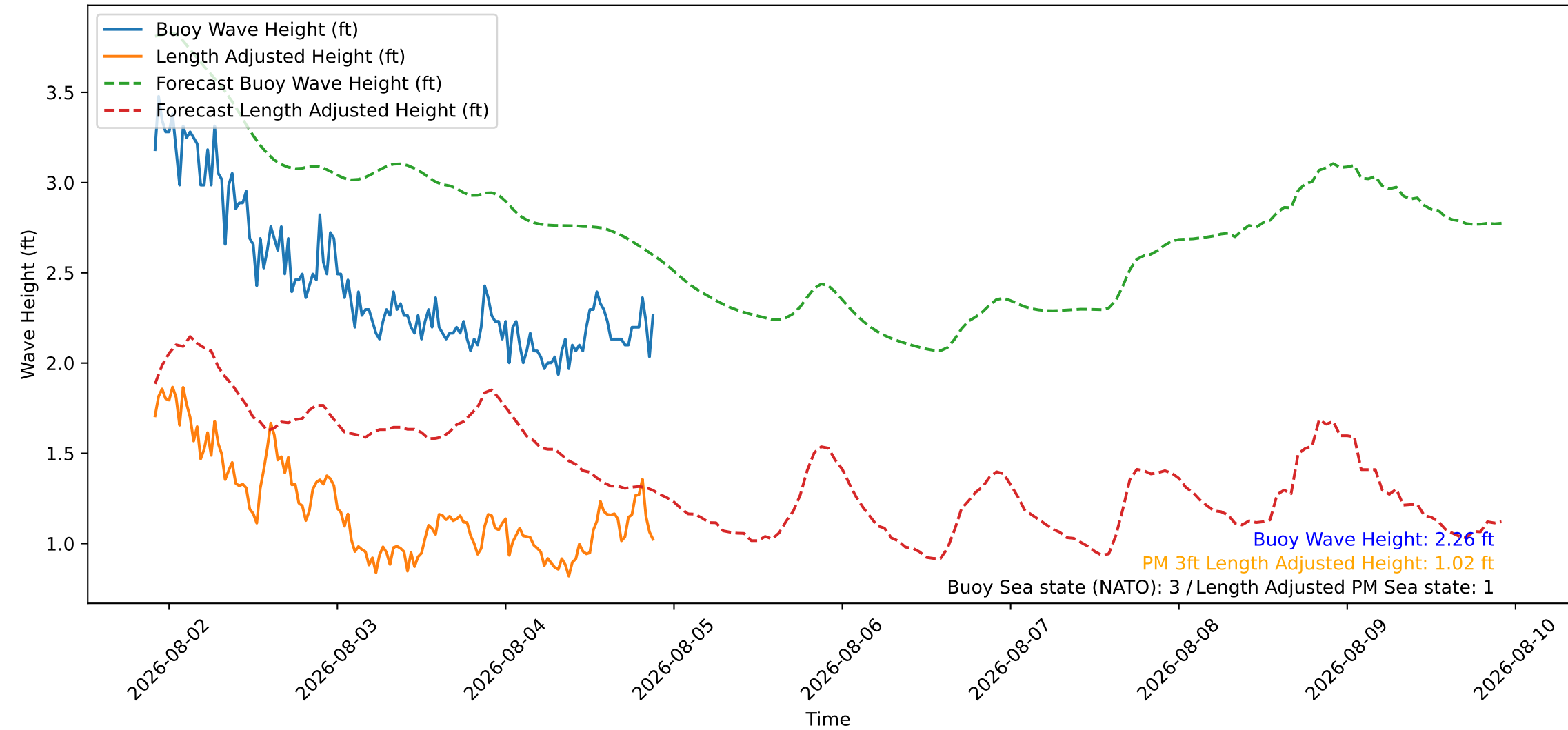
Wave Heights over Time for Green Beach at 2026-08-04 21:51:10
