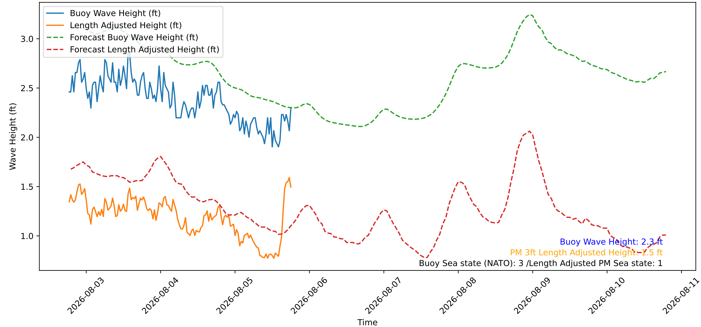
Wave Heights over Time for Oceanside Harbor at 2026-08-05 18:40:26
