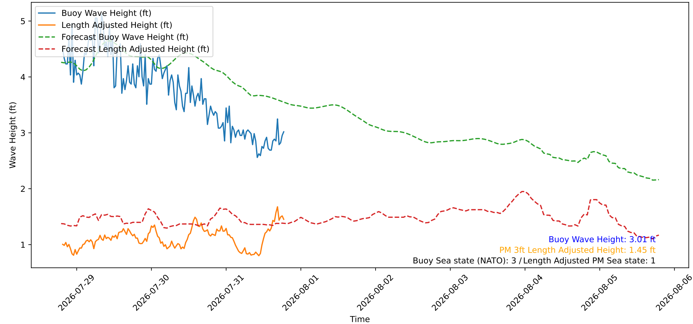
Wave Heights over Time for Red Beach at 2026-07-31 19:20:47
