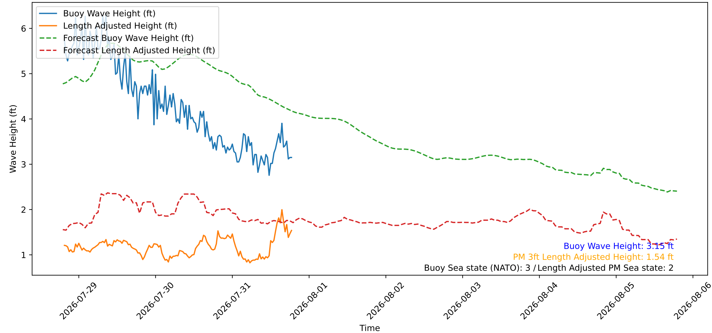
Wave Heights over Time for Green Beach at 2026-07-31 19:21:11
