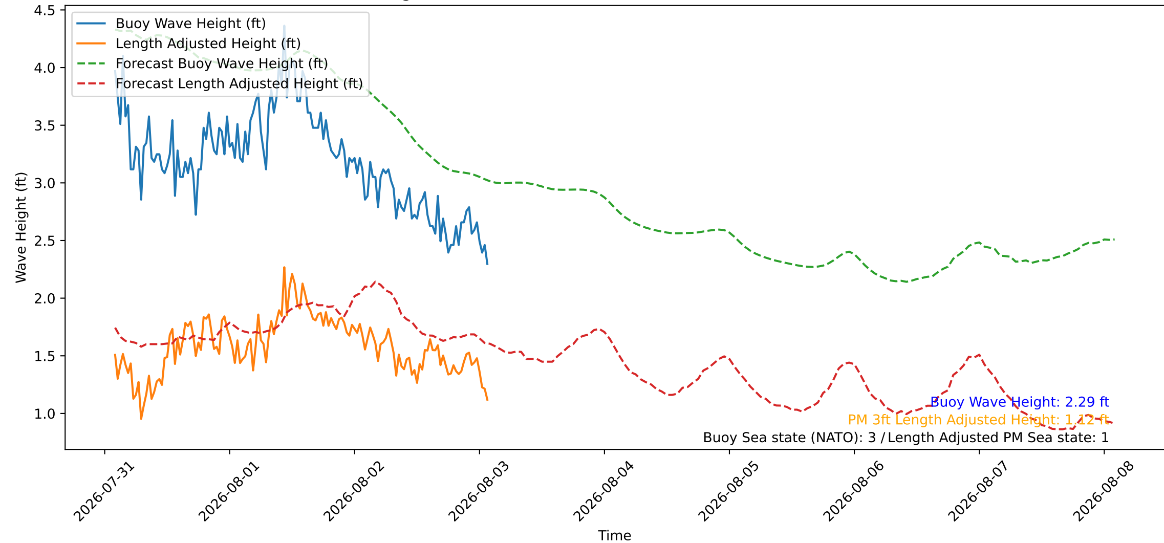
Wave Heights over Time for Oceanside Harbor at 2026-08-03 02:00:26
