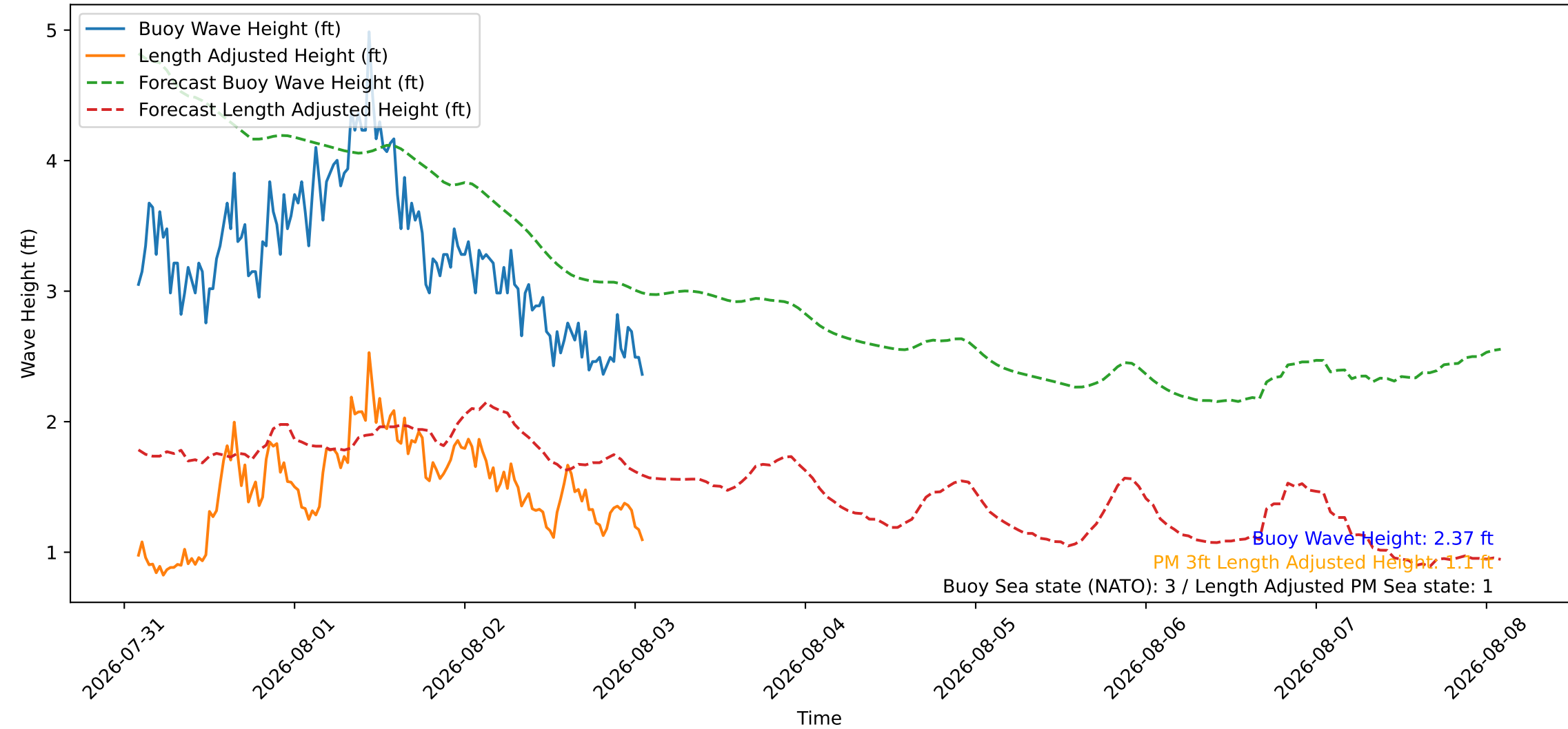
Wave Heights over Time for Green Beach at 2026-08-03 02:01:08
