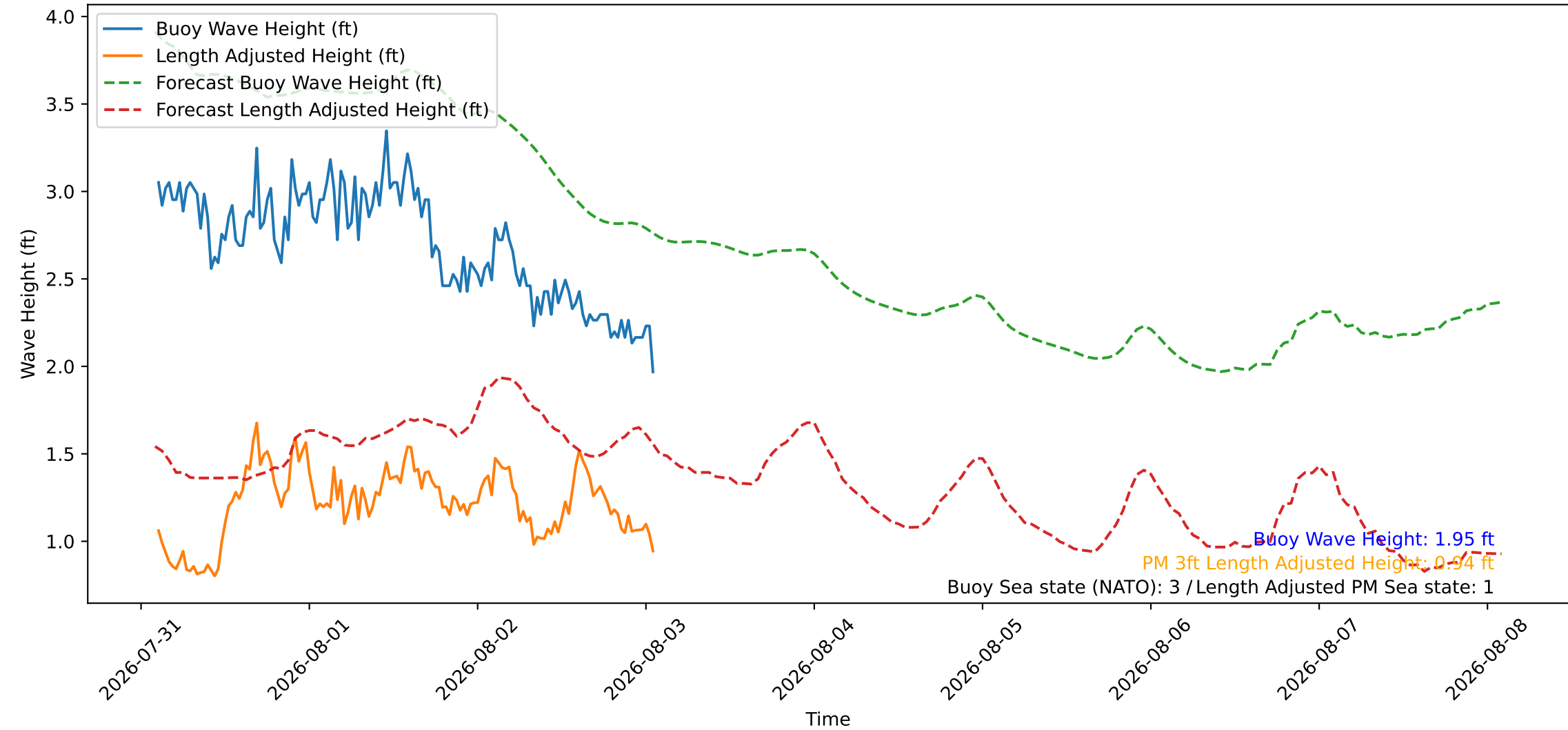
Wave Heights over Time for Red Beach at 2026-08-03 02:00:45
