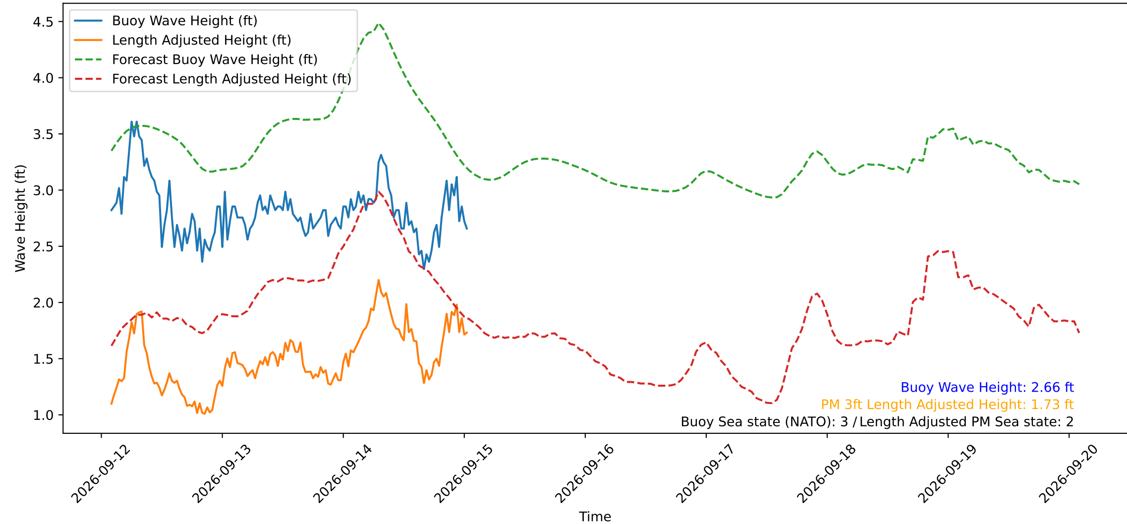
Wave Heights over Time for Green Beach at 2026-09-15 01:31:11
