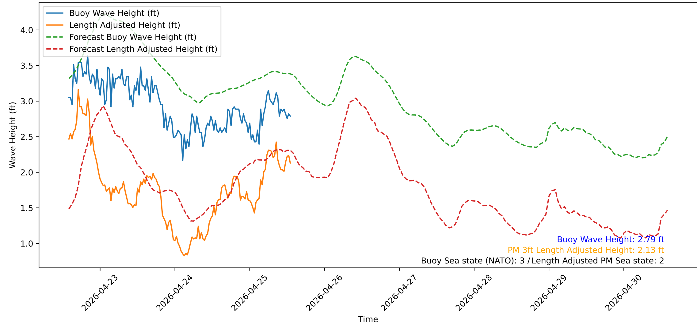
Wave Heights over Time for Red Beach at 2026-04-25 13:40:50
