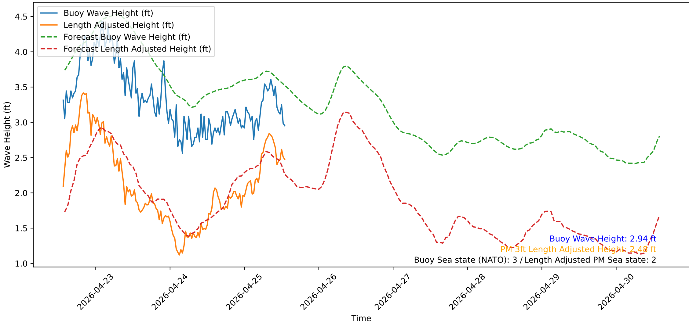
Wave Heights over Time for Oceanside Harbor at 2026-04-25 13:40:31
