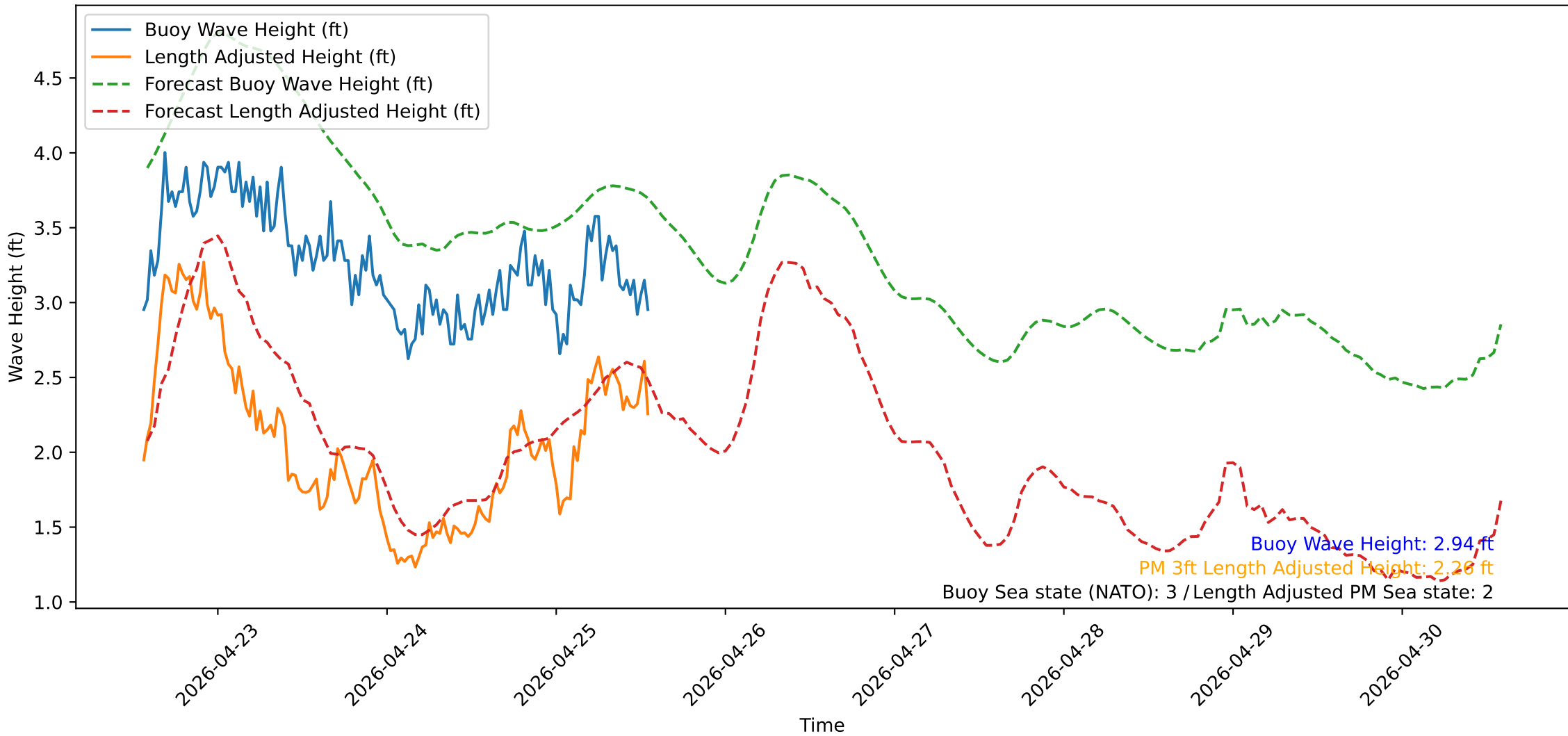
Wave Heights over Time for Green Beach at 2026-04-25 13:41:12
