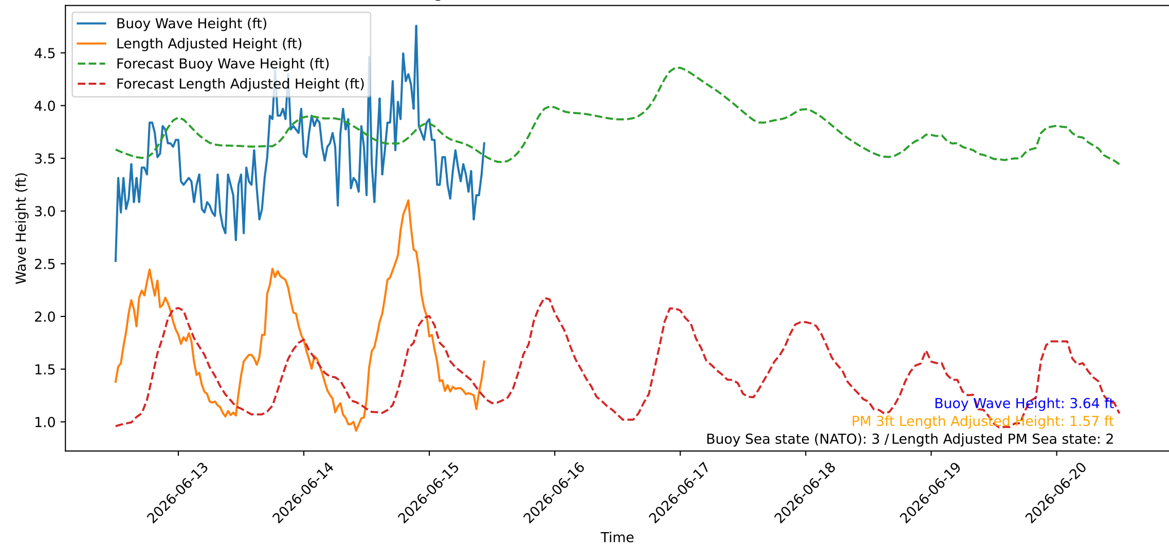
Wave Heights over Time for Red Beach at 2026-06-15 11:30:45
