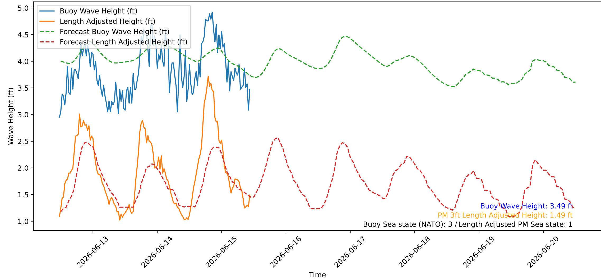
Wave Heights over Time for Green Beach at 2026-06-15 11:31:08
