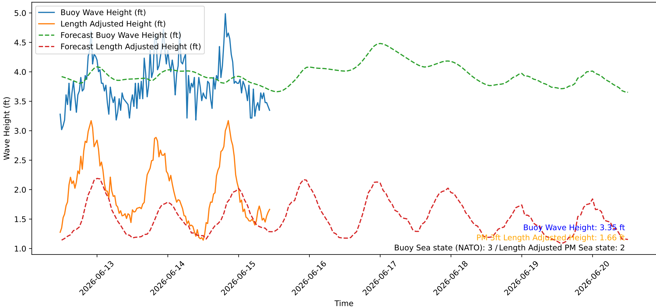
Wave Heights over Time for Oceanside Harbor at 2026-06-15 11:30:26
