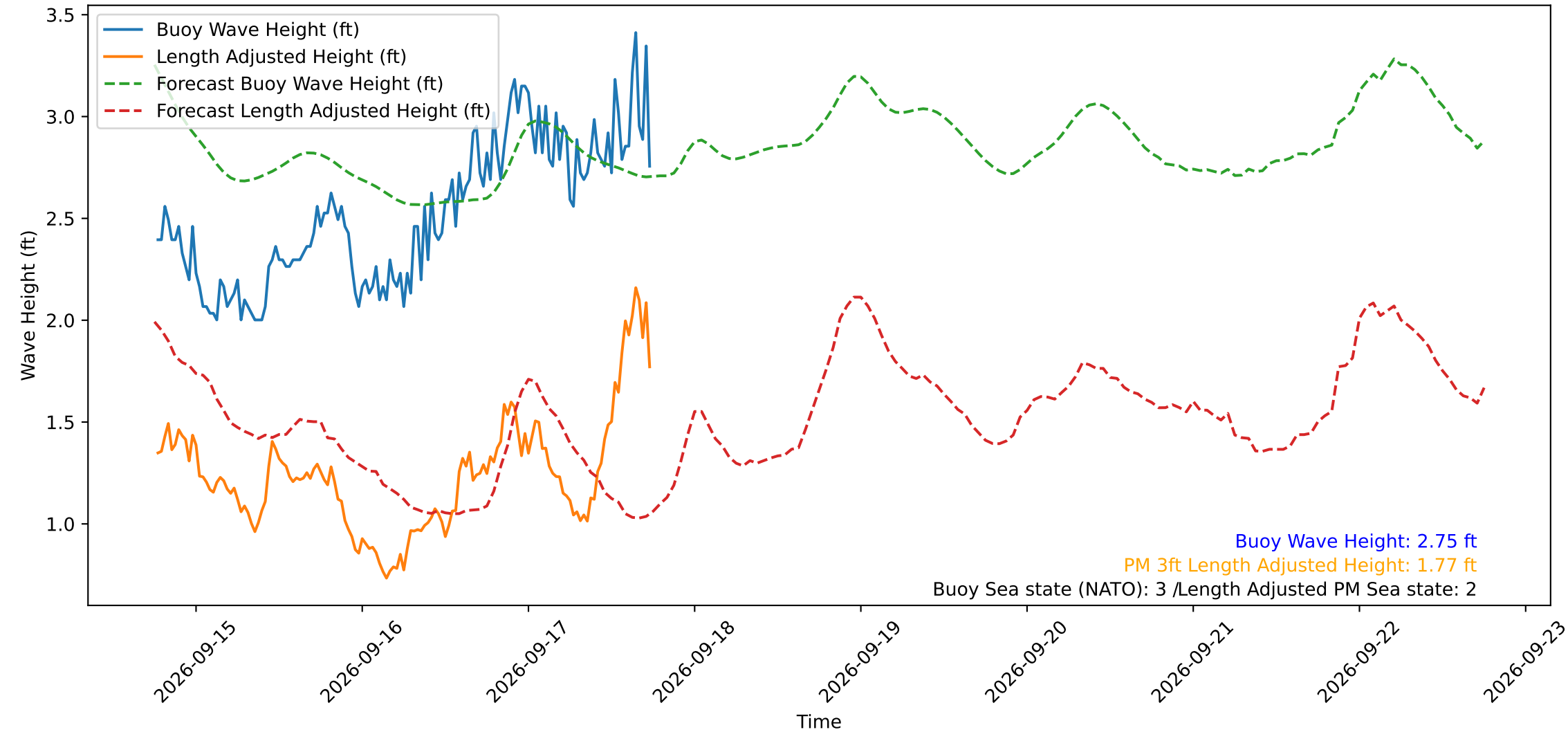
Wave Heights over Time for Red Beach at 2026-09-17 18:20:51
