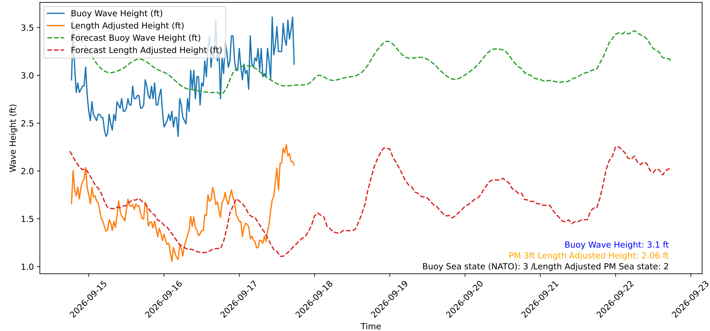
Wave Heights over Time for Oceanside Harbor at 2026-09-17 18:20:30
