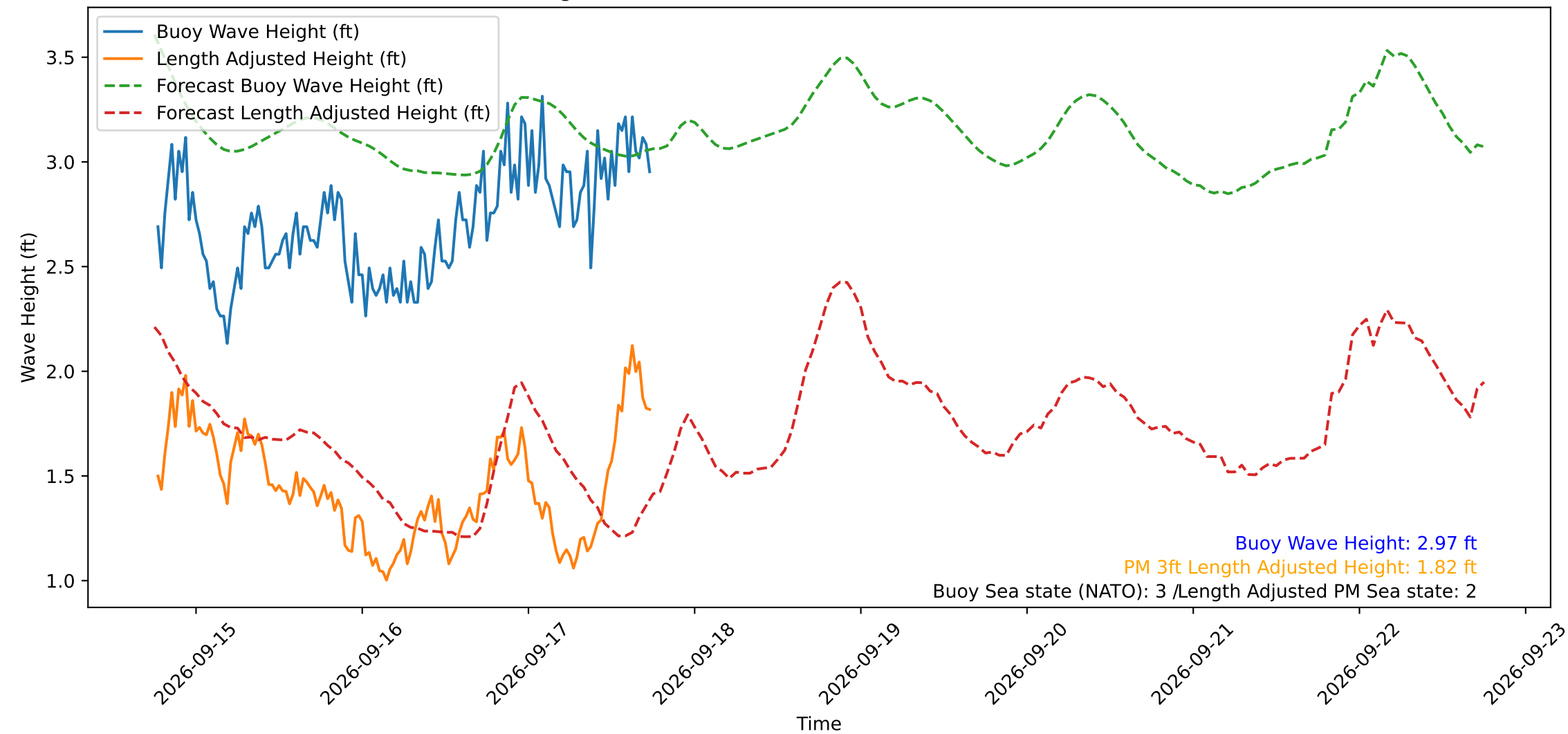
Wave Heights over Time for Green Beach at 2026-09-17 18:21:16
