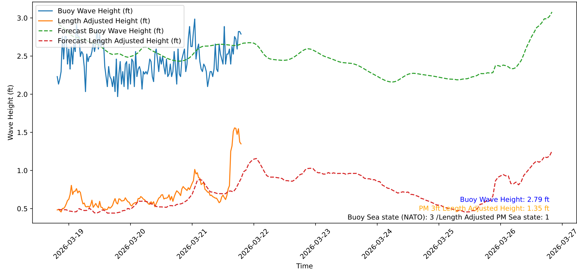
Wave Heights over Time for Oceanside Harbor at 2026-03-21 19:40:32
