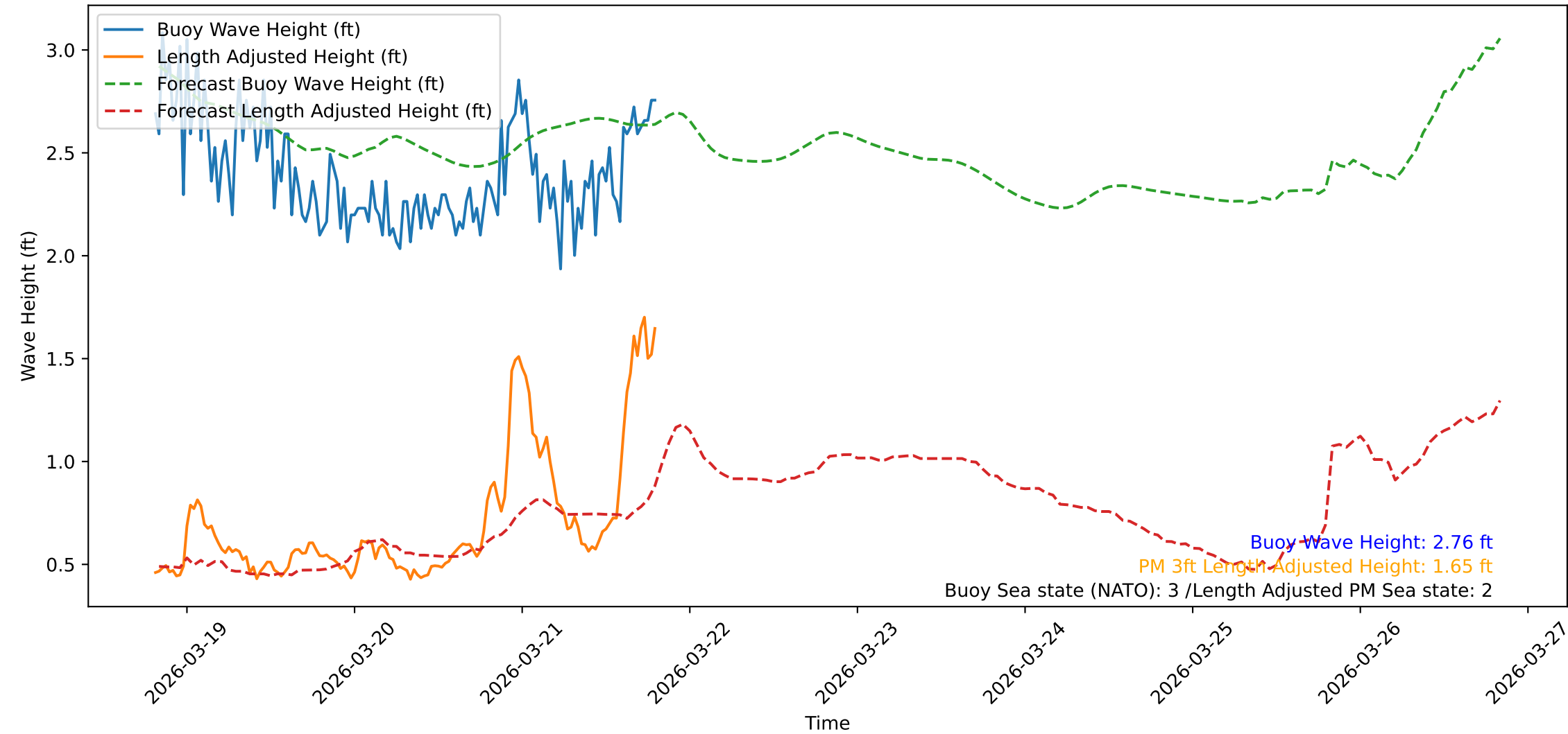
Wave Heights over Time for Green Beach at 2026-03-21 19:41:10
