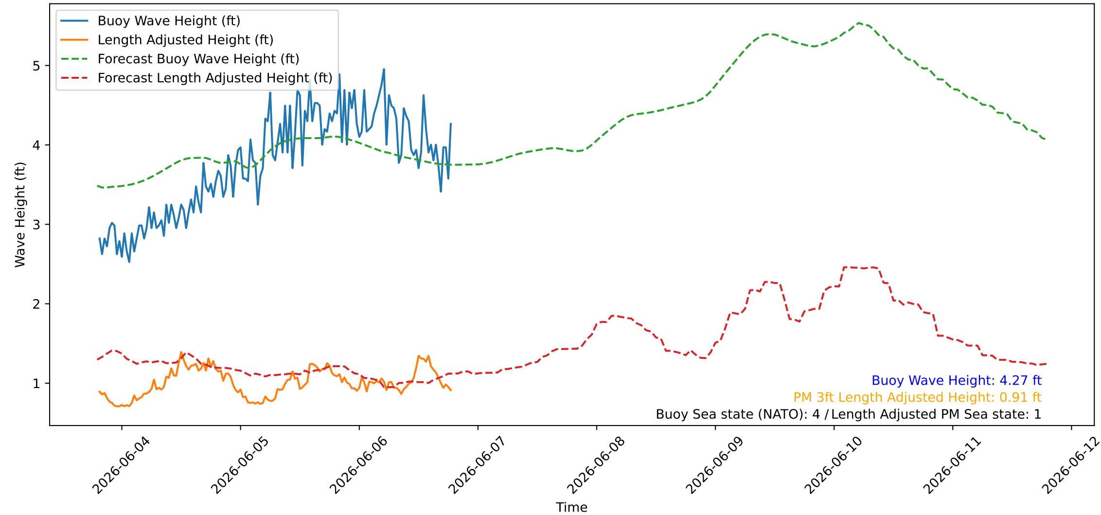
Wave Heights over Time for Red Beach at 2026-06-06 19:10:45
