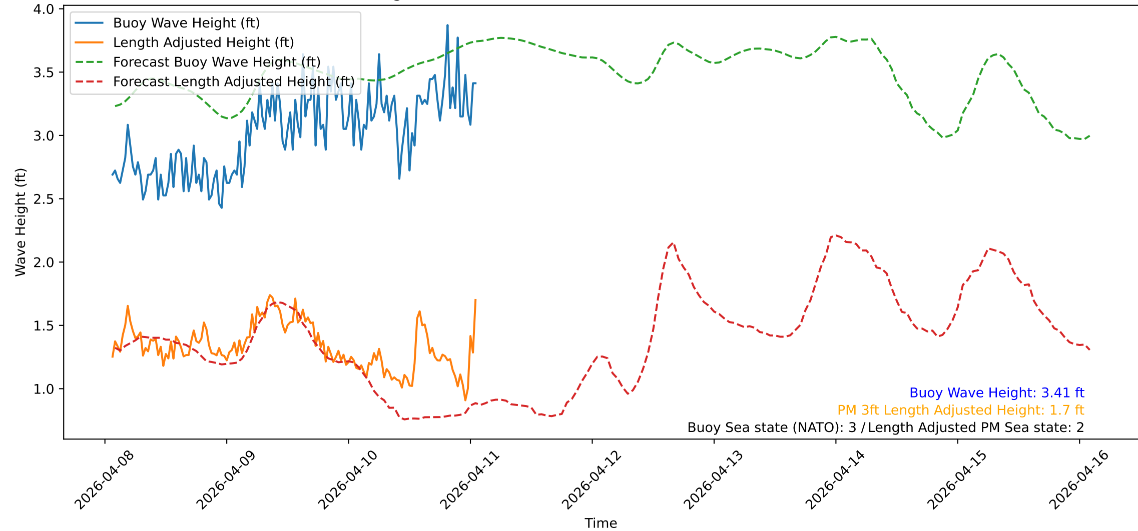
Wave Heights over Time for Oceanside Harbor at 2026-04-11 01:40:32
