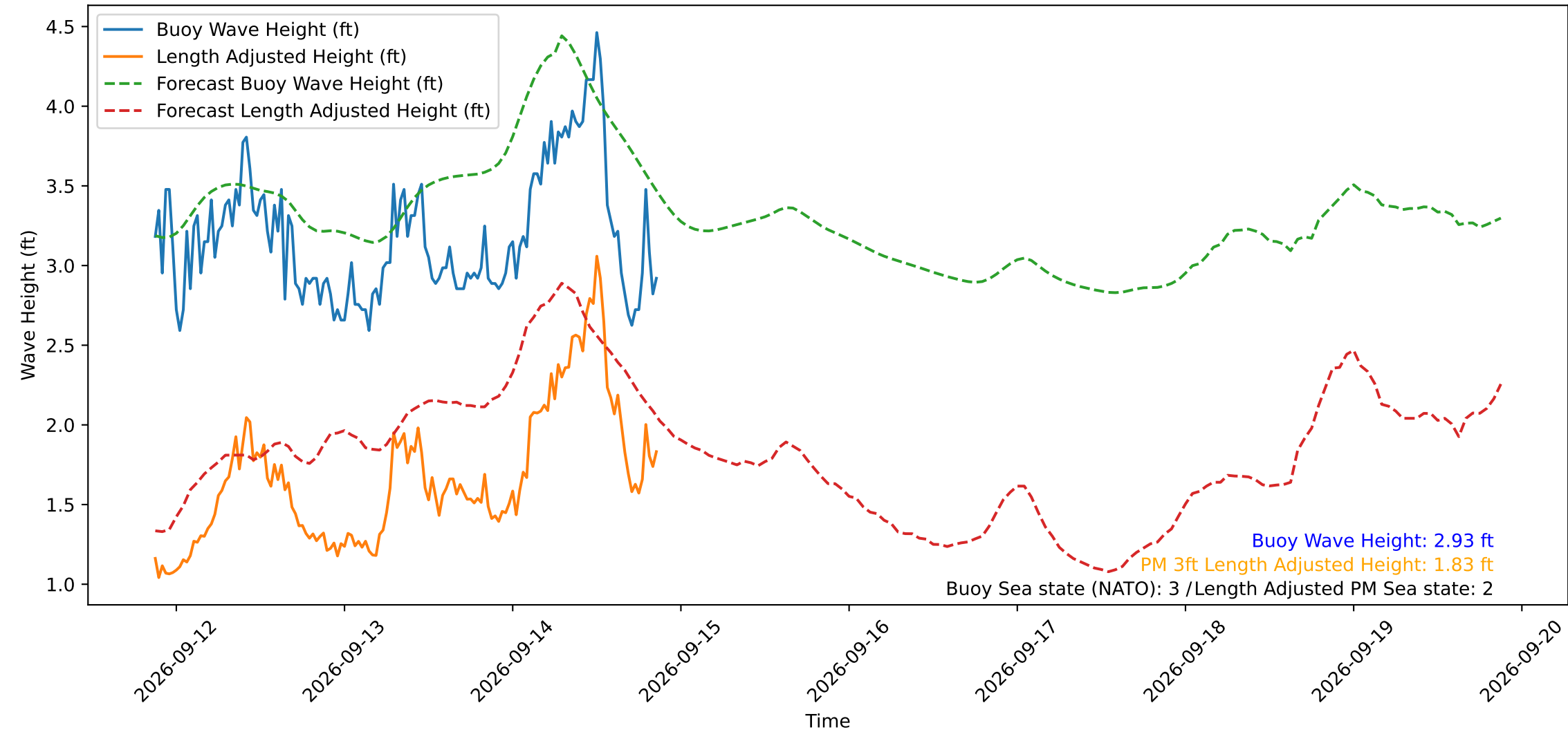
Wave Heights over Time for Oceanside Harbor at 2026-09-14 21:10:29
