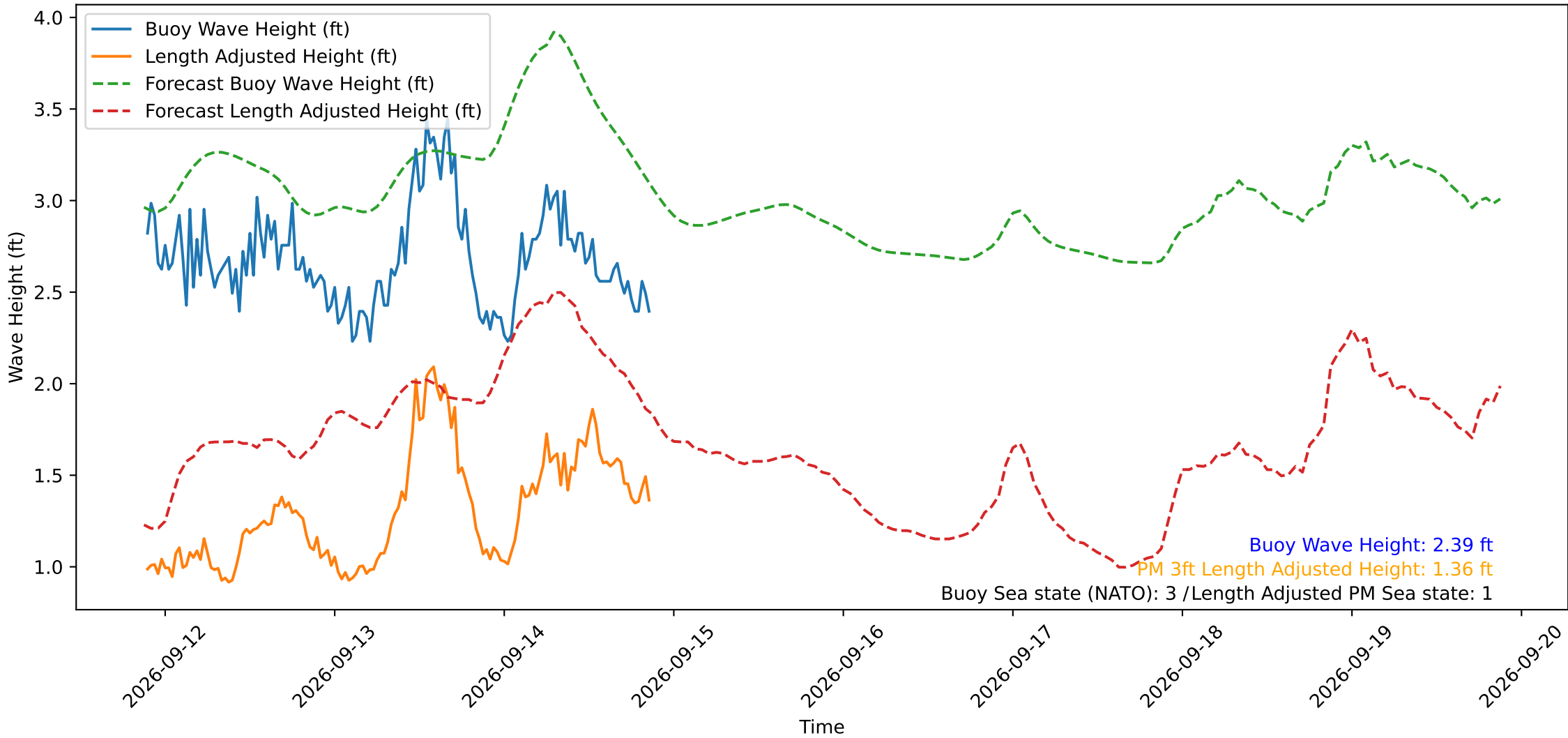
Wave Heights over Time for Red Beach at 2026-09-14 21:10:48
