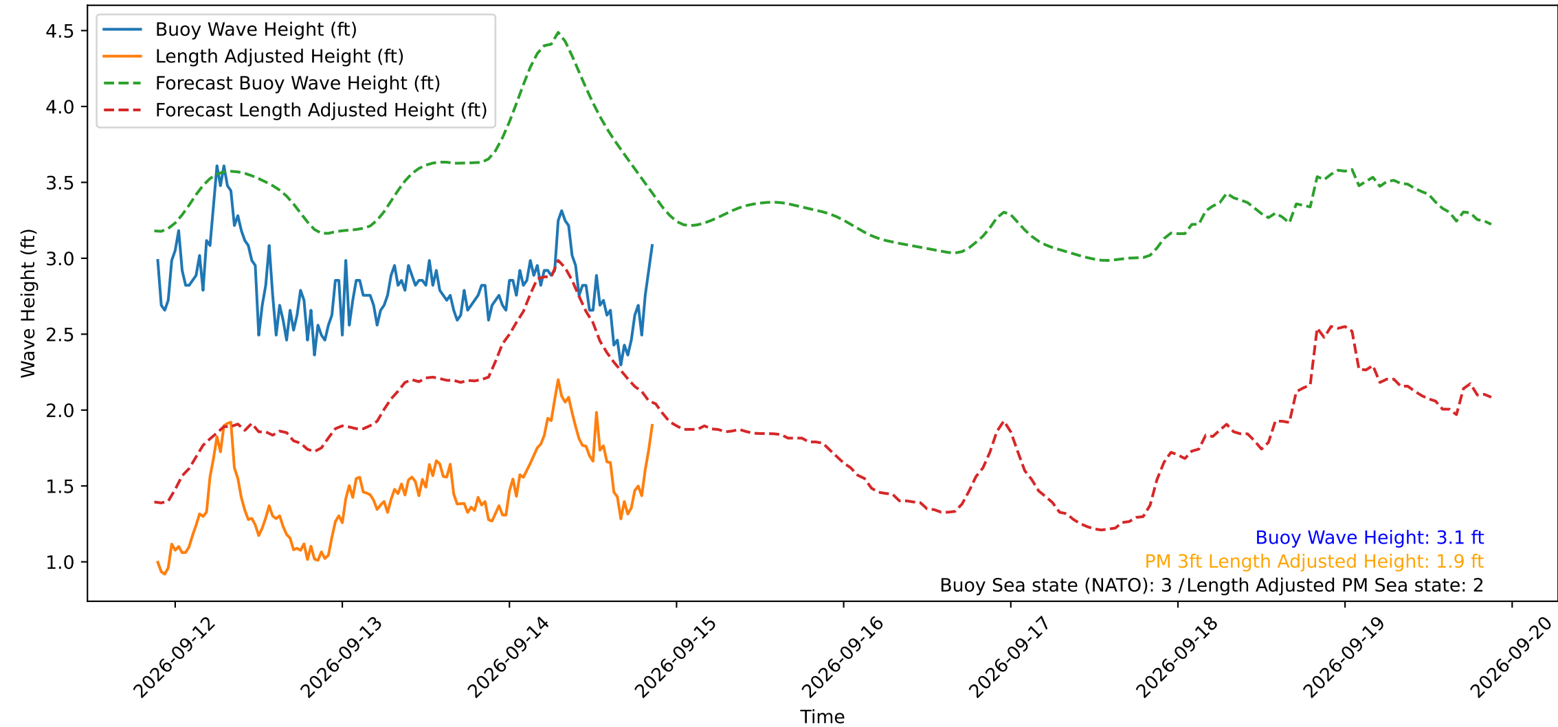
Wave Heights over Time for Green Beach at 2026-09-14 21:11:11
