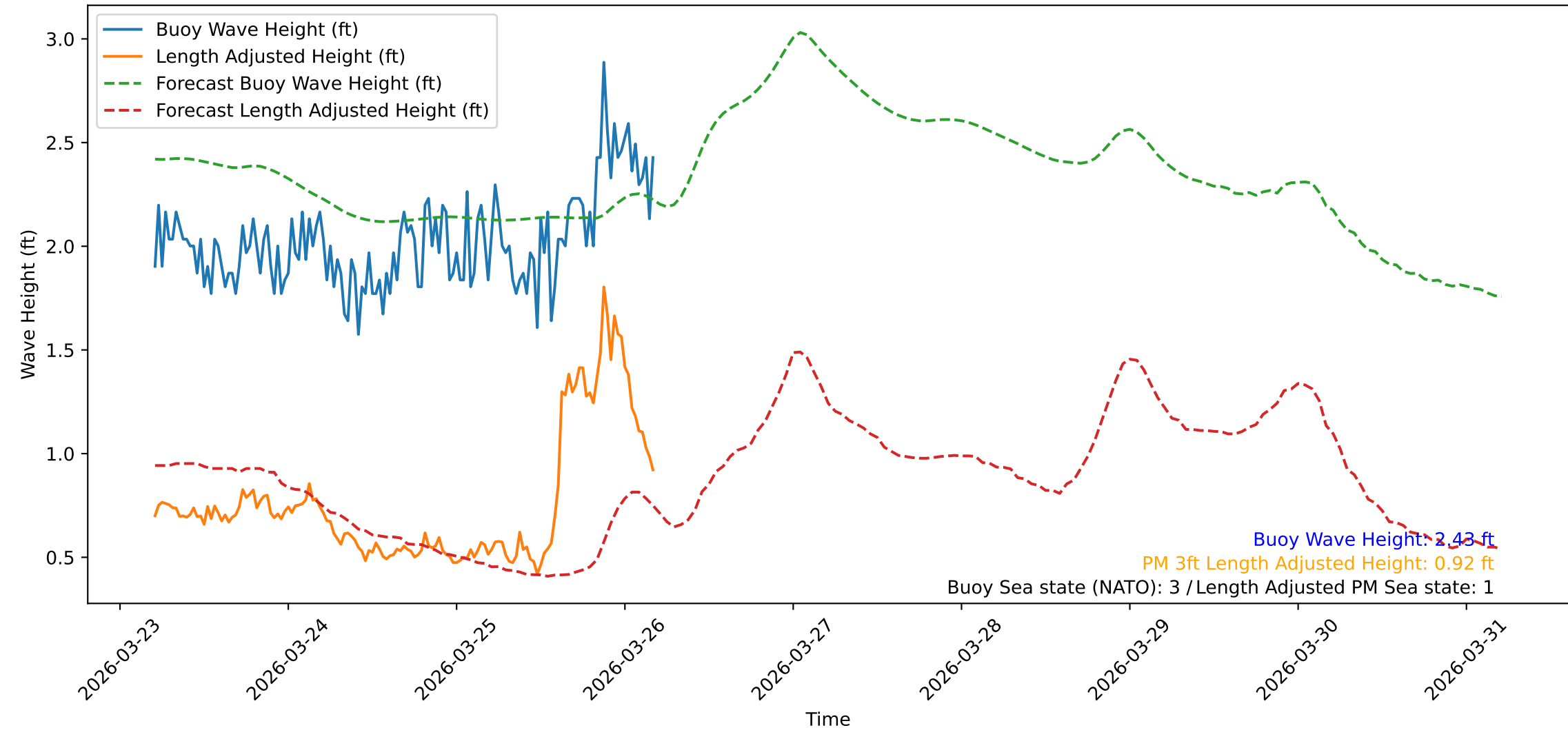
Wave Heights over Time for Oceanside Harbor at 2026-03-26 05:10:32
