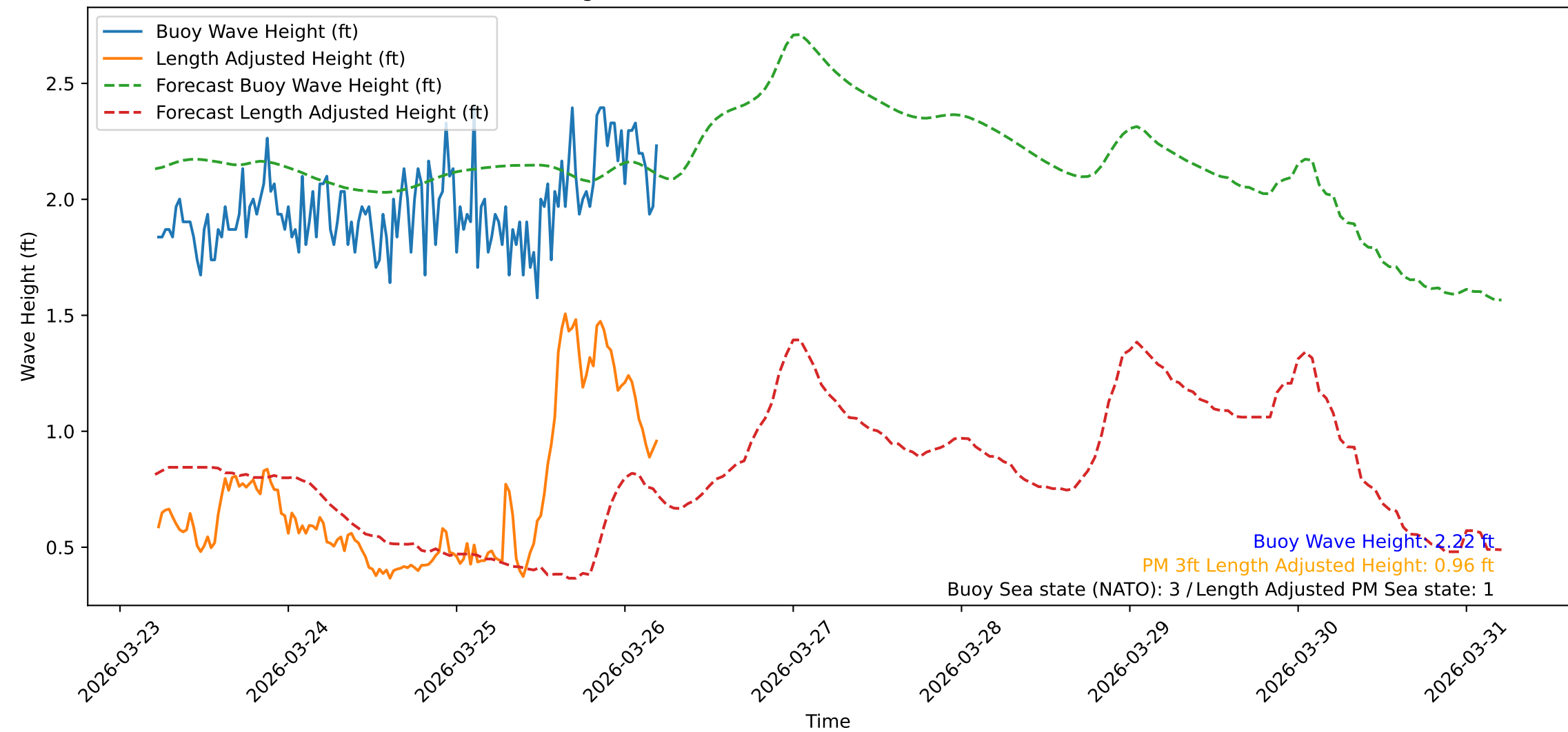
Wave Heights over Time for Red Beach at 2026-03-26 05:10:48
