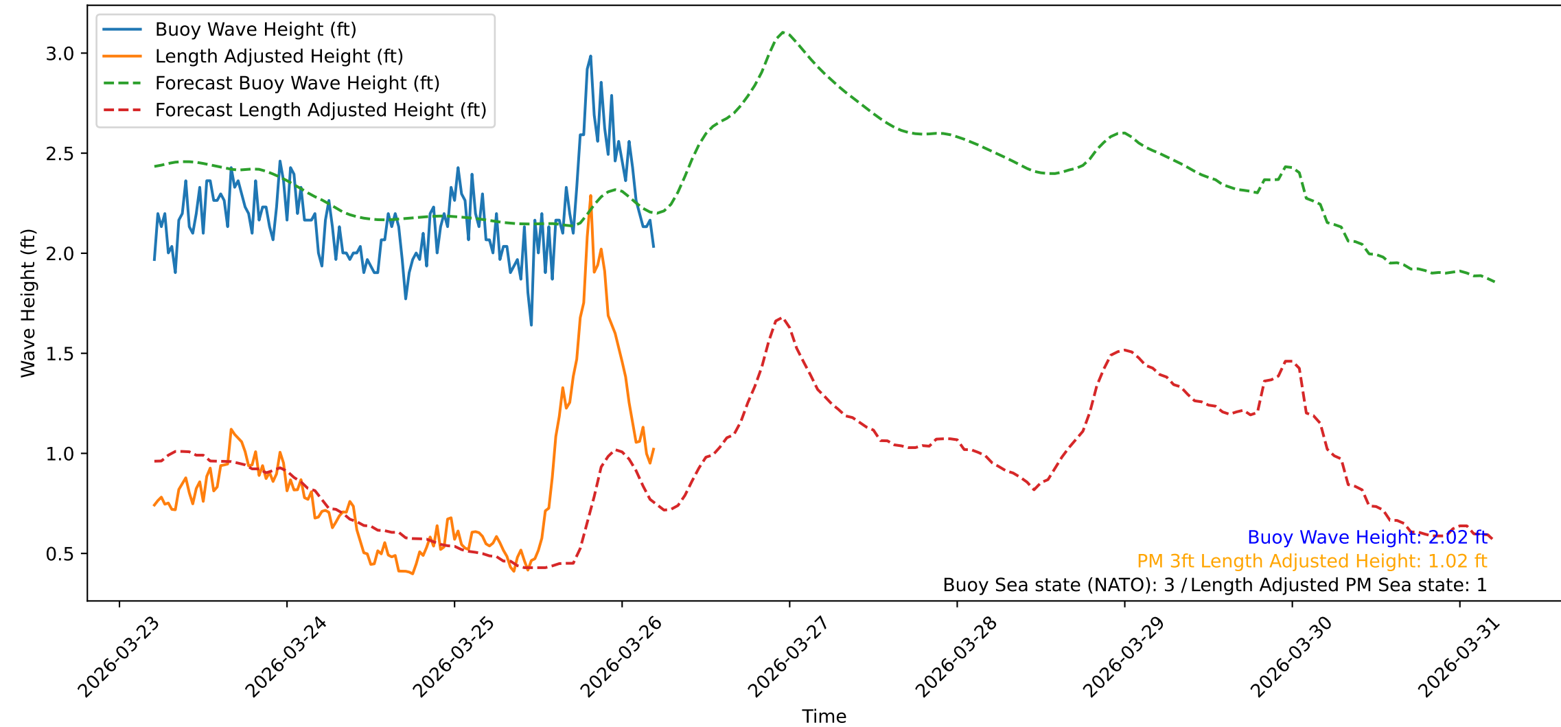
Wave Heights over Time for Green Beach at 2026-03-26 05:11:10
