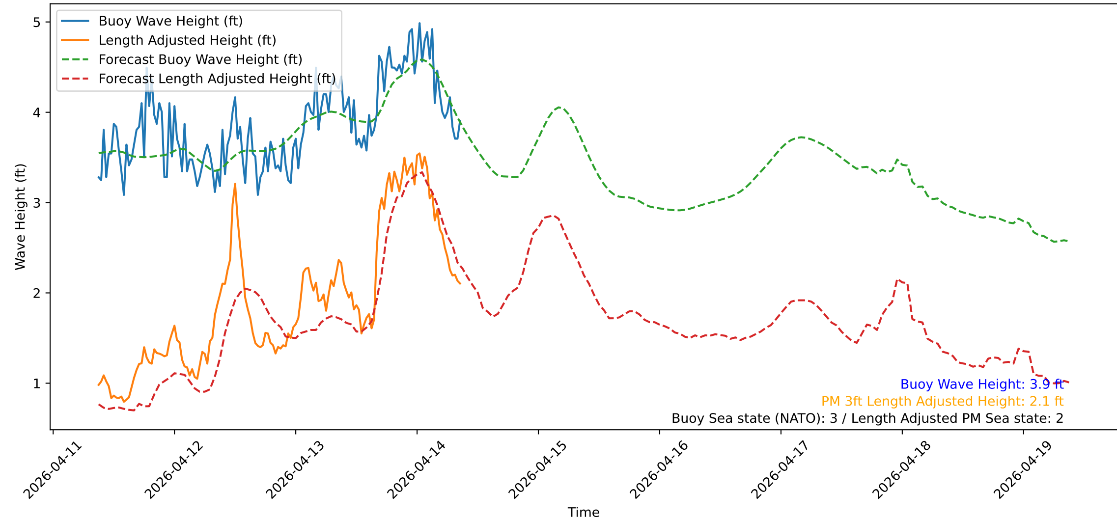
Wave Heights over Time for Green Beach at 2026-04-14 09:11:12
