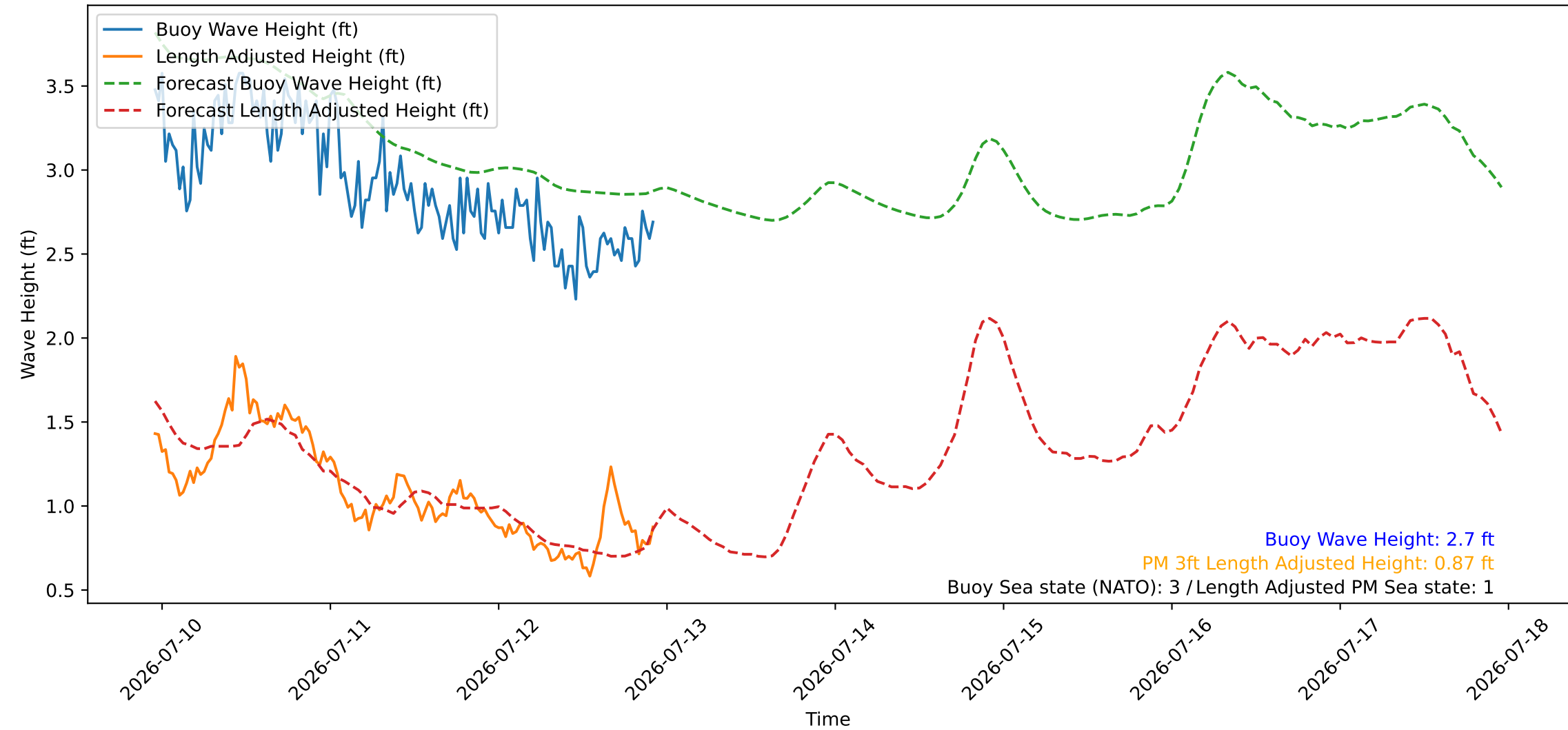
Wave Heights over Time for Green Beach at 2026-07-12 23:01:07
