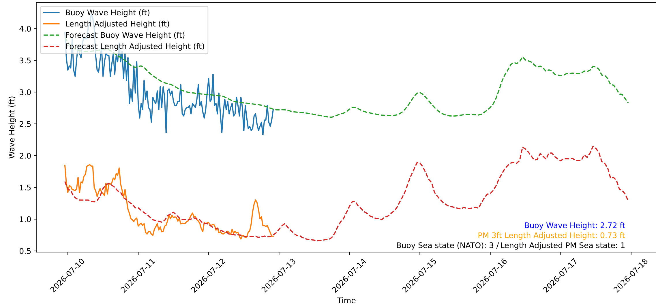
Wave Heights over Time for Oceanside Harbor at 2026-07-12 23:00:26
