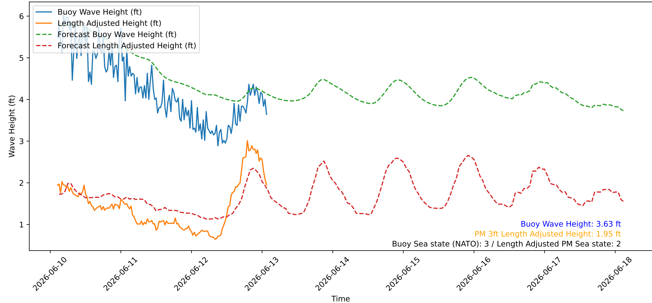
Wave Heights over Time for Green Beach at 2026-06-13 02:31:09
