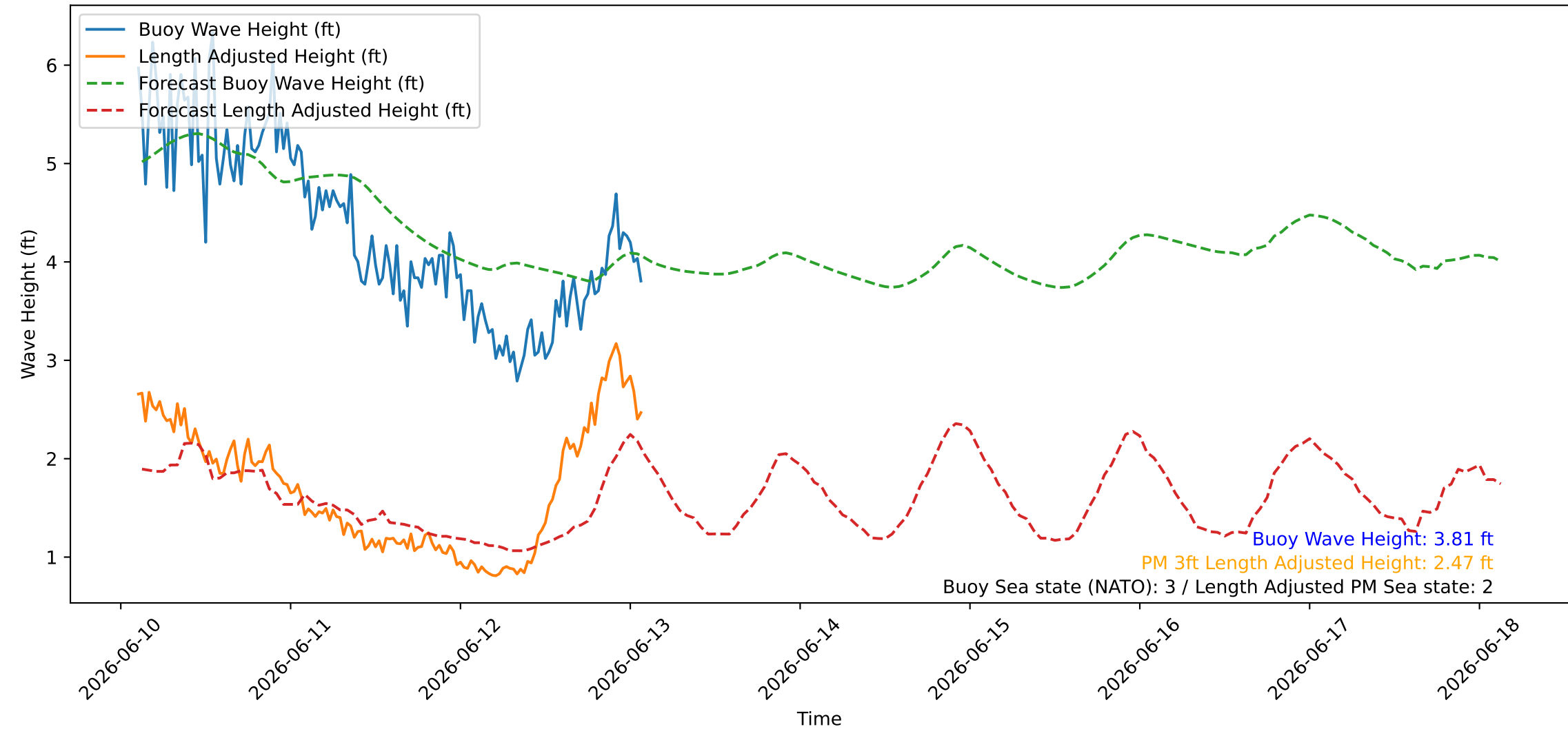
Wave Heights over Time for Oceanside Harbor at 2026-06-13 02:30:27
