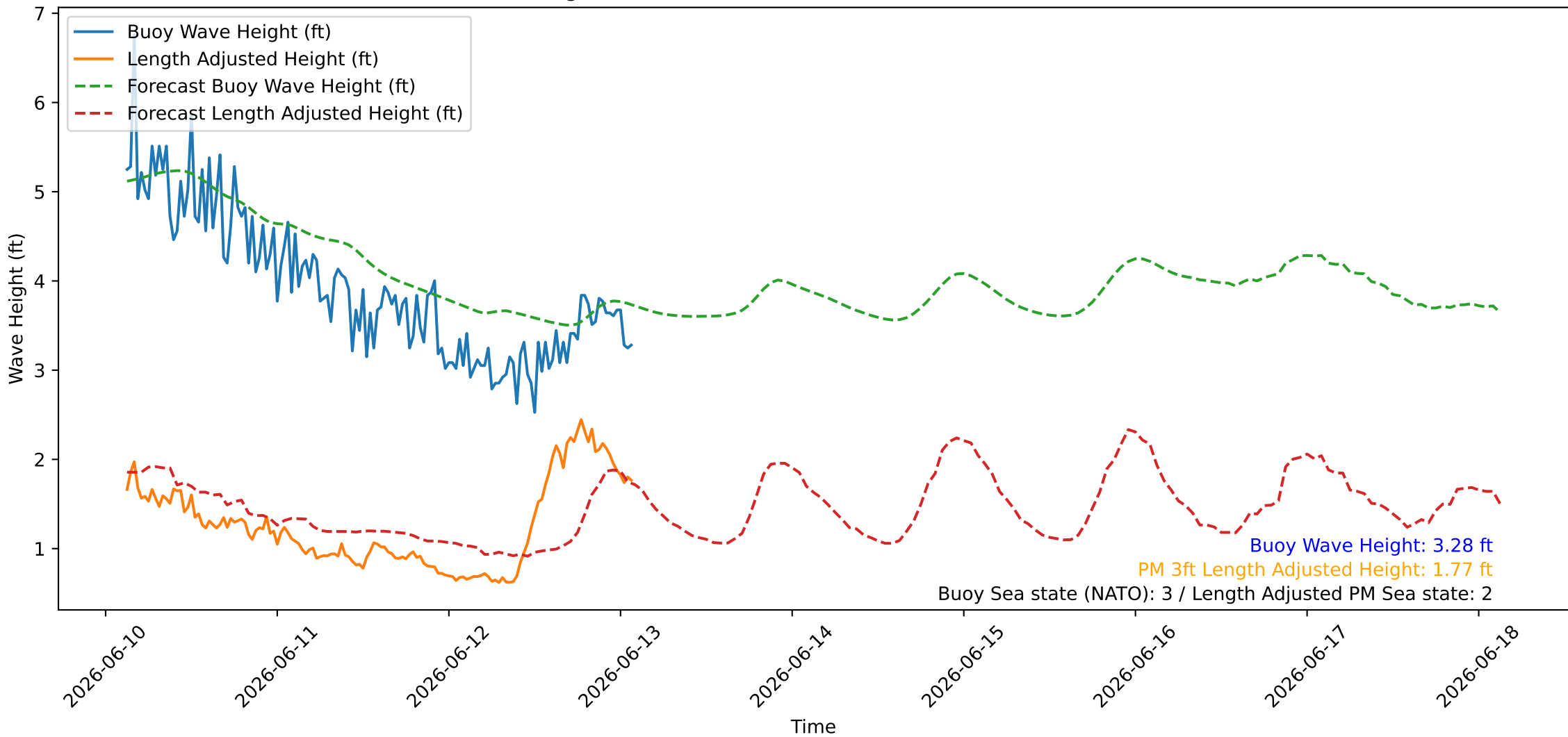
Wave Heights over Time for Red Beach at 2026-06-13 02:30:46
