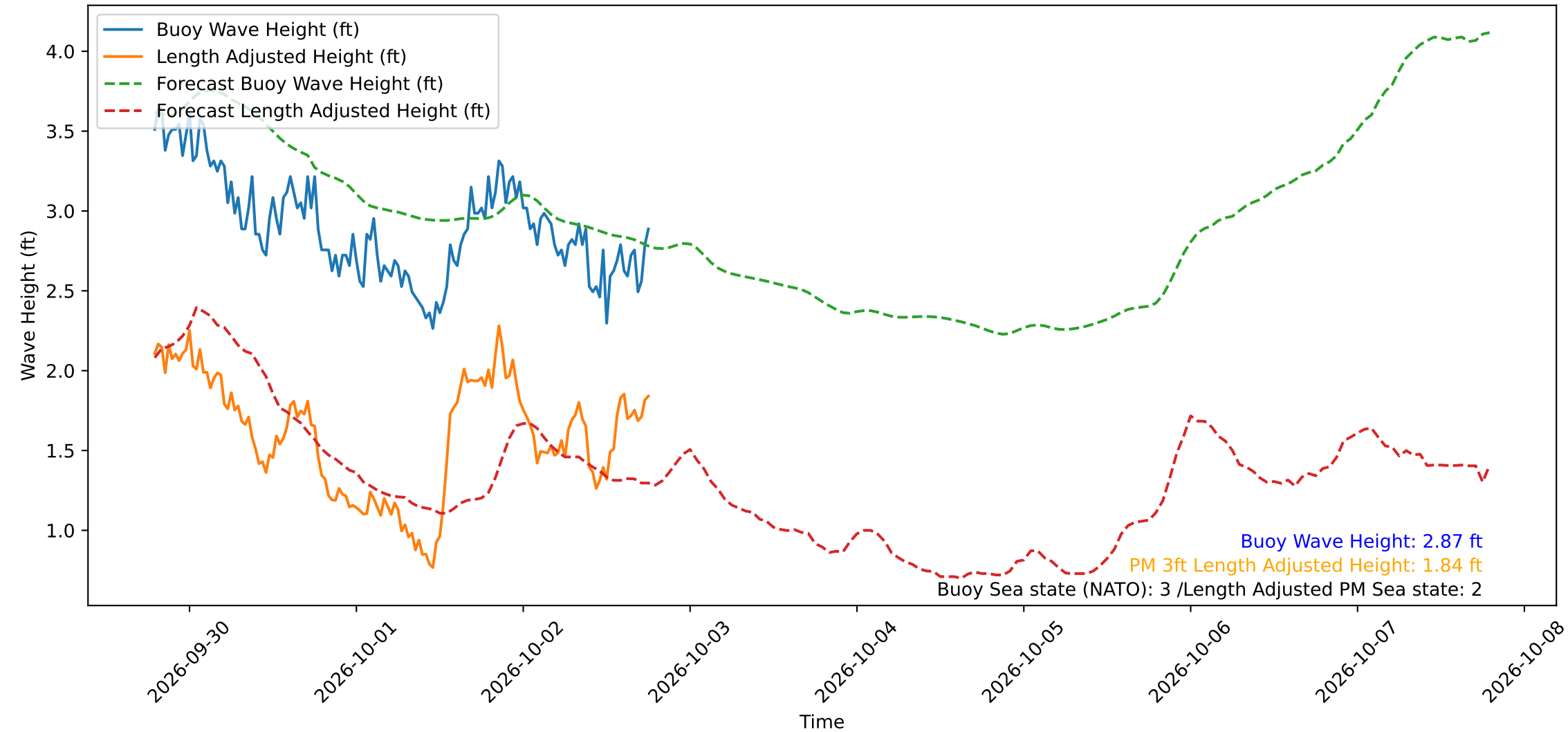
Wave Heights over Time for Oceanside Harbor at 2026-10-02 18:50:29
