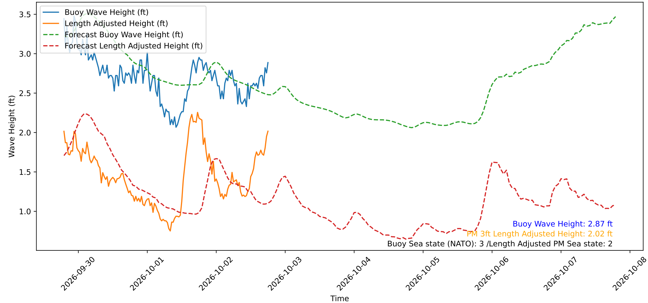
Wave Heights over Time for Red Beach at 2026-10-02 18:50:50
