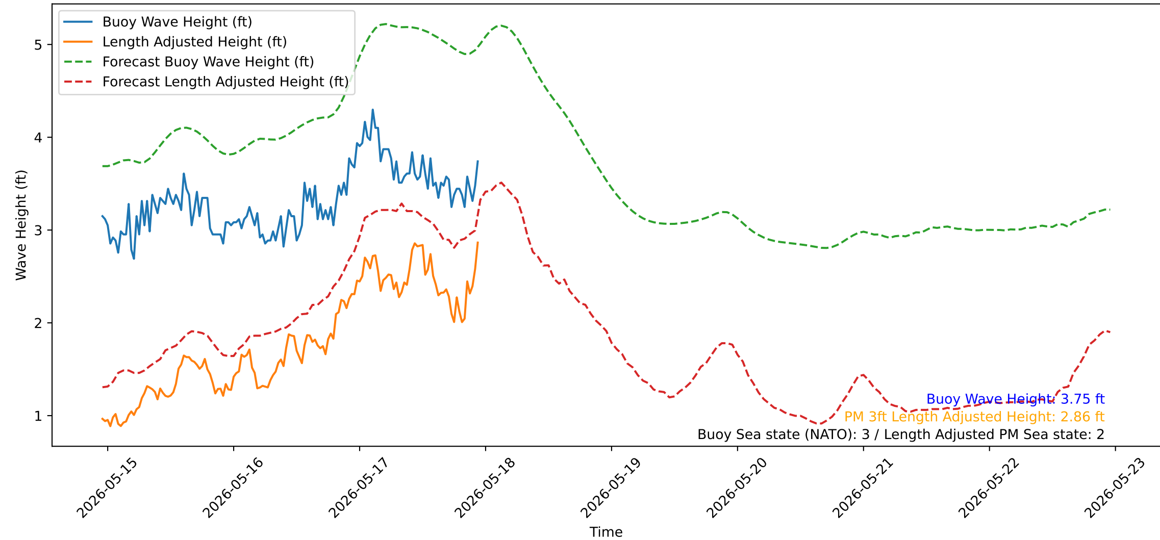
Wave Heights over Time for Oceanside Harbor at 2026-05-17 23:10:32
