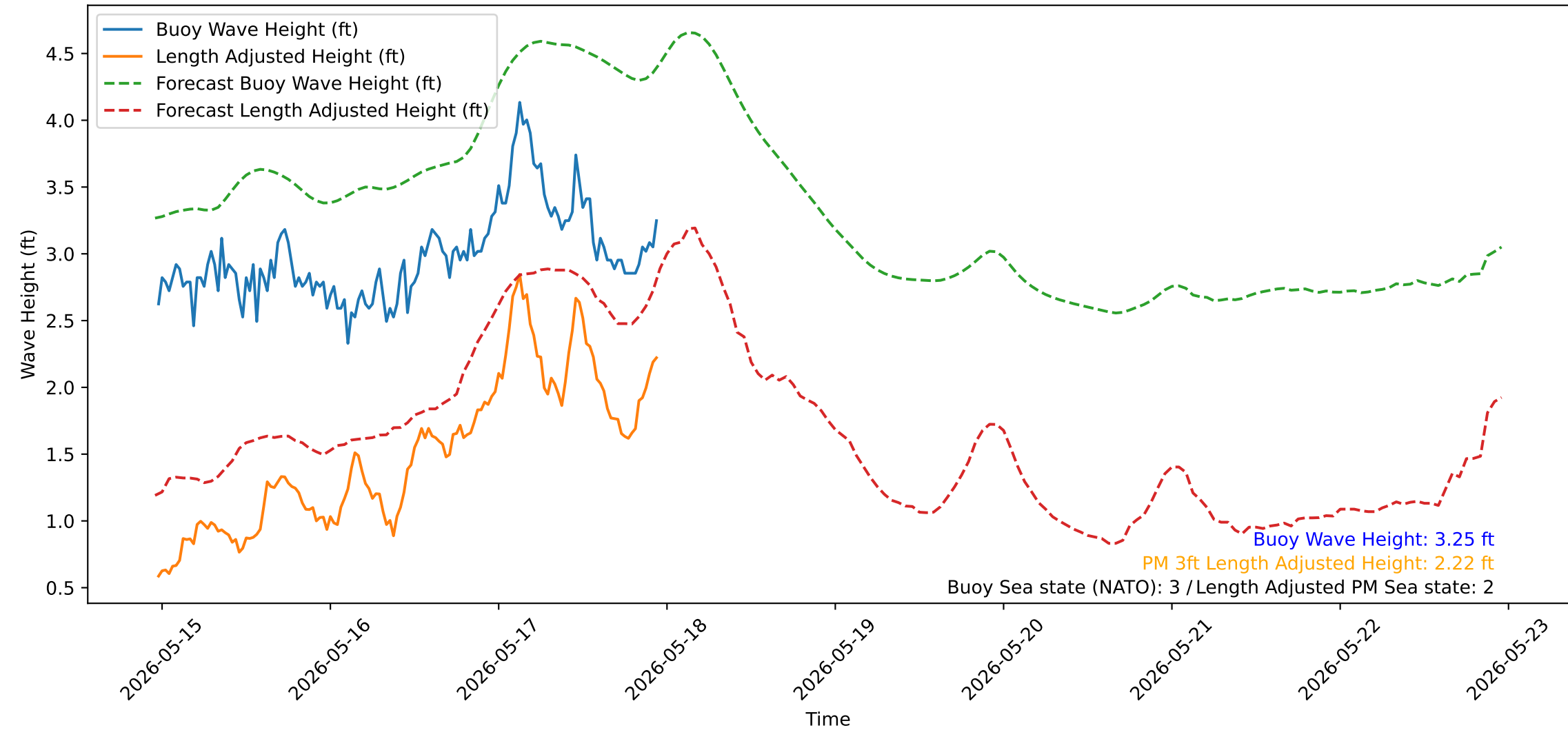
Wave Heights over Time for Red Beach at 2026-05-17 23:10:51
