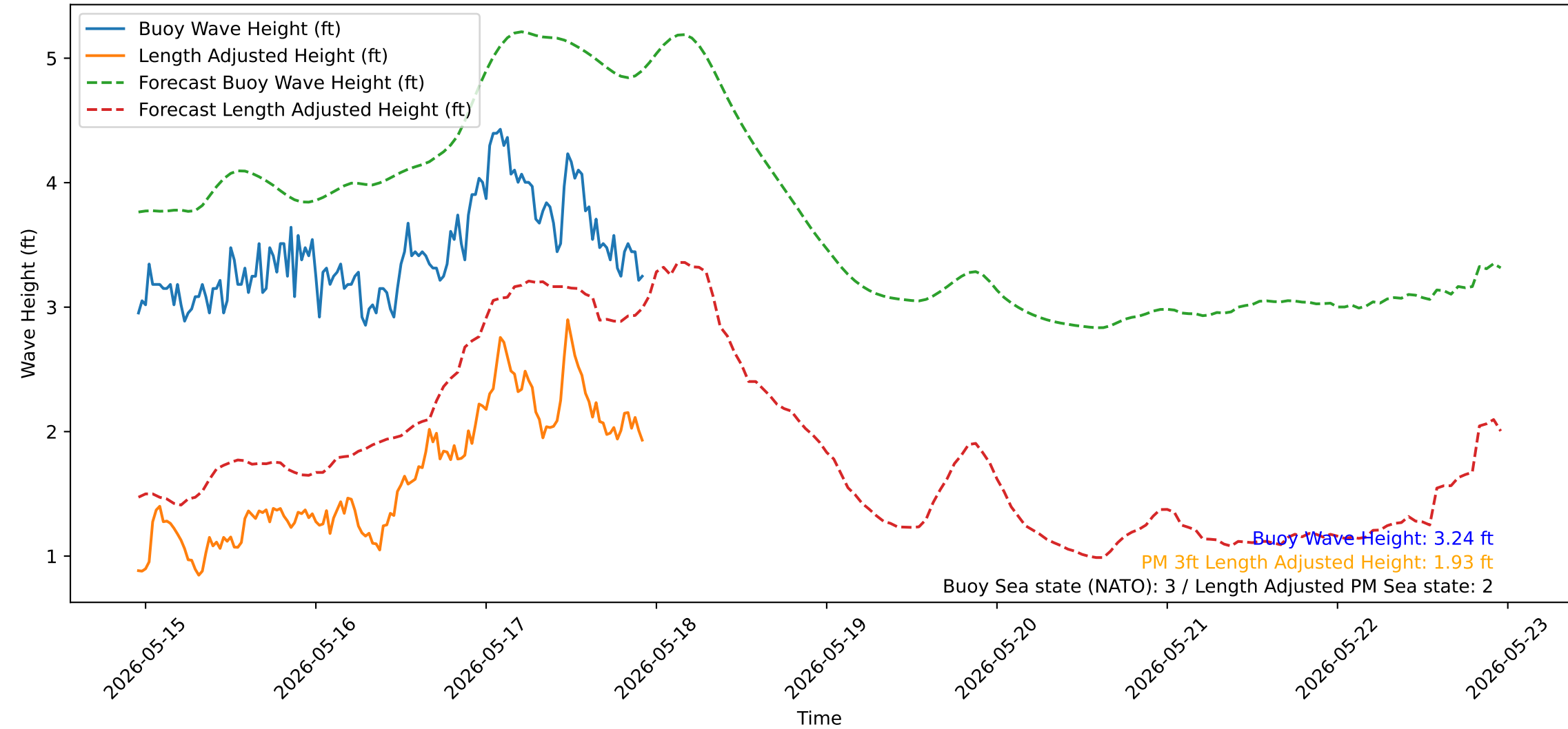
Wave Heights over Time for Green Beach at 2026-05-17 23:11:14
