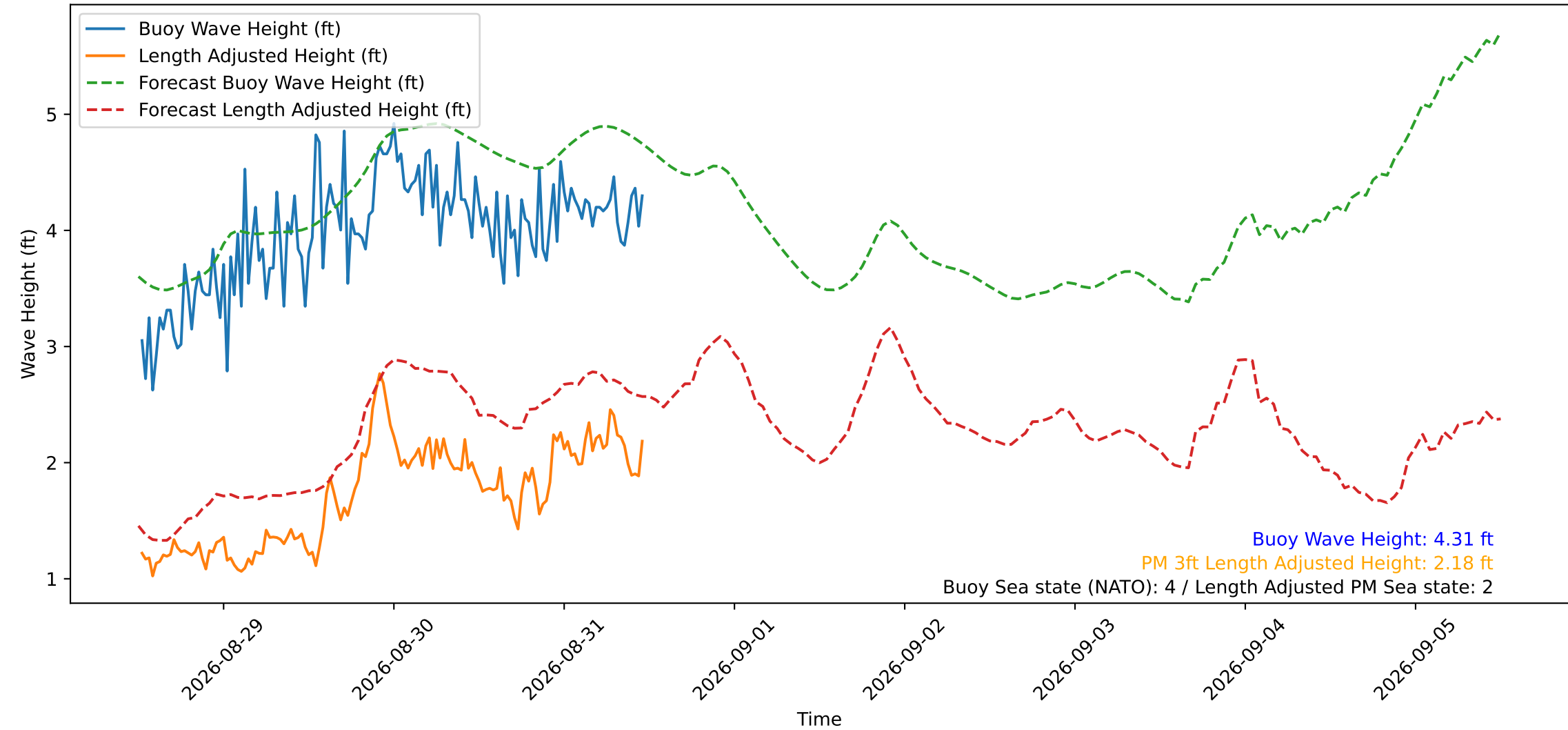
Wave Heights over Time for Green Beach at 2026-08-31 12:01:11
