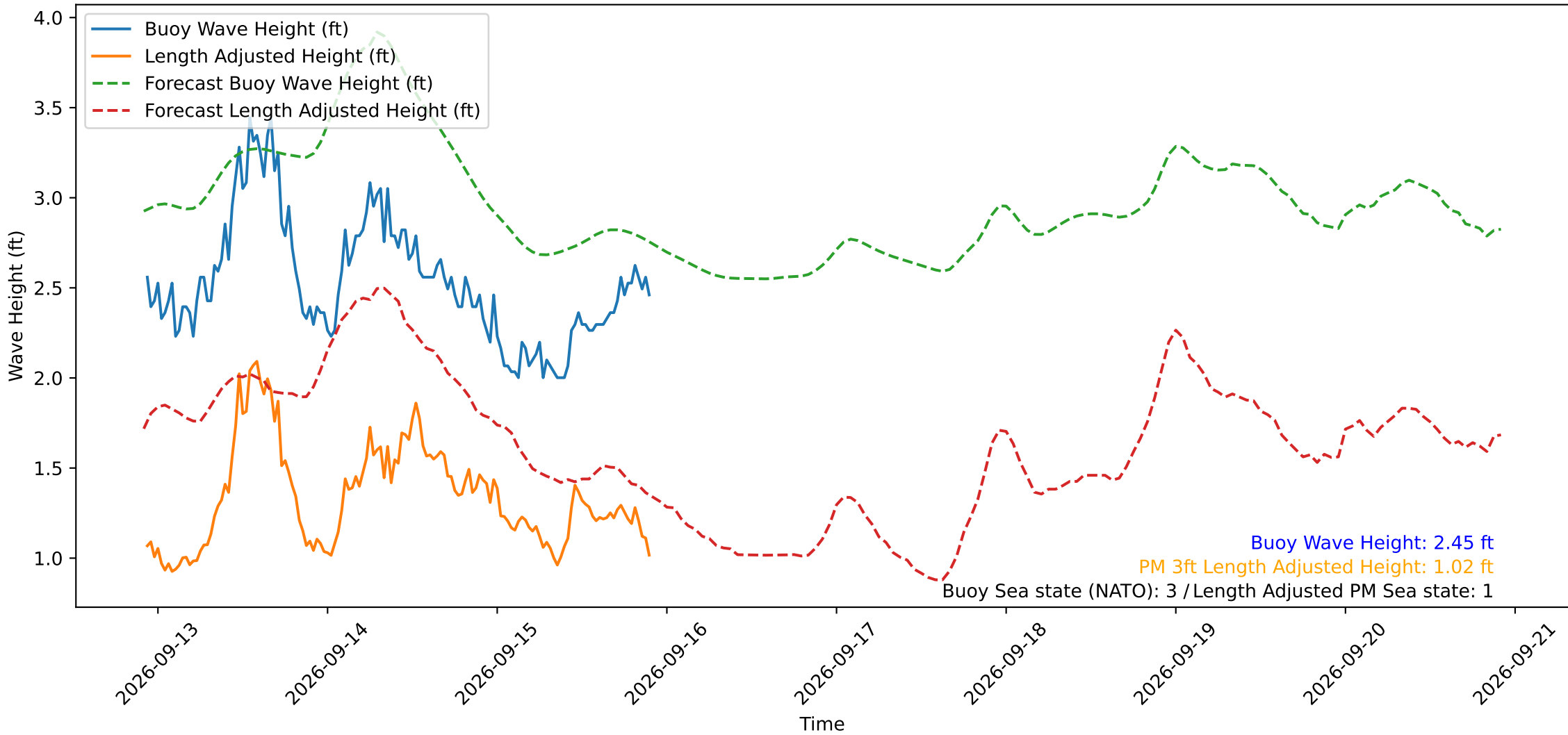
Wave Heights over Time for Red Beach at 2026-09-15 22:10:49
