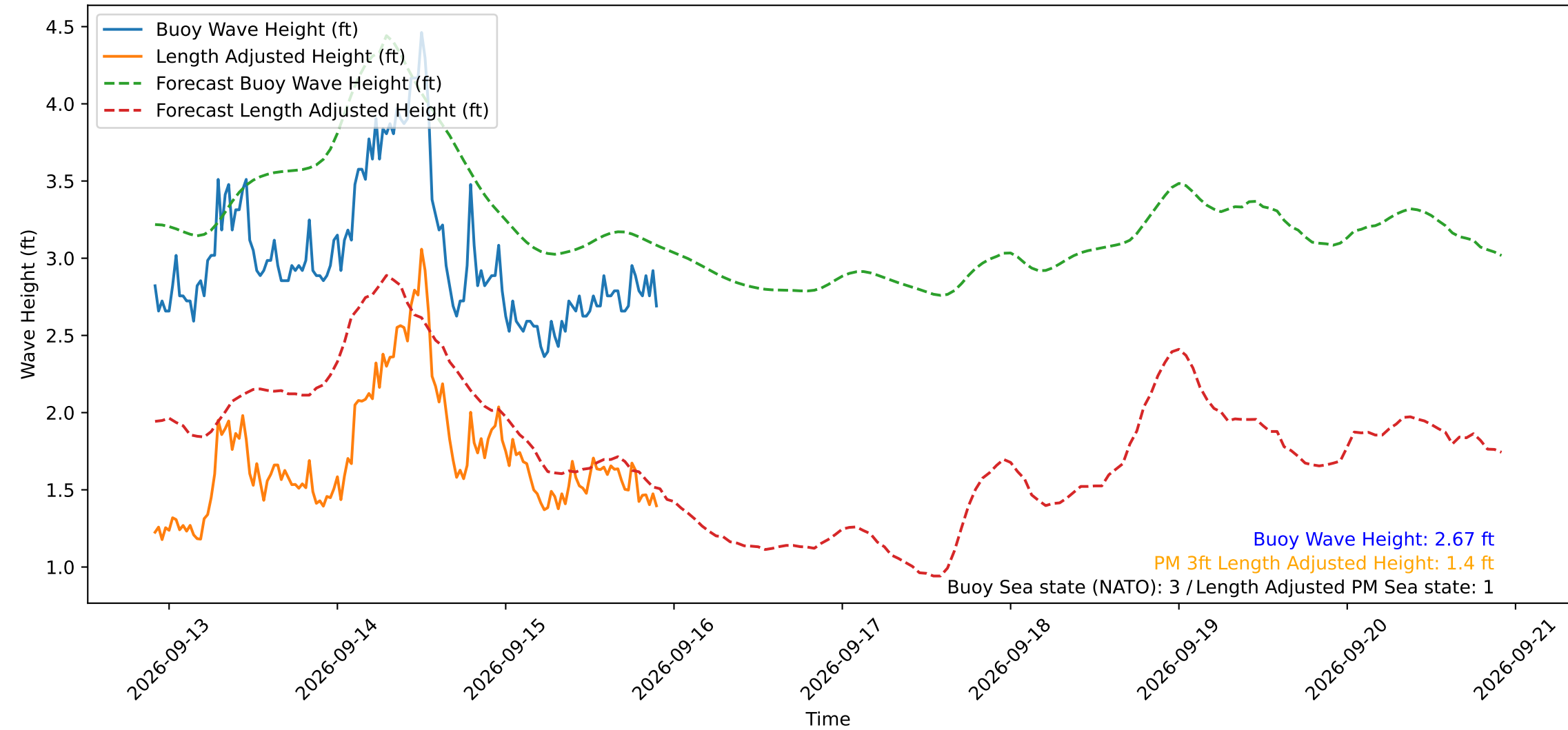
Wave Heights over Time for Oceanside Harbor at 2026-09-15 22:10:29
