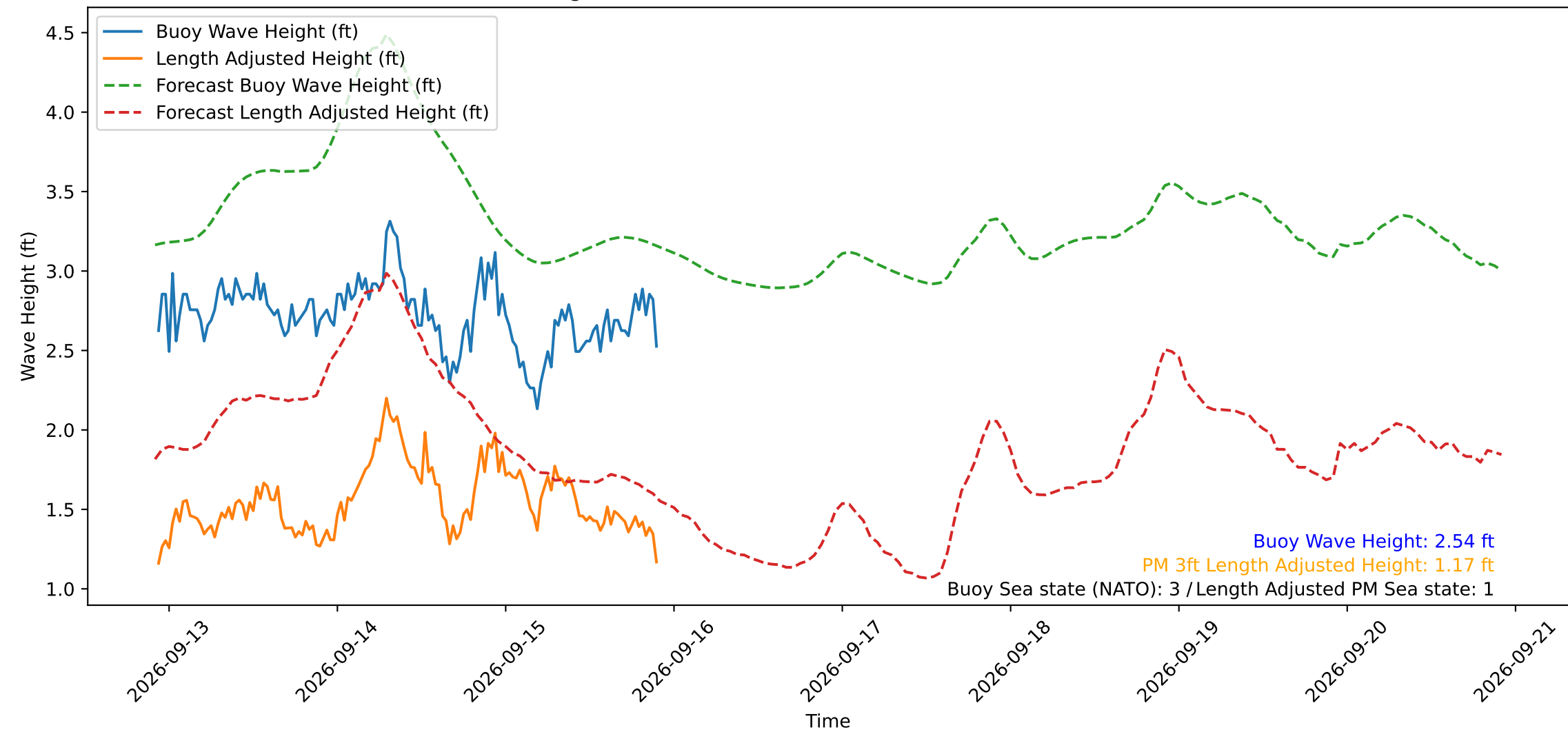
Wave Heights over Time for Green Beach at 2026-09-15 22:11:12
