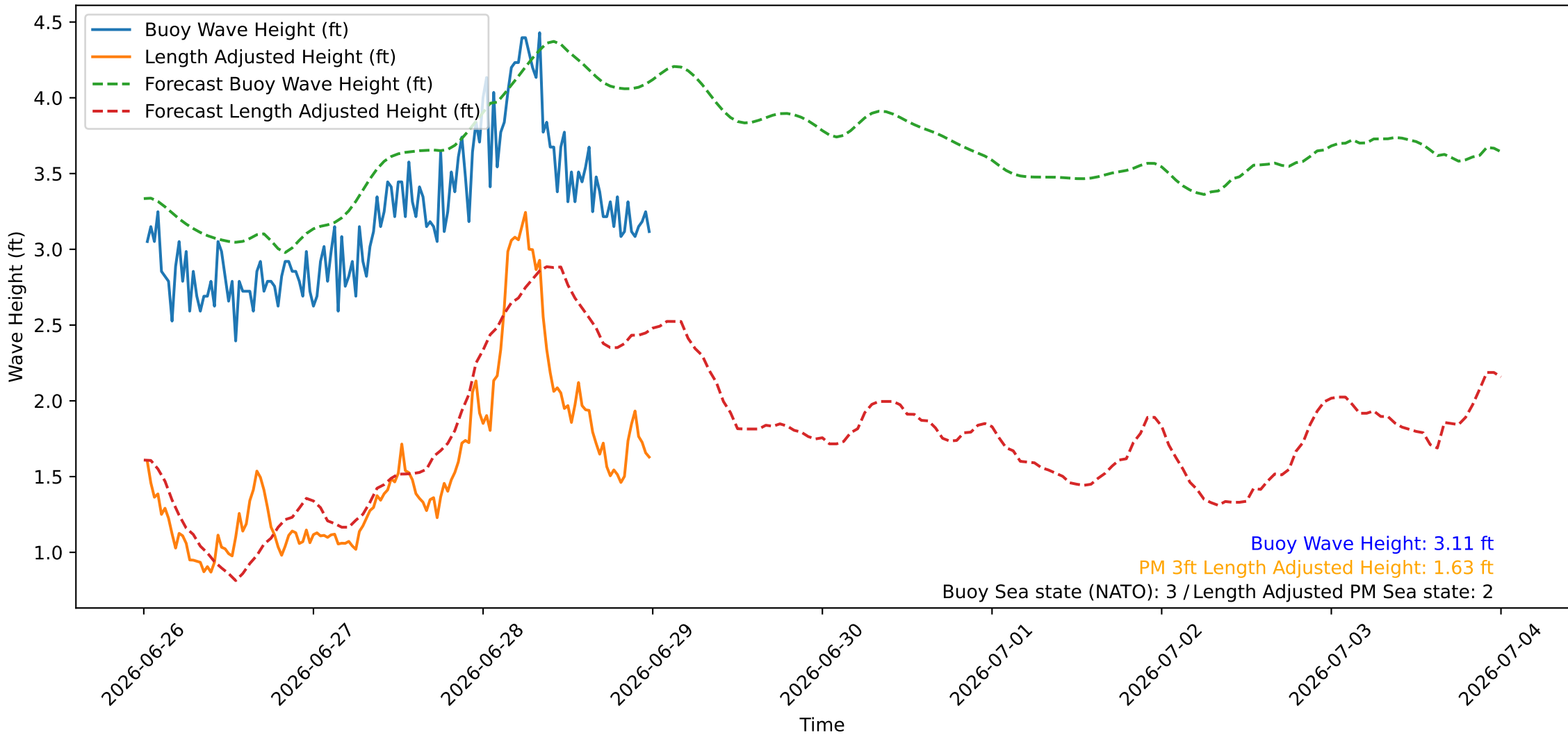
Wave Heights over Time for Oceanside Harbor at 2026-06-29 00:20:25
