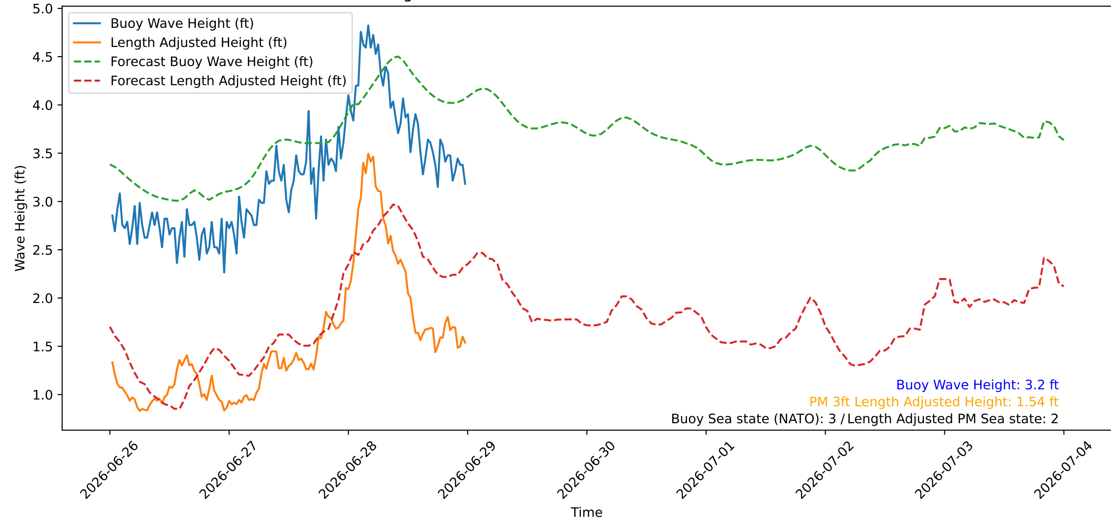
Wave Heights over Time for Green Beach at 2026-06-29 00:21:08
