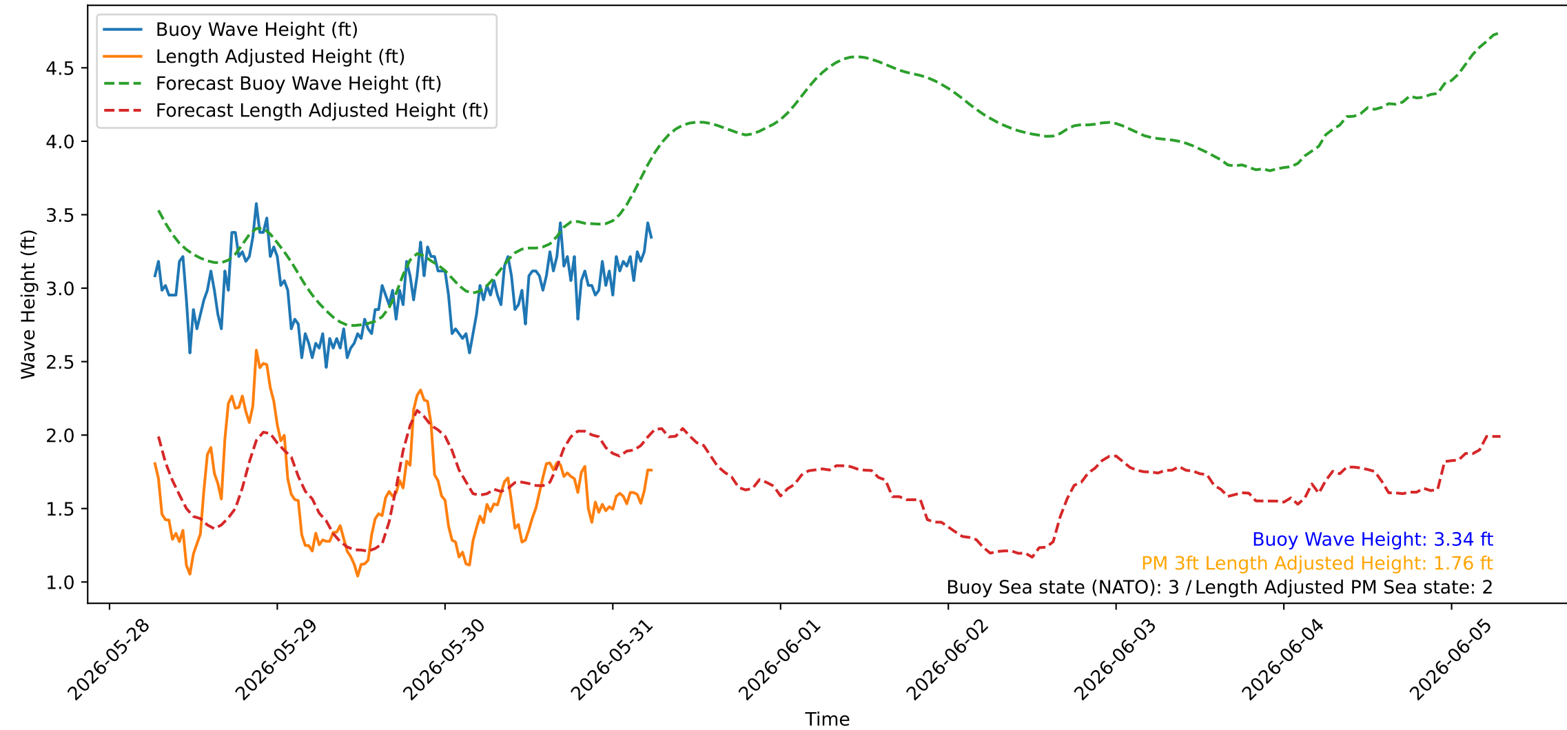
Wave Heights over Time for Green Beach at 2026-05-31 06:31:06
