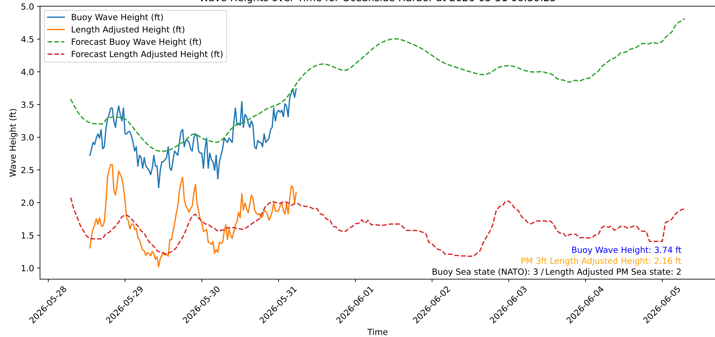
Wave Heights over Time for Oceanside Harbor at 2026-05-31 06:30:25
