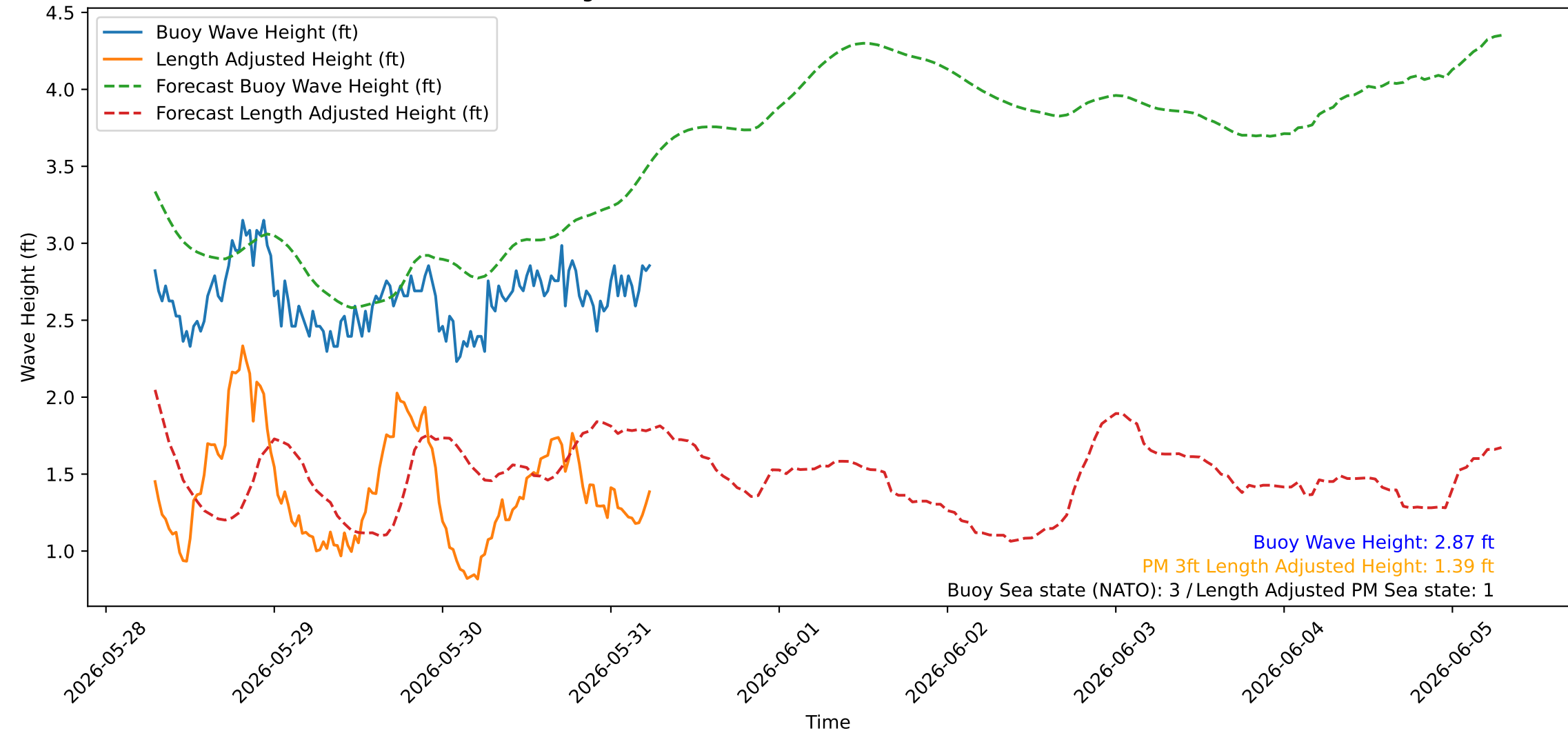
Wave Heights over Time for Red Beach at 2026-05-31 06:30:44
