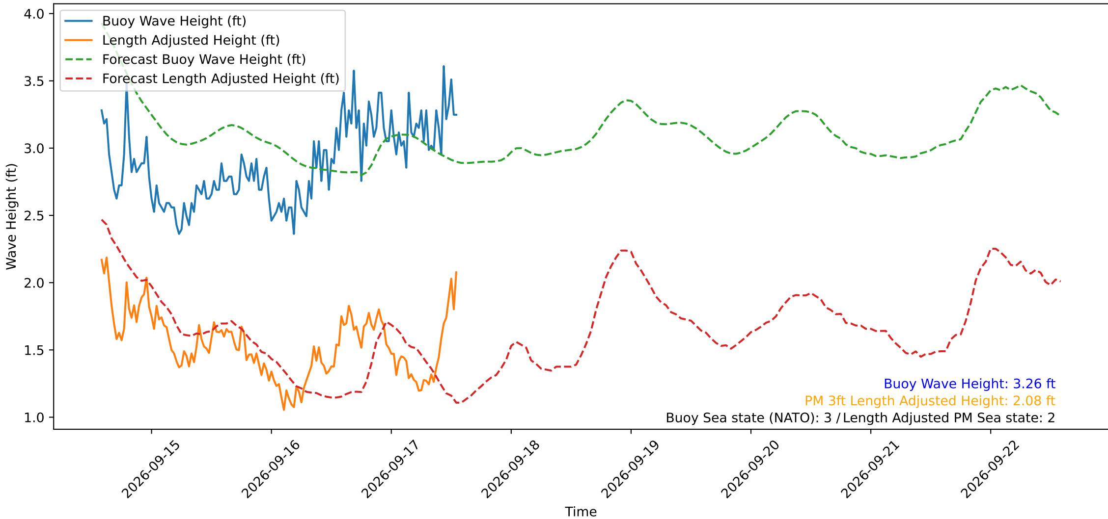
Wave Heights over Time for Oceanside Harbor at 2026-09-17 14:00:29
