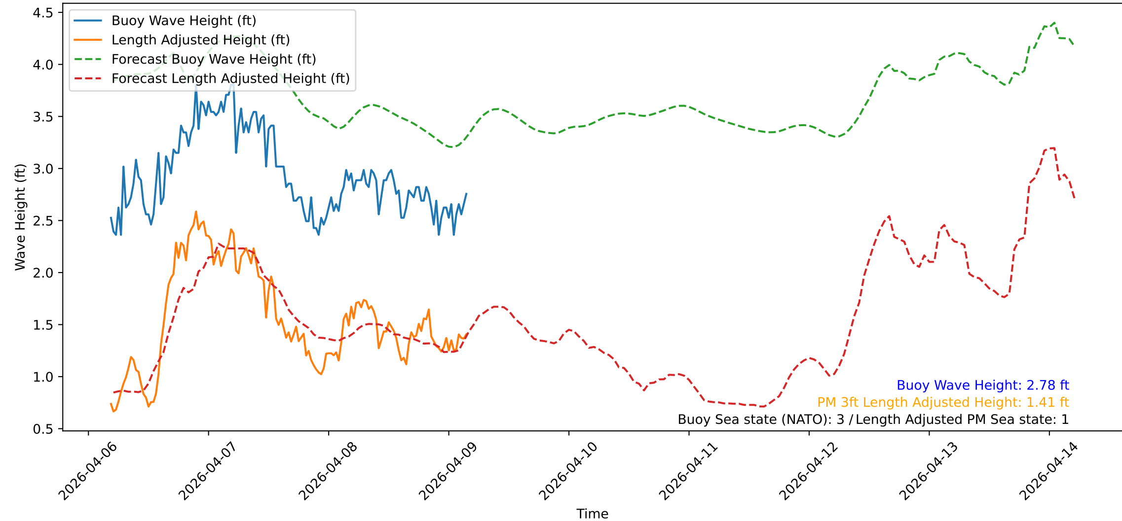
Wave Heights over Time for Green Beach at 2026-04-09 04:31:10
