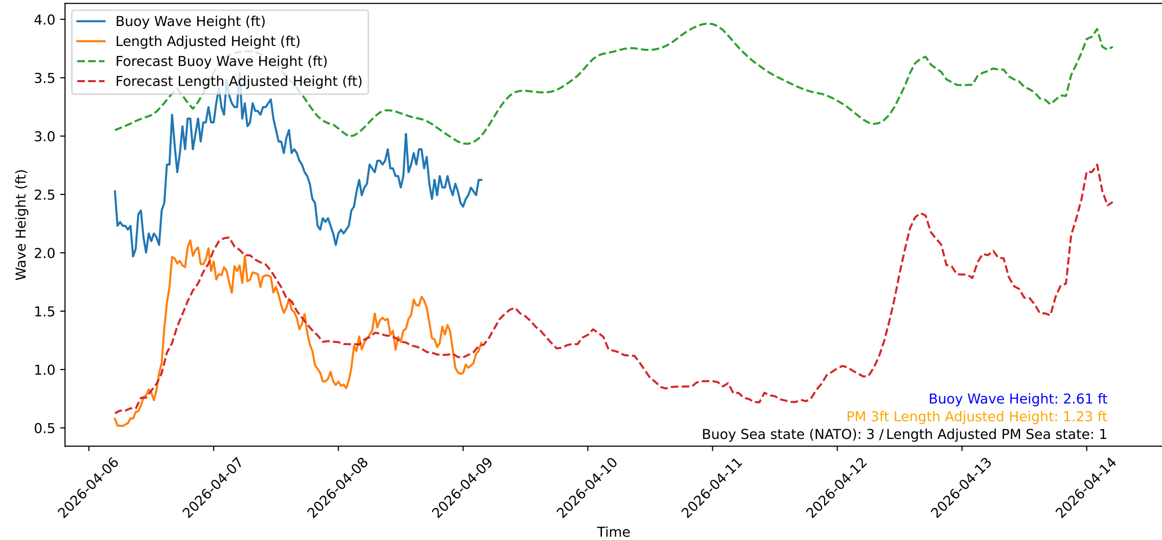
Wave Heights over Time for Red Beach at 2026-04-09 04:30:47
