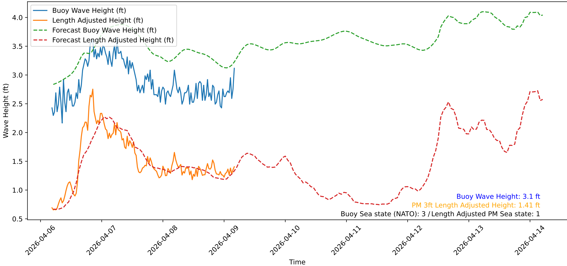
Wave Heights over Time for Oceanside Harbor at 2026-04-09 04:30:31
