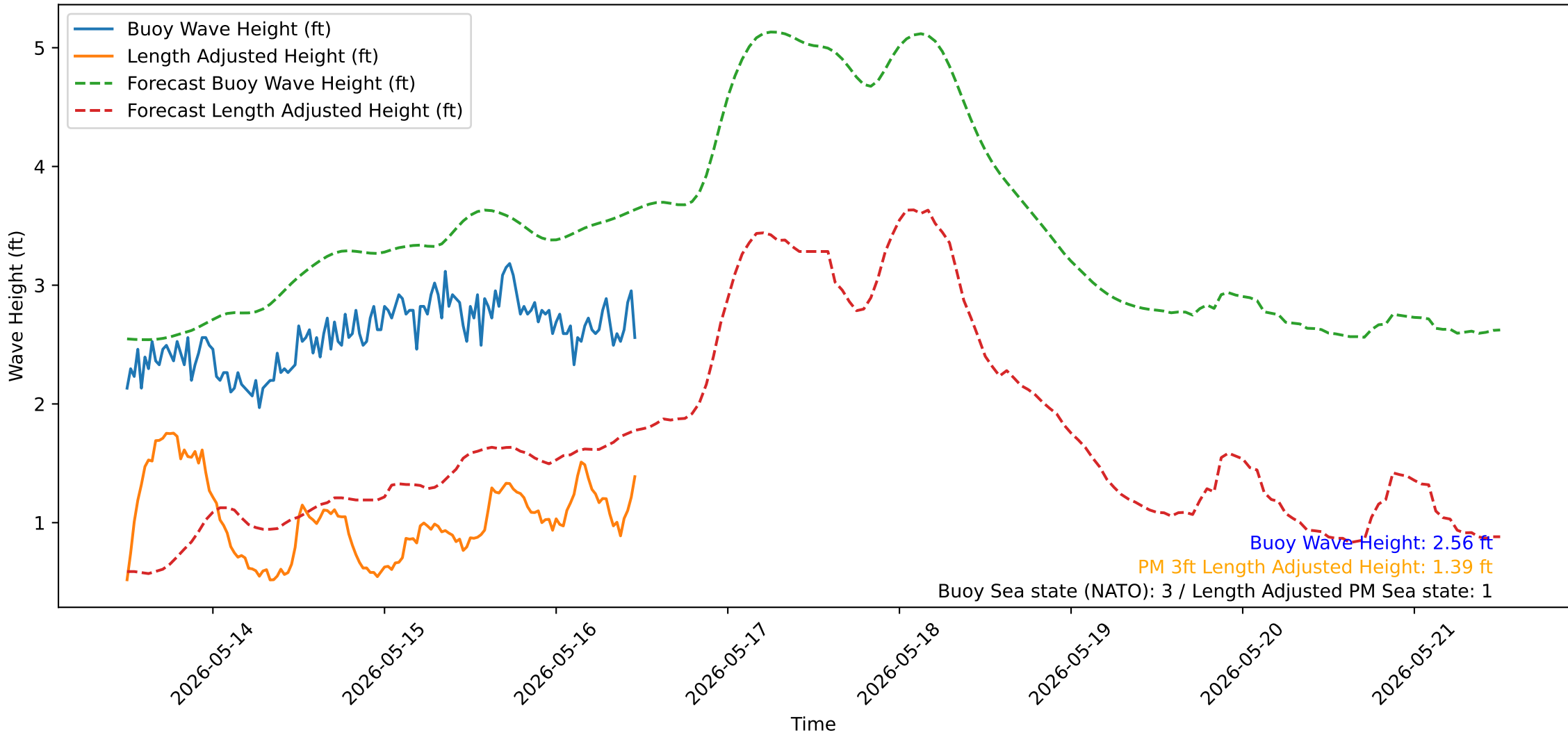
Wave Heights over Time for Red Beach at 2026-05-16 11:50:53
