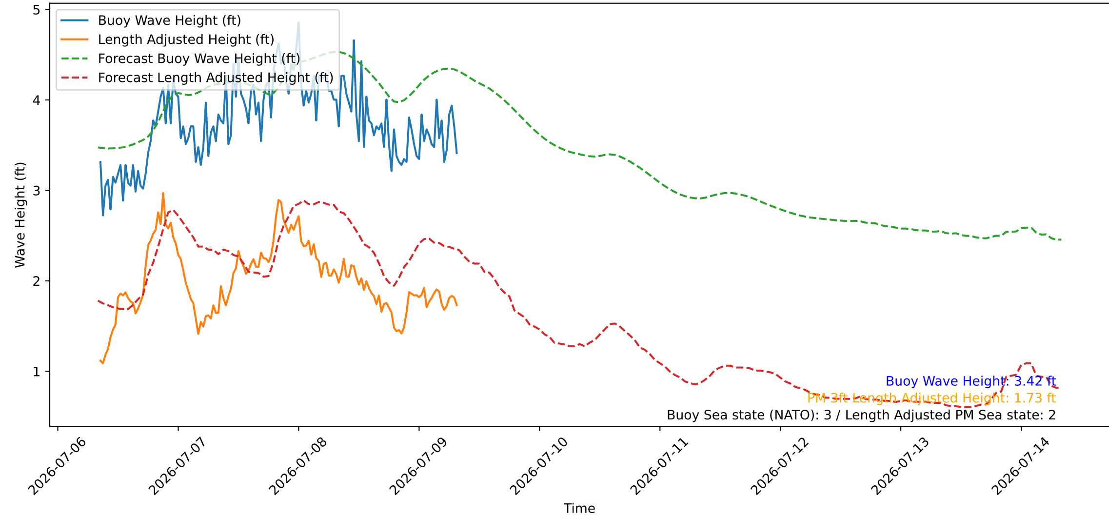
Wave Heights over Time for Red Beach at 2026-07-09 08:10:47
