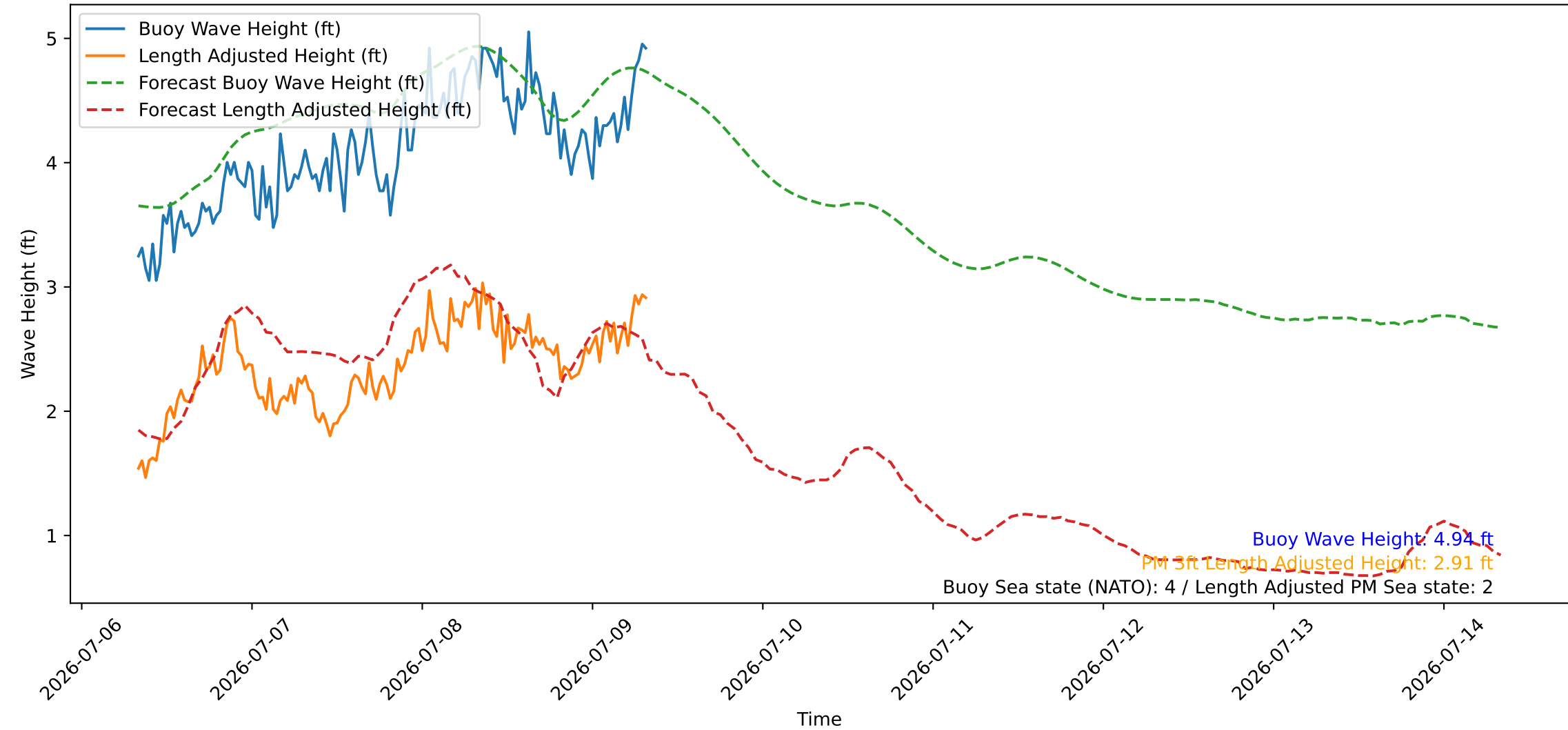
Wave Heights over Time for Oceanside Harbor at 2026-07-09 08:10:27
