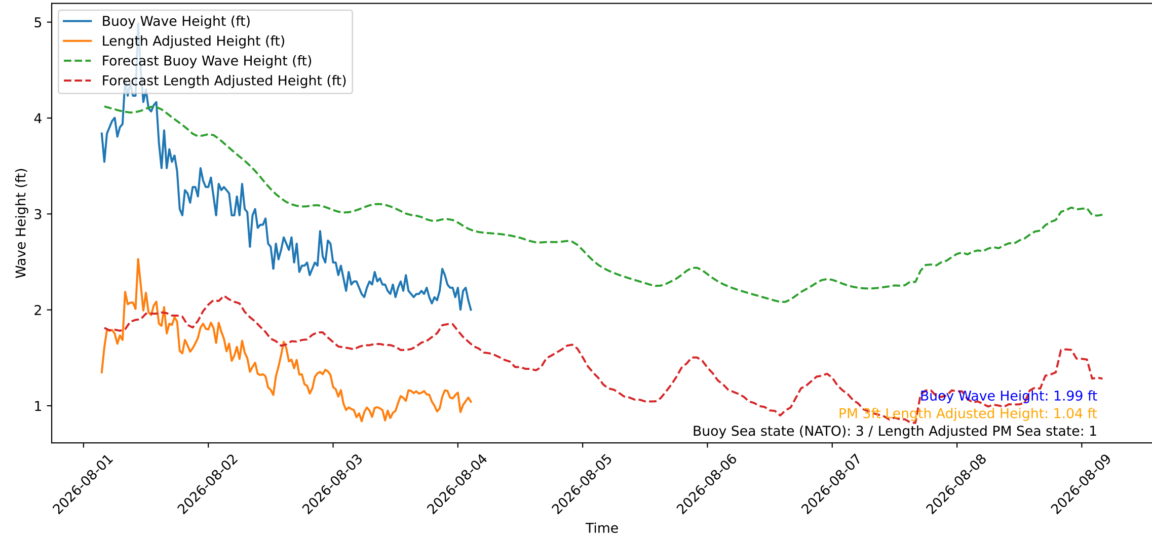
Wave Heights over Time for Green Beach at 2026-08-04 03:31:08
