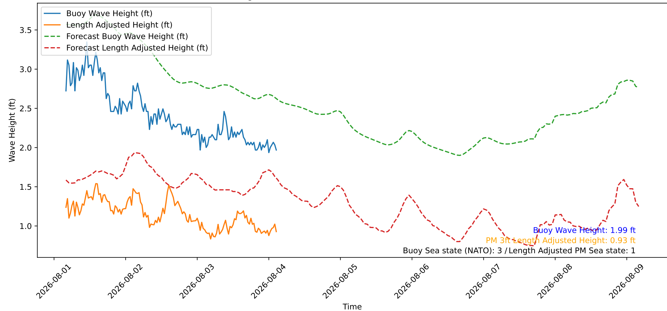
Wave Heights over Time for Red Beach at 2026-08-04 03:30:46
