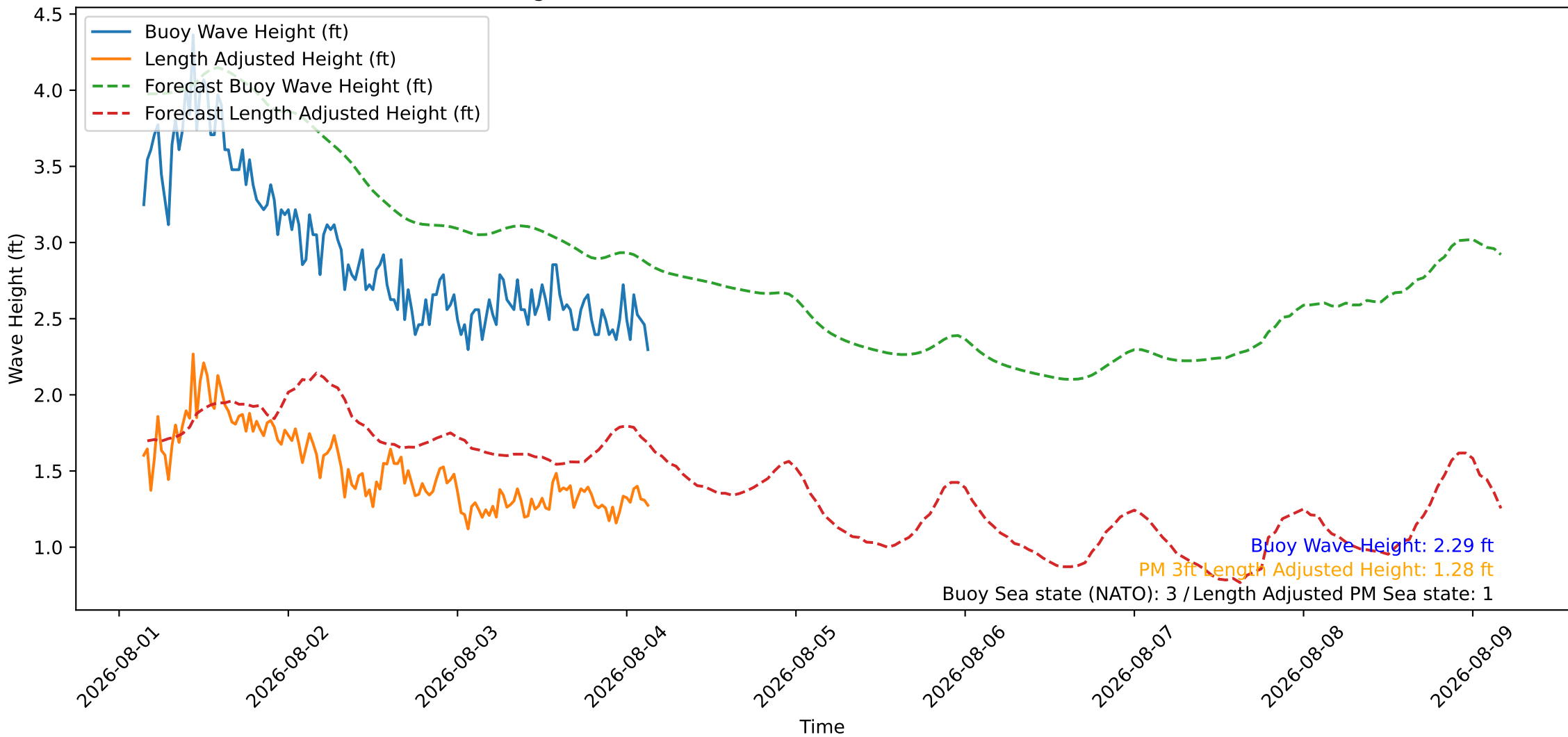
Wave Heights over Time for Oceanside Harbor at 2026-08-04 03:30:27
