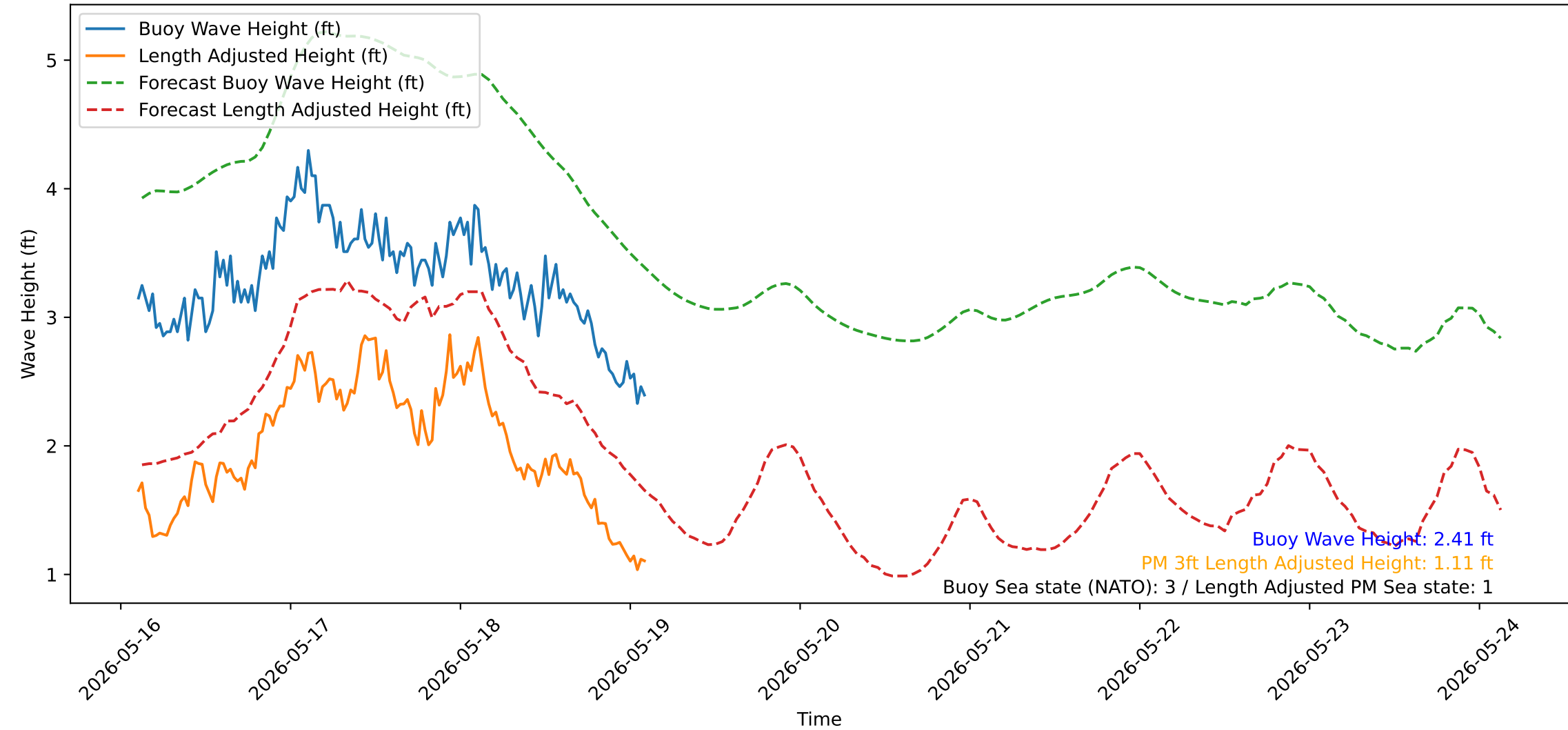
Wave Heights over Time for Oceanside Harbor at 2026-05-19 02:40:31
