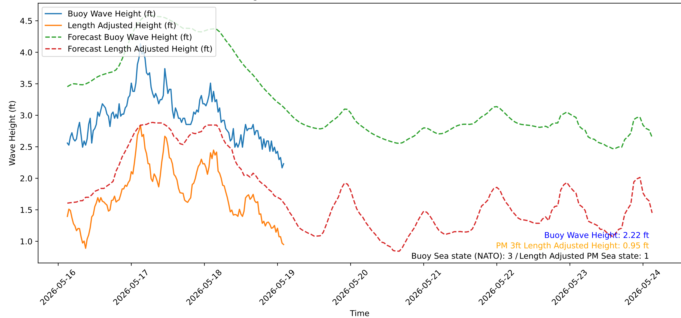
Wave Heights over Time for Red Beach at 2026-05-19 02:40:51
