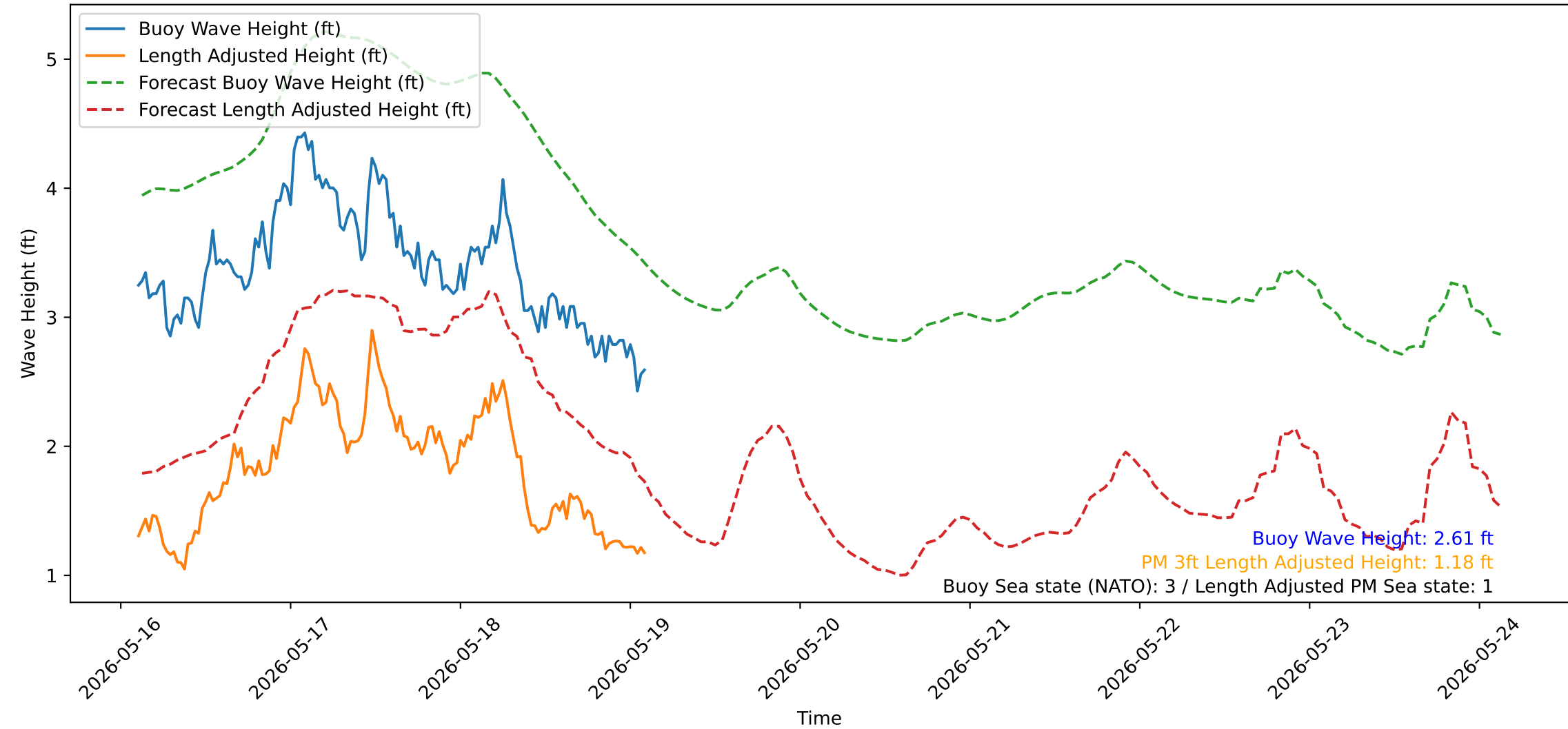
Wave Heights over Time for Green Beach at 2026-05-19 02:41:14
