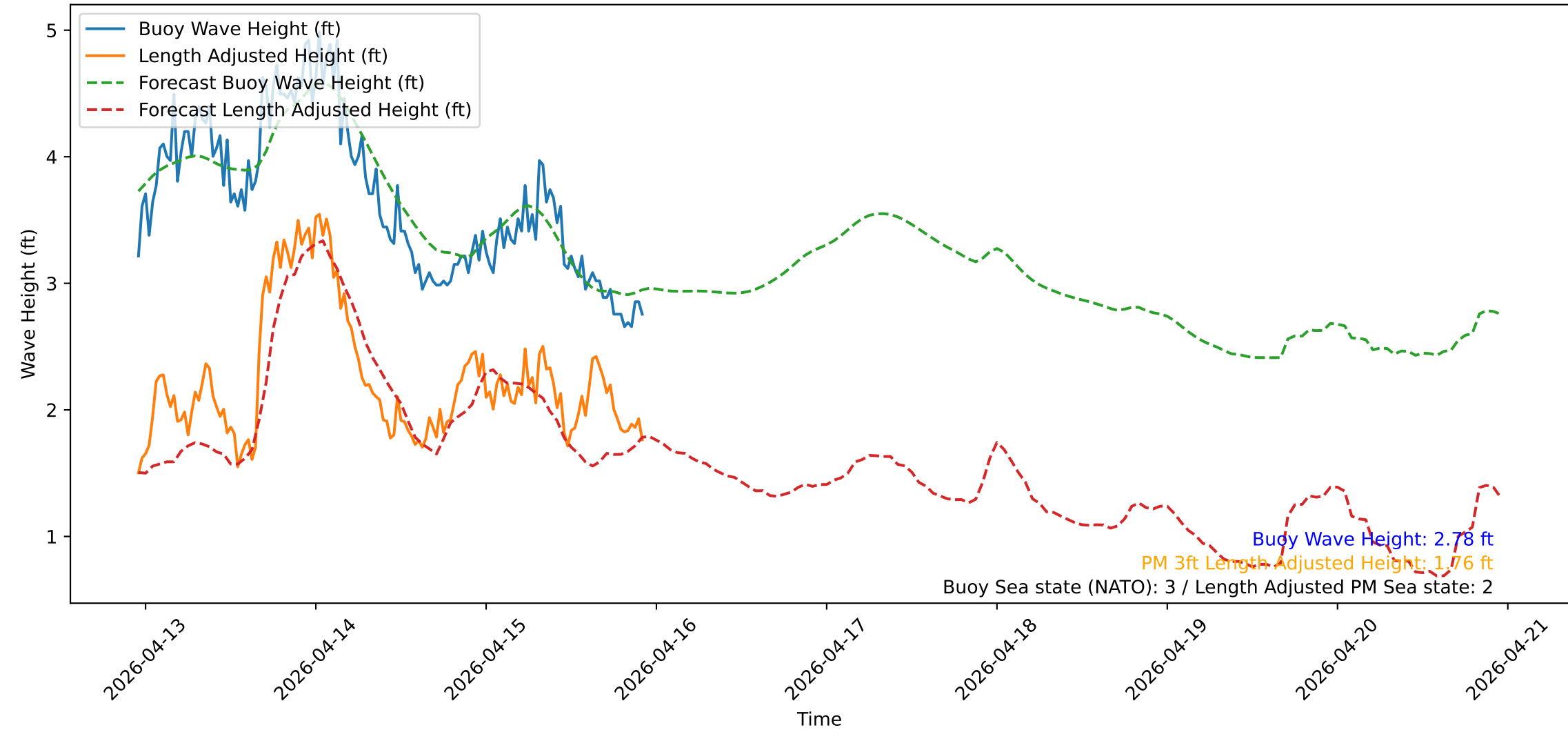
Wave Heights over Time for Green Beach at 2026-04-15 23:01:14
