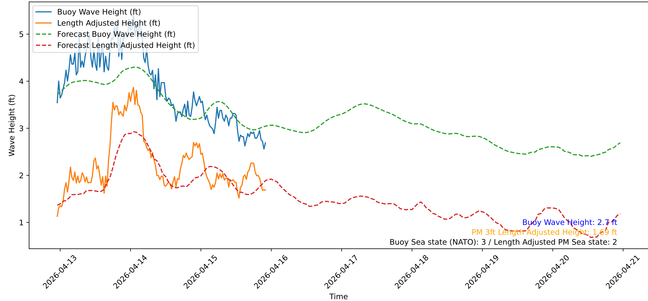
Wave Heights over Time for Oceanside Harbor at 2026-04-15 23:00:32
