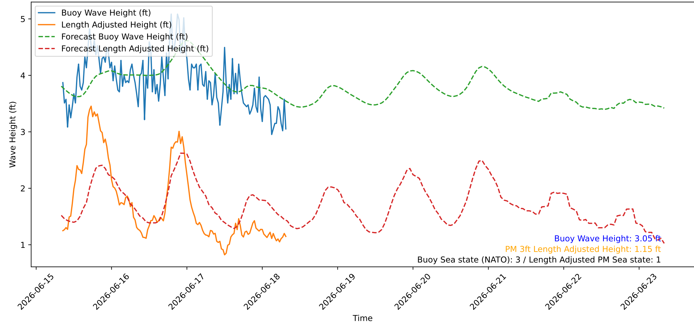
Wave Heights over Time for Green Beach at 2026-06-18 08:21:10
