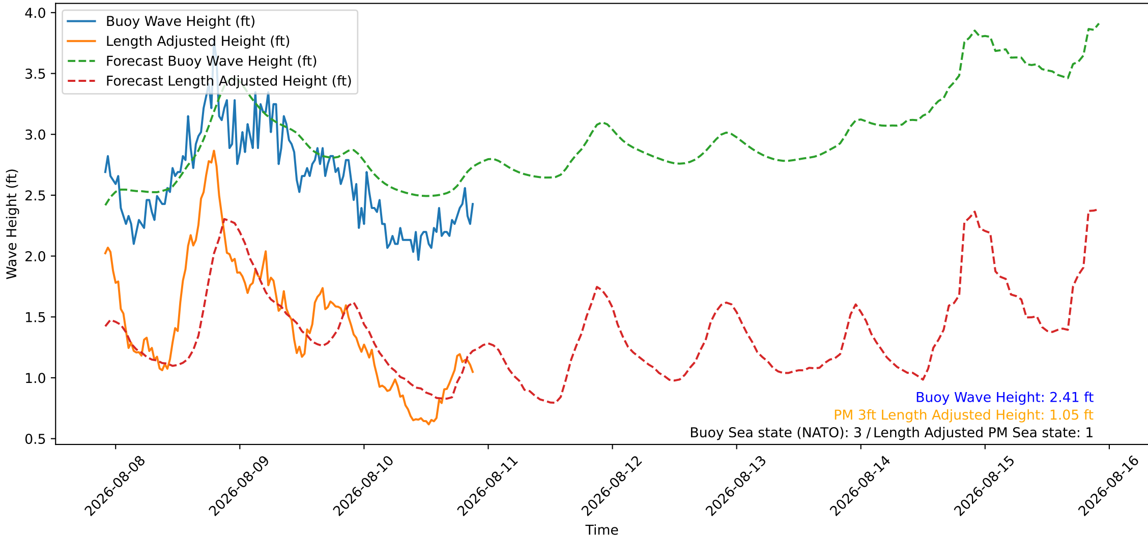
Wave Heights over Time for Green Beach at 2026-08-10 21:51:10
