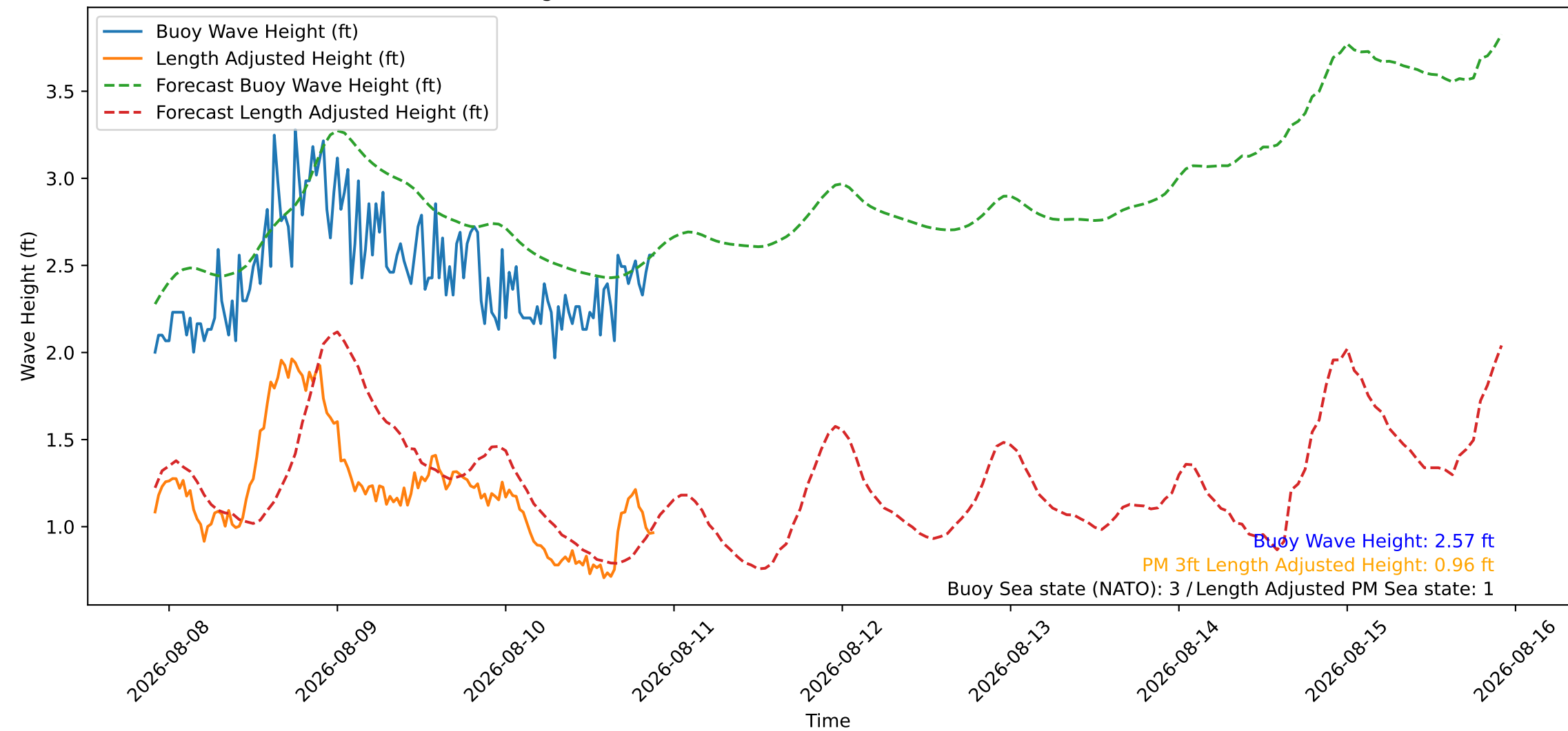
Wave Heights over Time for Oceanside Harbor at 2026-08-10 21:50:27
