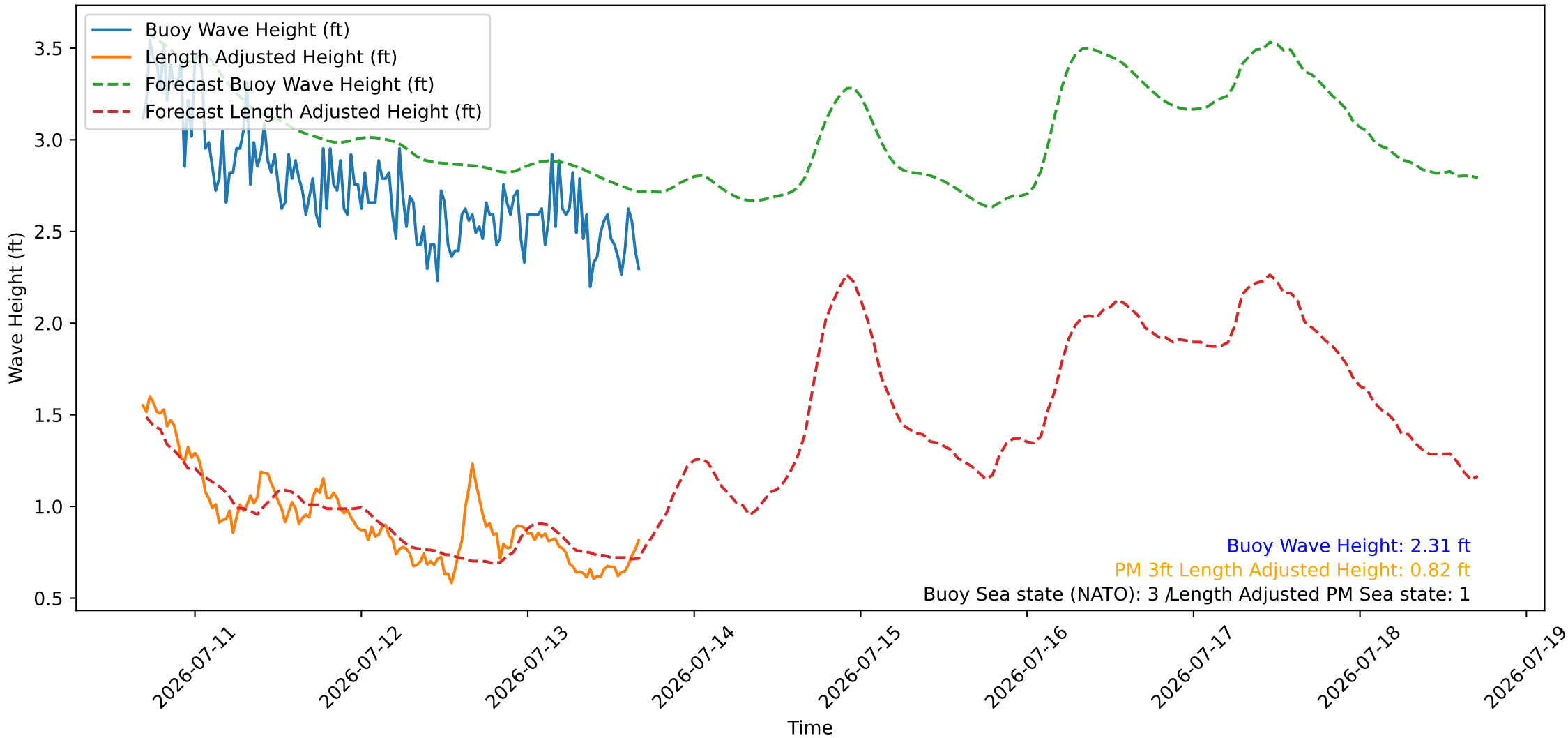
Wave Heights over Time for Green Beach at 2026-07-13 16:41:09
