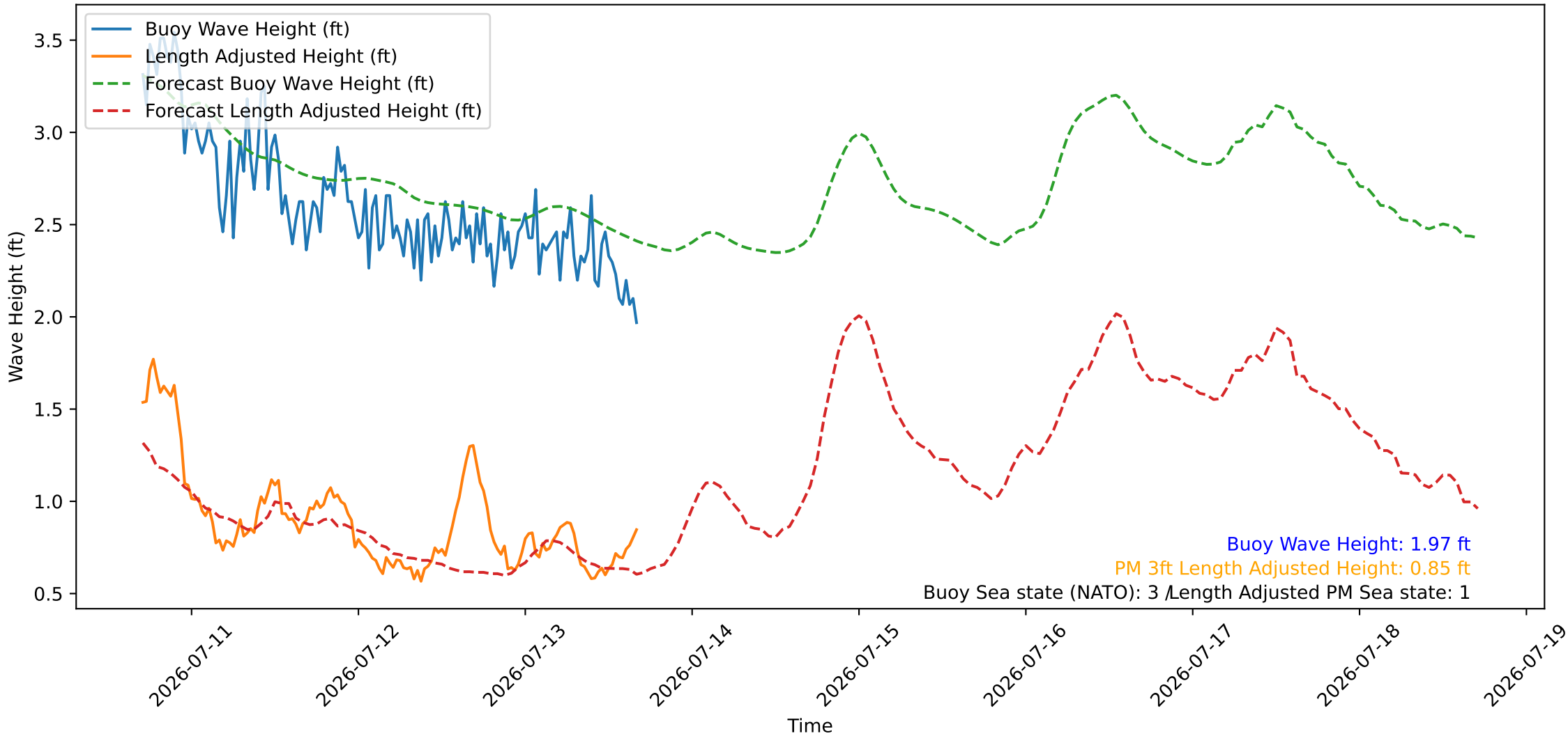
Wave Heights over Time for Red Beach at 2026-07-13 16:40:46
