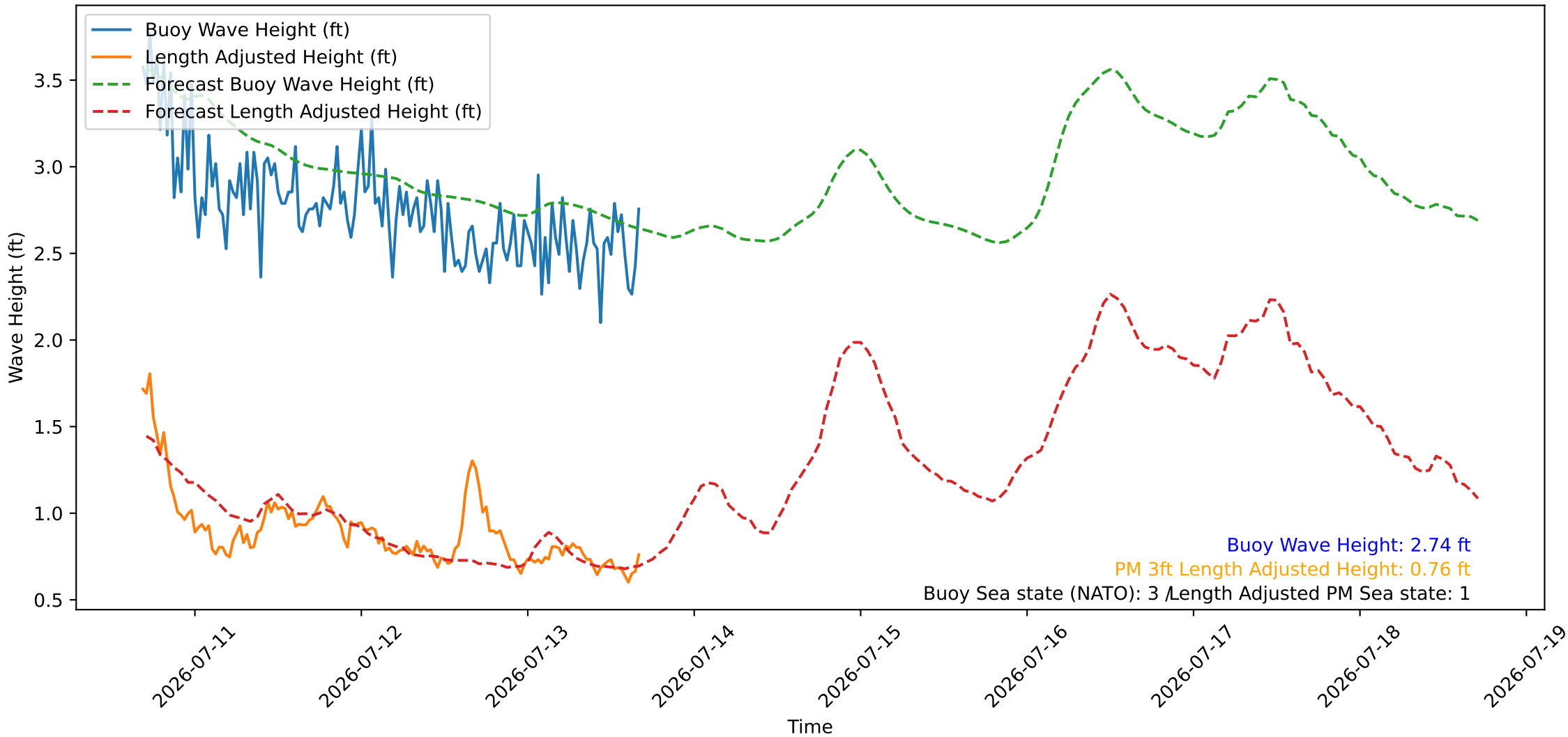
Wave Heights over Time for Oceanside Harbor at 2026-07-13 16:40:27
