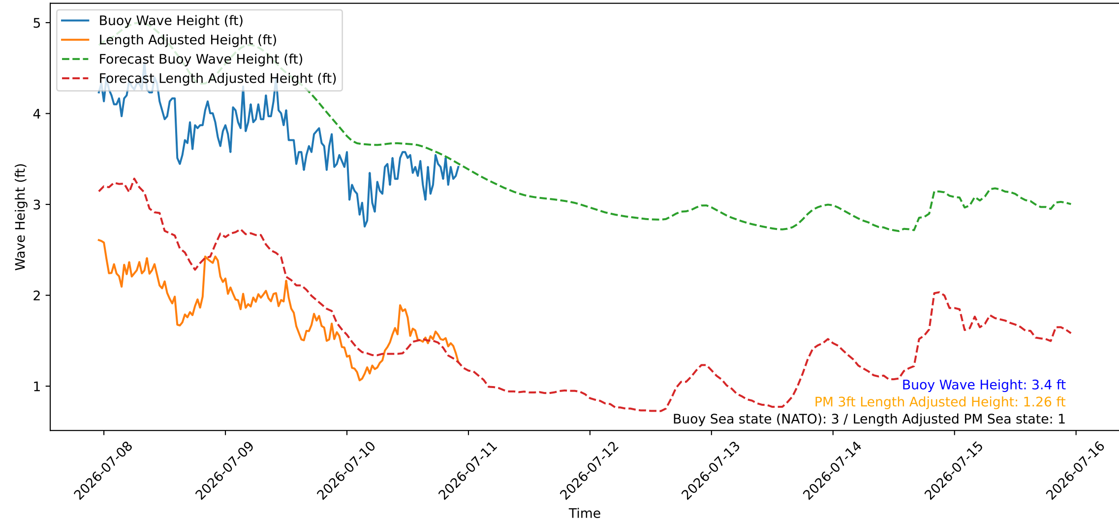
Wave Heights over Time for Green Beach at 2026-07-10 22:51:09
