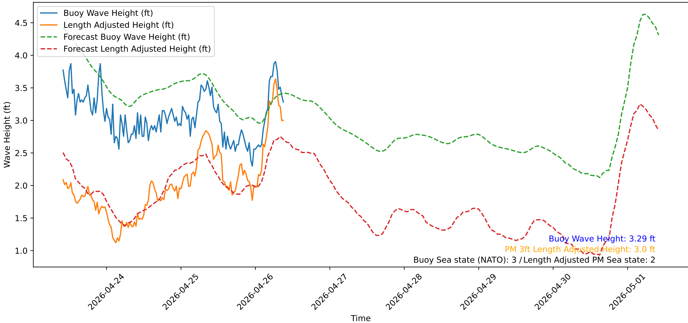
Wave Heights over Time for Oceanside Harbor at 2026-04-26 09:50:31
