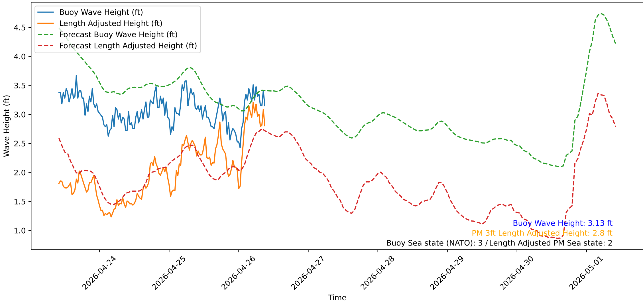
Wave Heights over Time for Green Beach at 2026-04-26 09:51:13
